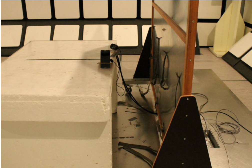
Photograph 3. Conducted emissions.
