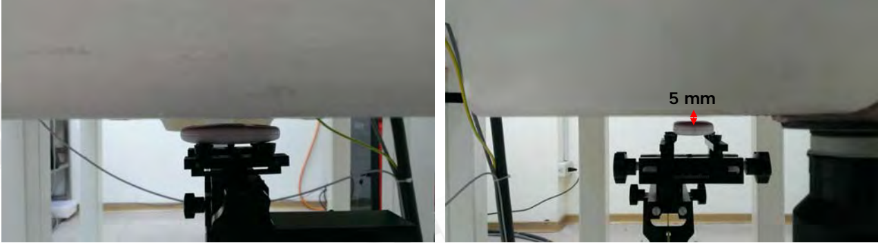
Fig.3 EUT front side to flat phantom
