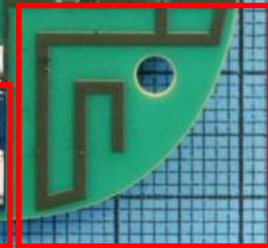
GNSS antenna
