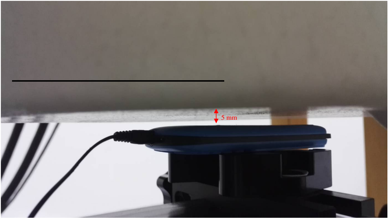
Body Back with headset Setup Photo (5mm)
