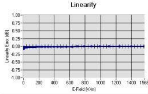
Linearity \pm 1.82% ( \pm 0.08dB)
