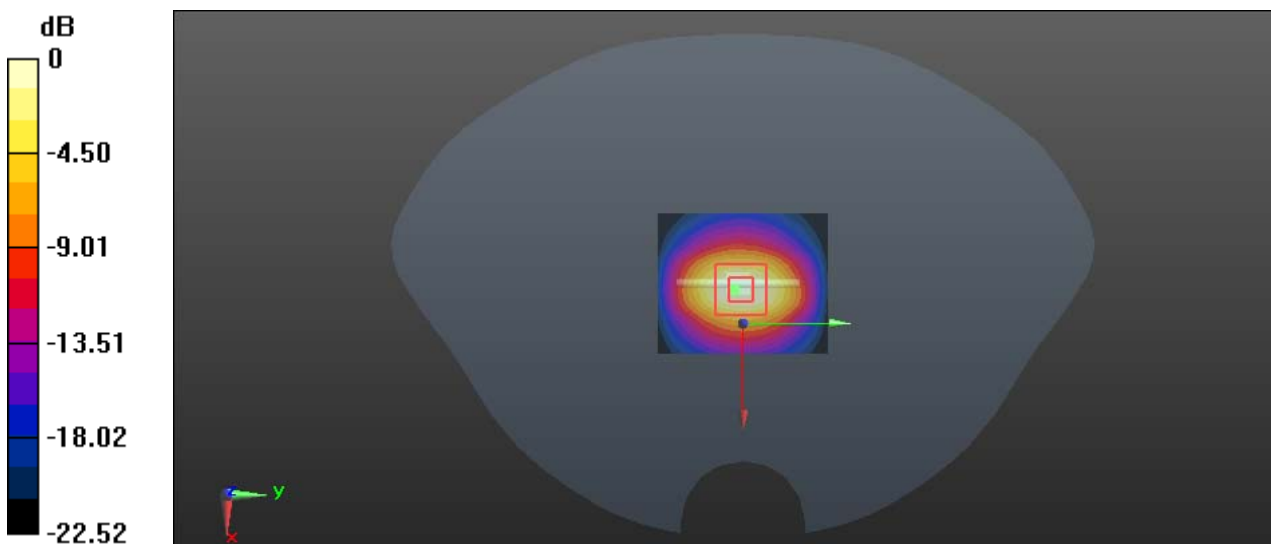
0 dB = 8.91 W/kg = 9.50 dBW/kg
