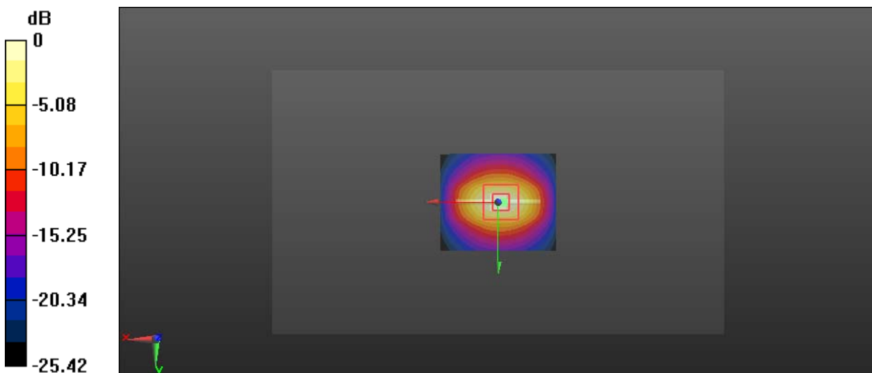
0 dB = 8.83 W/kg = 9.46 dBW/kg
