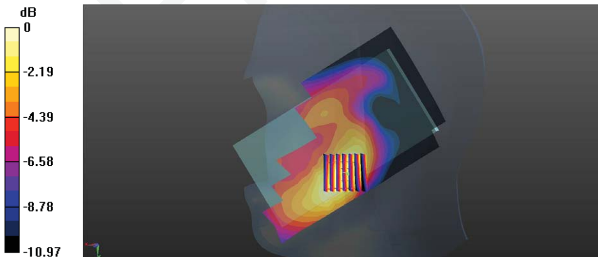
0 dB = 0.105 W/kg = -9.79 dBW/kg
