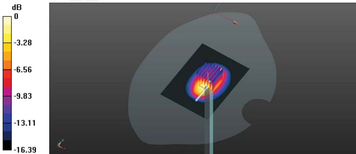
0 dB = 44.7 W/kg = 16.50 dBW/kg
