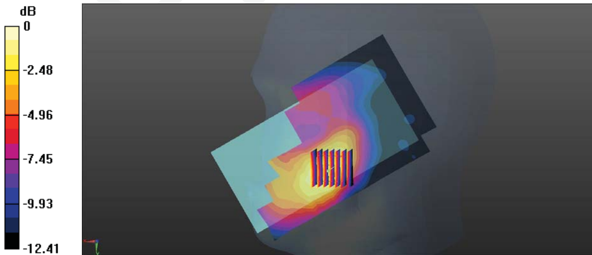
0 dB = 0.155 W/kg = -8.10 dBW/kg
