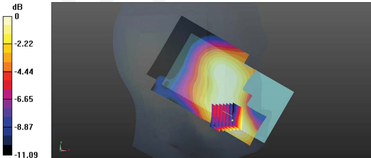
0 dB = 0.0458 W/kg = -13.39 dBW/kg
