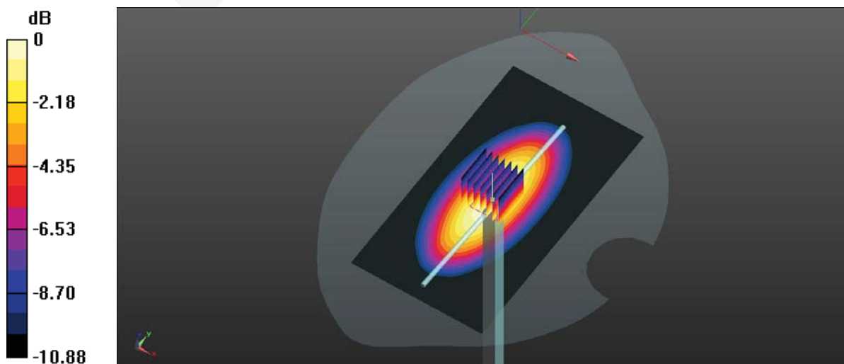
0 dB = 10.7 W/kg = 10.29 dBW/kg
