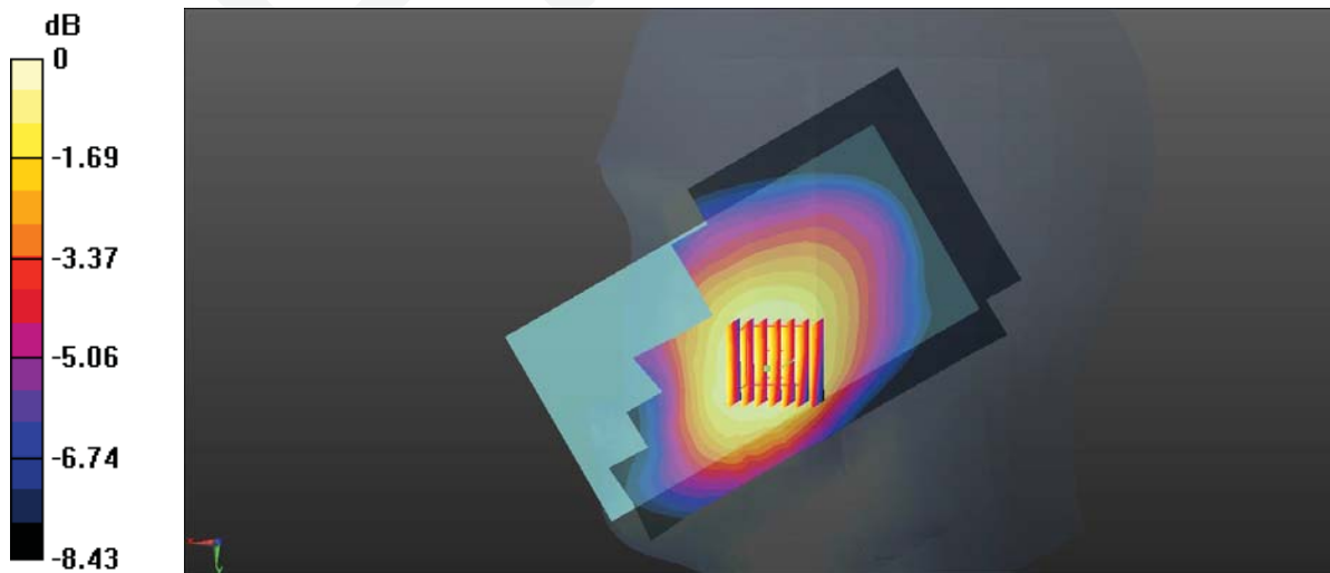
0 dB = 0.318 W/kg = -4.98 dBW/kg
