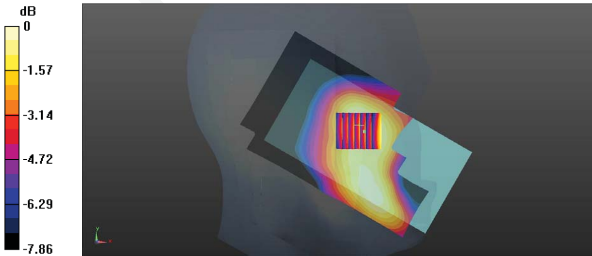
0 dB = 0.0622 W/kg = -12.06 dBW/kg
