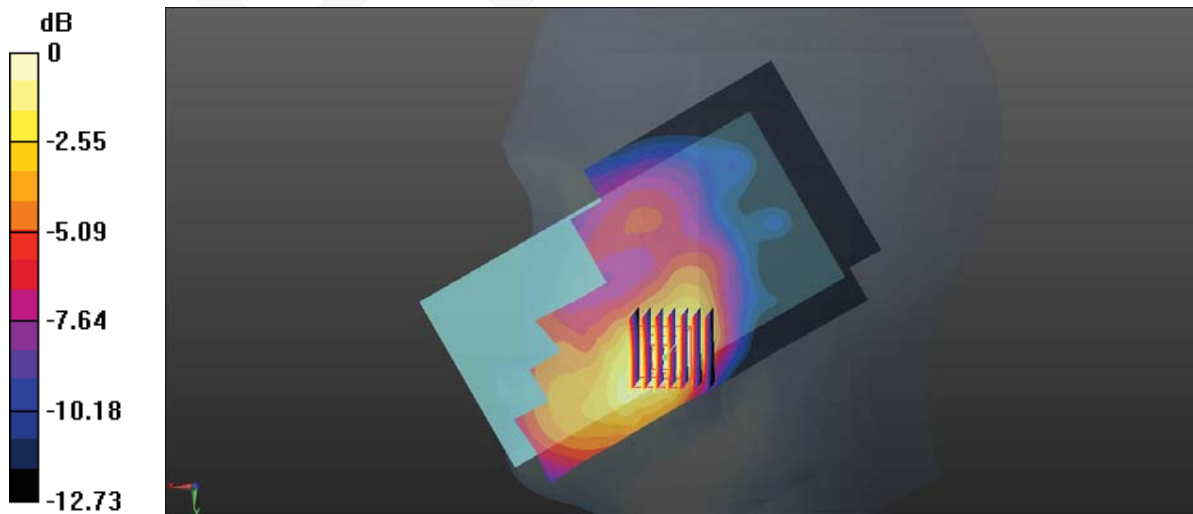
0 dB = 0.261 W/kg = -5.83 dBW/kg
