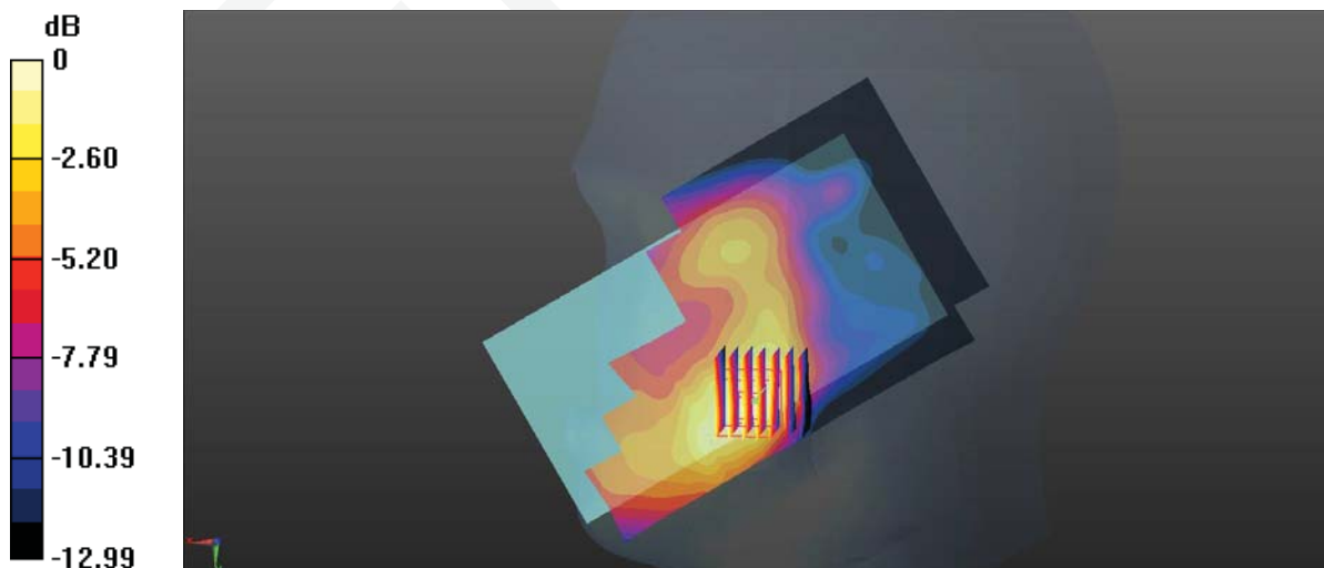
0 dB = 0.181 W/kg = -7.42 dBW/kg
