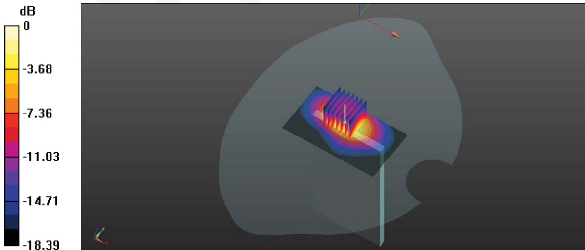
0 dB = 1.59 W/kg = 2.01 dBW/kg
