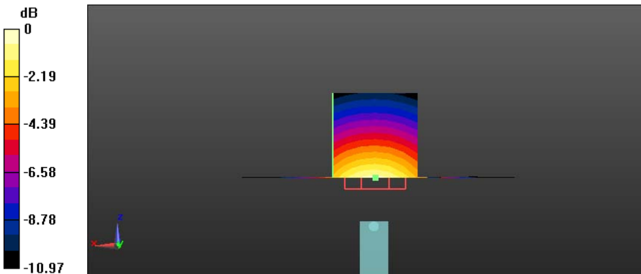
0 dB = 10.9 W/kg = 10.37 dBW/kg
