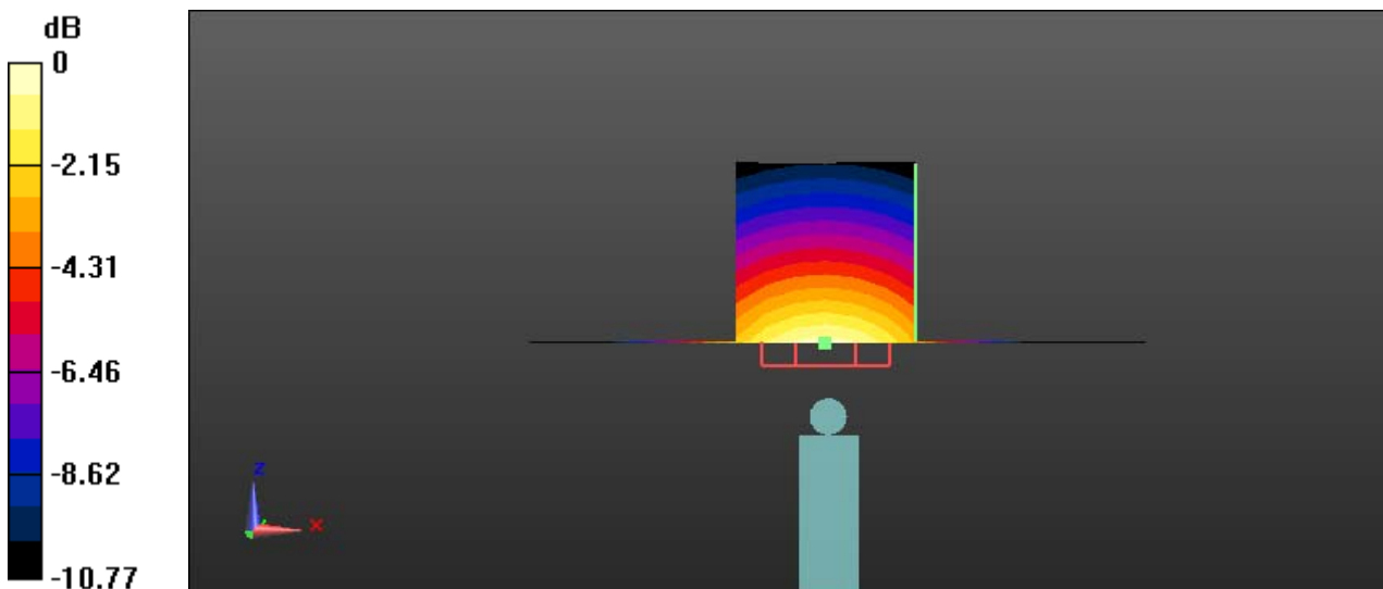
0 dB = 9.39 W/kg = 9.73 dBW/kg
