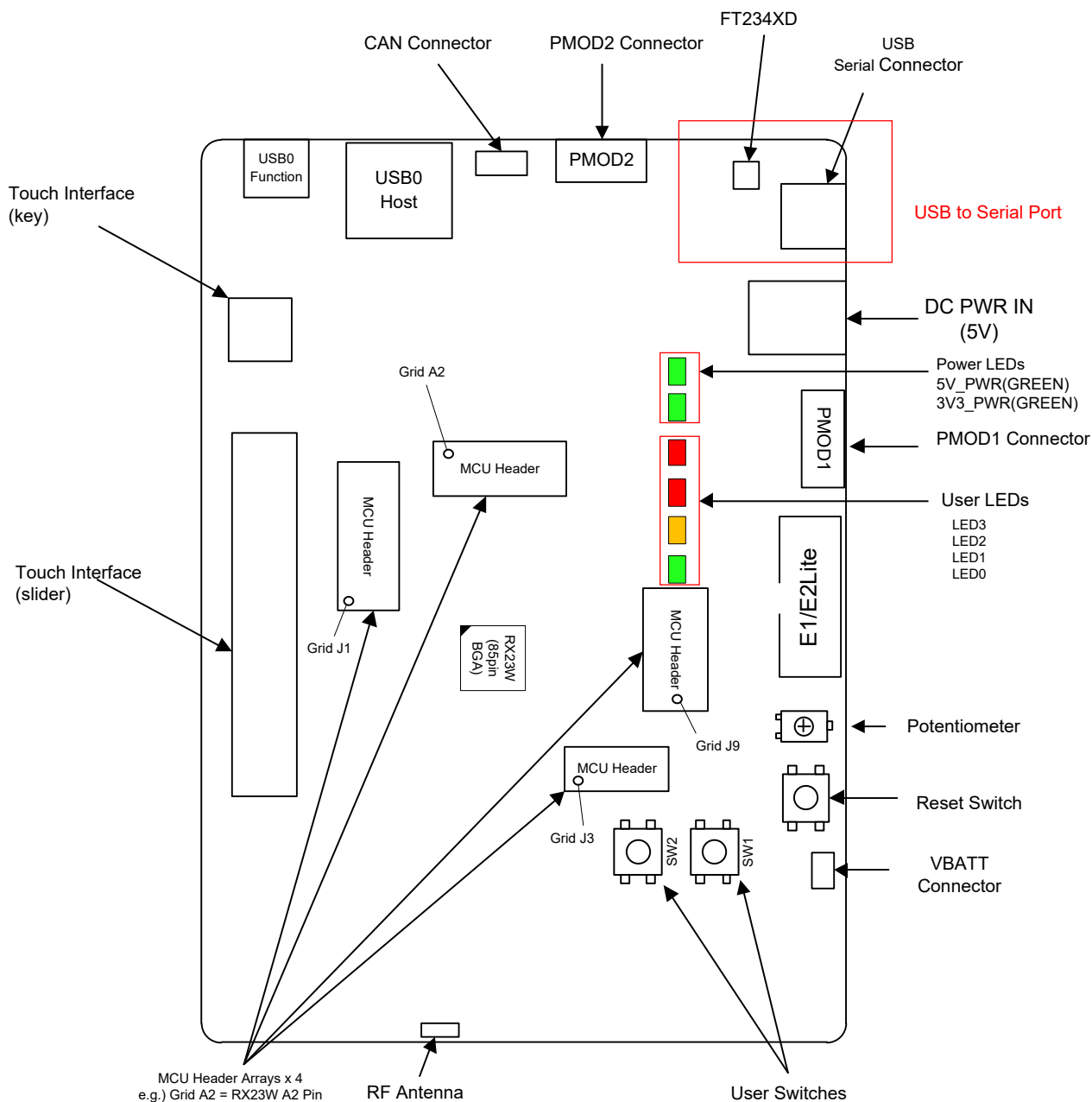
Figure 3-1: Board Layout
