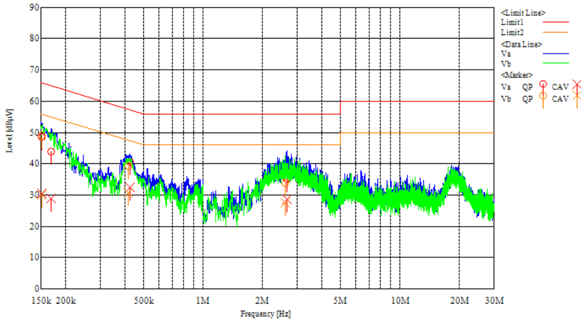
[Chart (2480MHz)]
