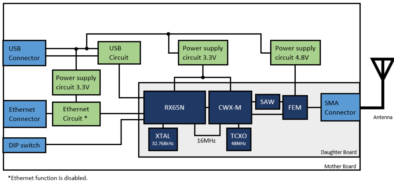
Figure 1-1: Block Diagram
