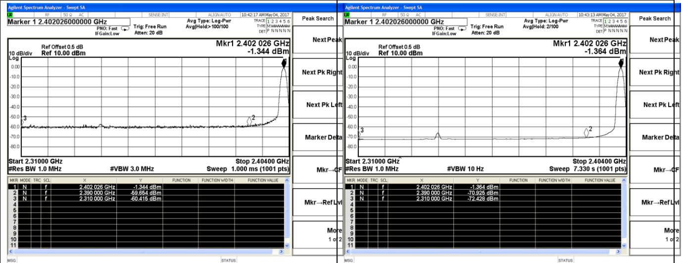
Channel 00 / 2402 MHz – Peak
