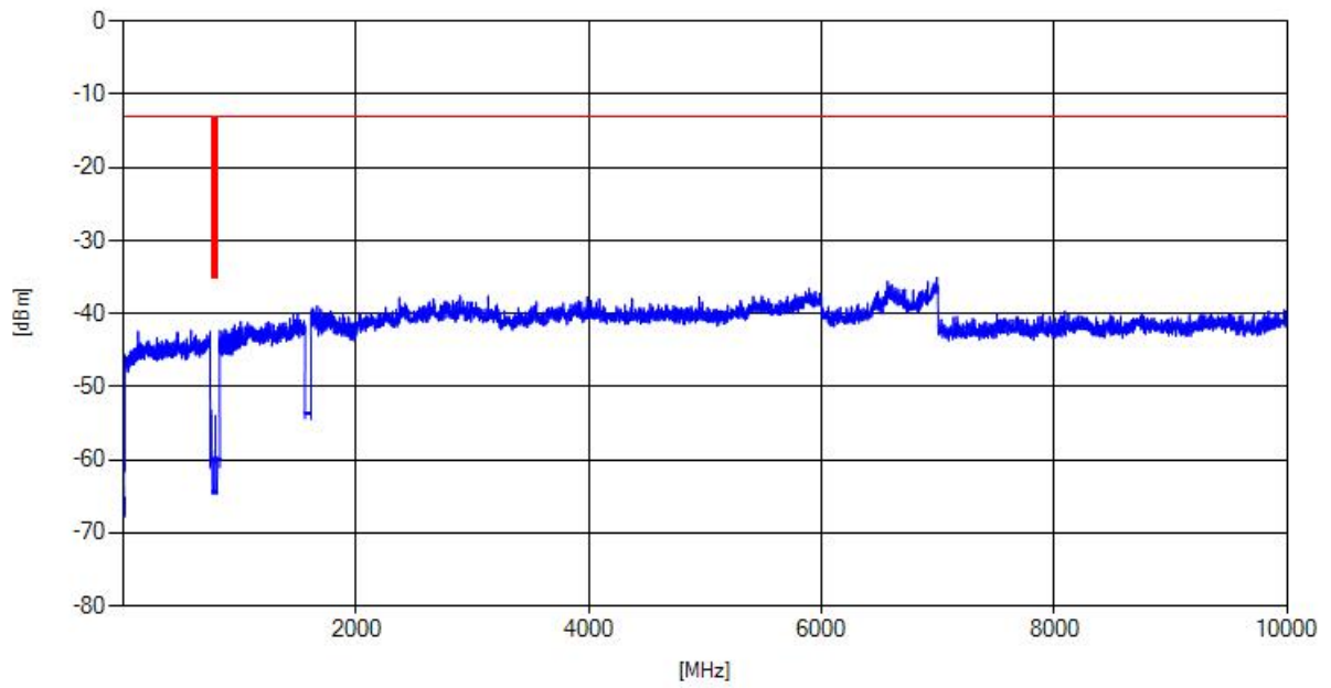
NB-IoT eFDD13 QPSK, Channel = mid
