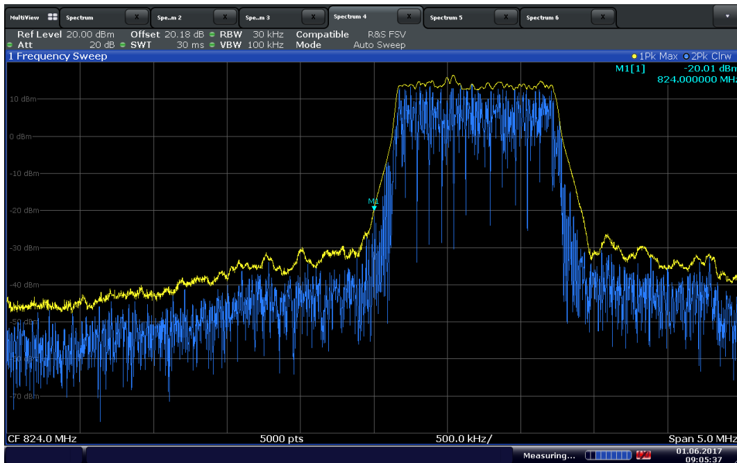
LTE Band 5 Band Edge @ 824MHz (QPSK)
