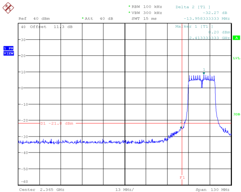
Plot 38. 802.11g No HT, 2412MHz Lower Band Edge, Chain 1
