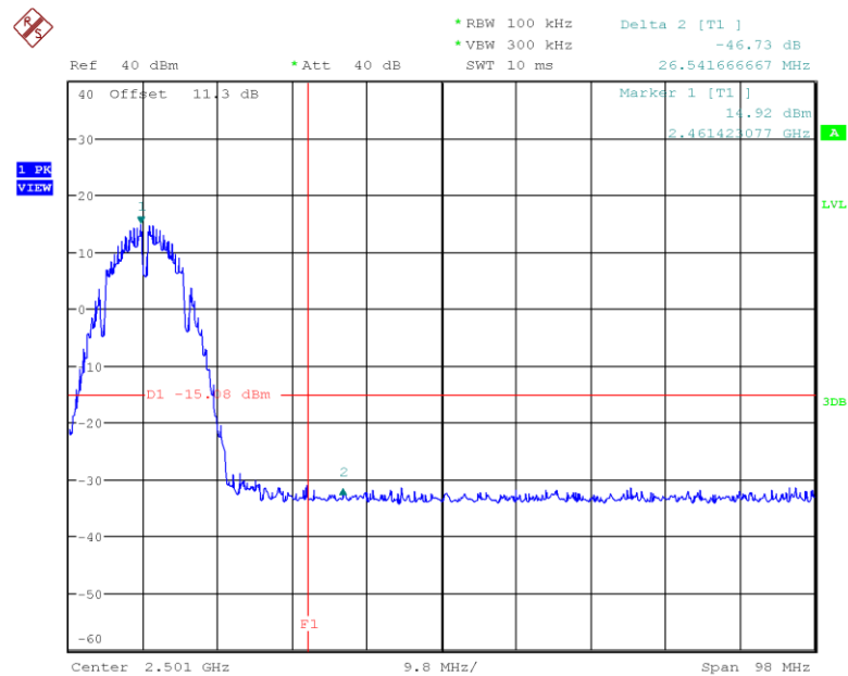
Plot 44. 802.11b CCK, 2462MHz Upper Band Edge, Chain 1
