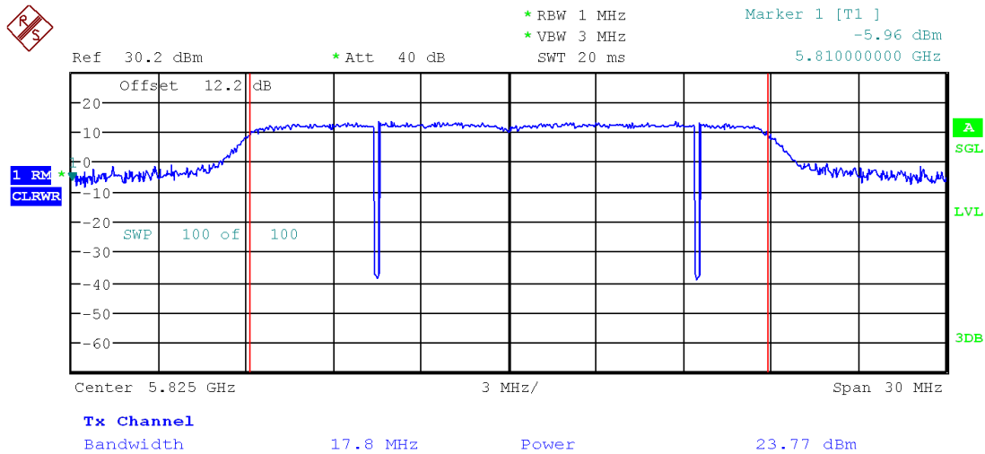
Figure 3: Output Power, Channel 165 802.11 HT20, Chain 0
