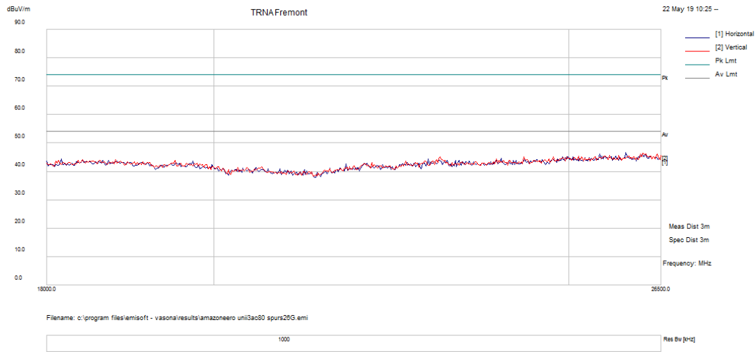
Figure 153: 18-26.5 GHz 802.11ac80 Mode Channel 155
