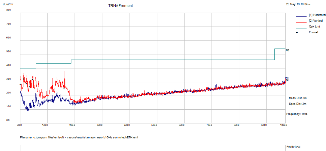
Figure 129: 30MHz-1GHz 802.11a Mode Channel 44
