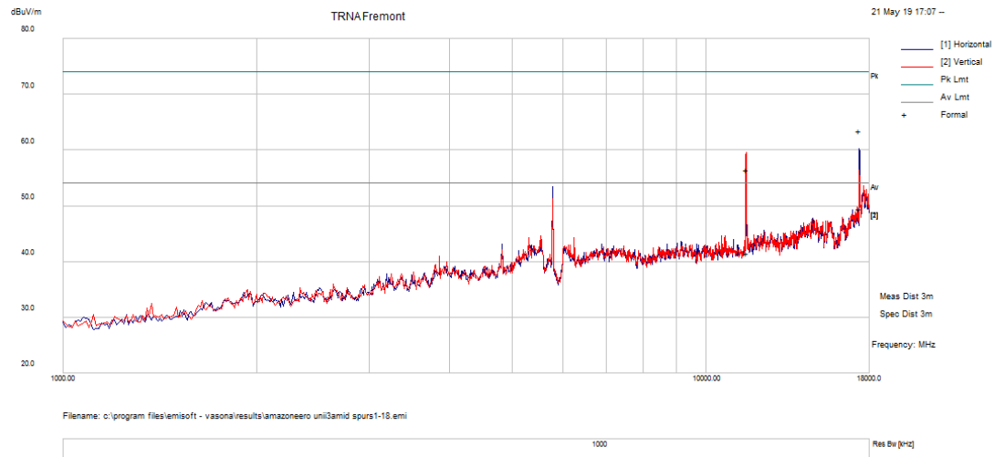
Figure 146: 1-18GHz 802.11a Mode Channel 157
