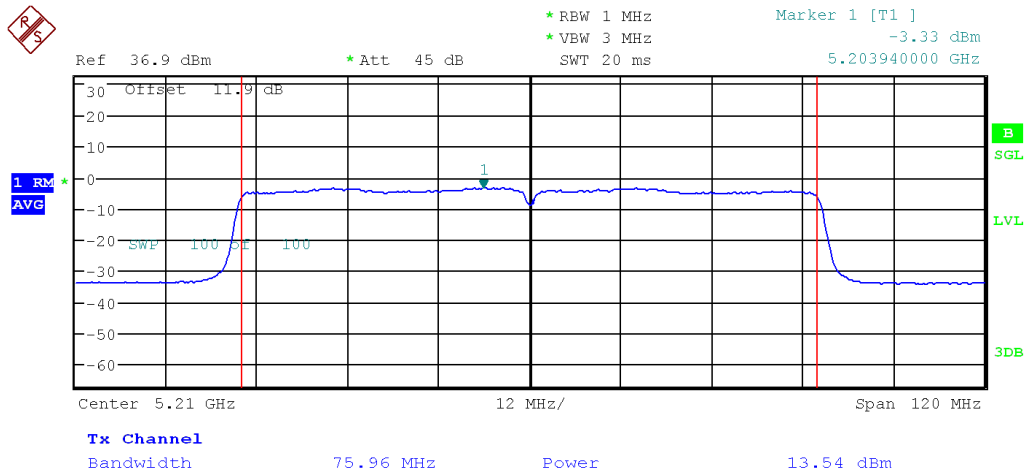
Figure 5: Output Power, Channel 42 802.11 ac80, Chain 0
