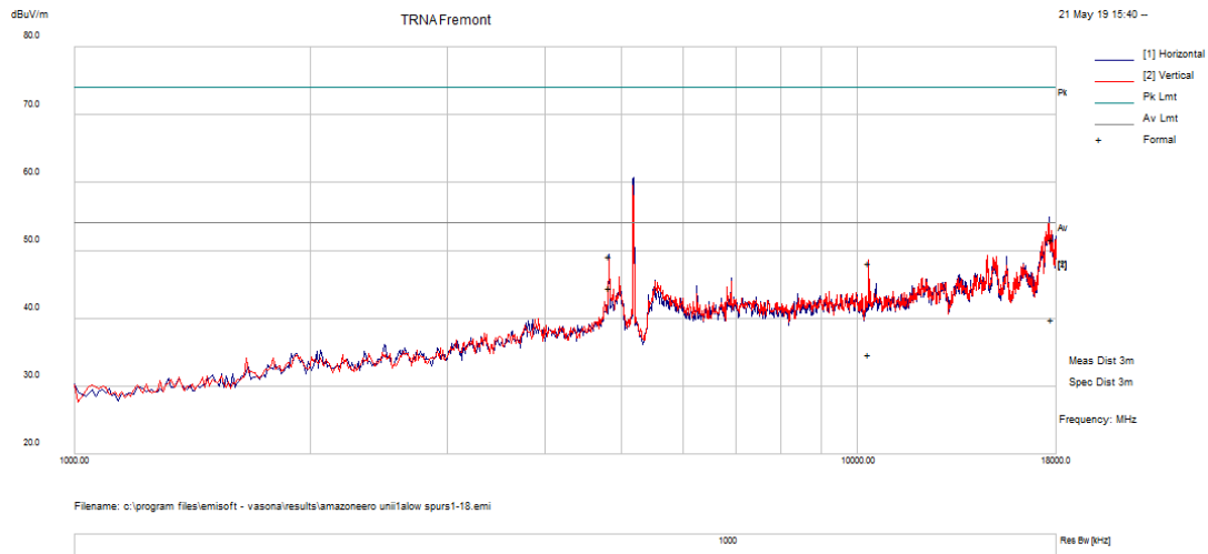
Figure 130: 1-18GHz 802.11a Mode Channel 36
