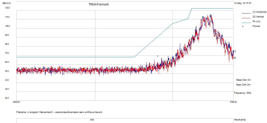
Figure 121: Low U-NII-3 band edge for 802.11a NoHT 6Mbps at Channel 149
