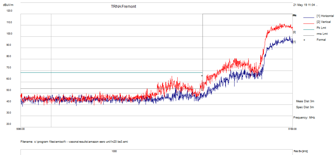
Figure 118: UNII-1 Low Band Edge for 802.11n HT20 6.5Mbps at 5180 MHz-peak
