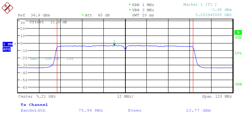
Figure 6: Output Power, Channel 42 802.11 ac80, Chain 1
