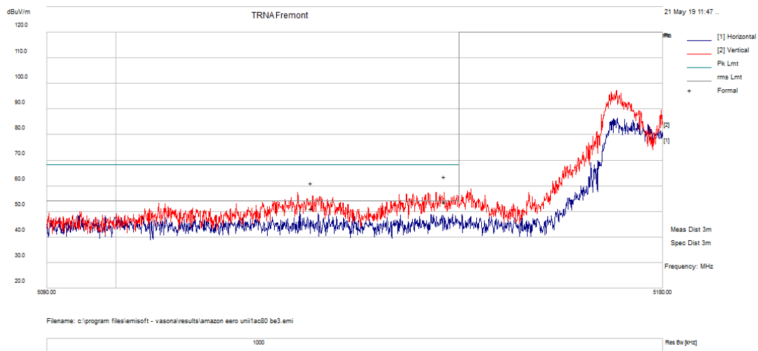
Figure 120: UNII-1 Low Band Edge for 802.11ac VHT80 MCS0 at 5210 MHz-Peak
