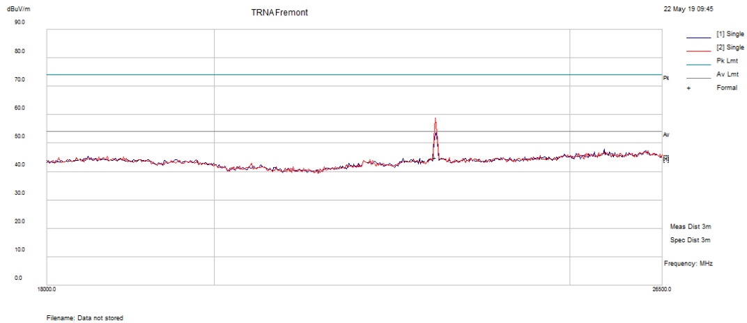
Figure 144: 18-26.5 GHz 802.11a Mode Channel 149
