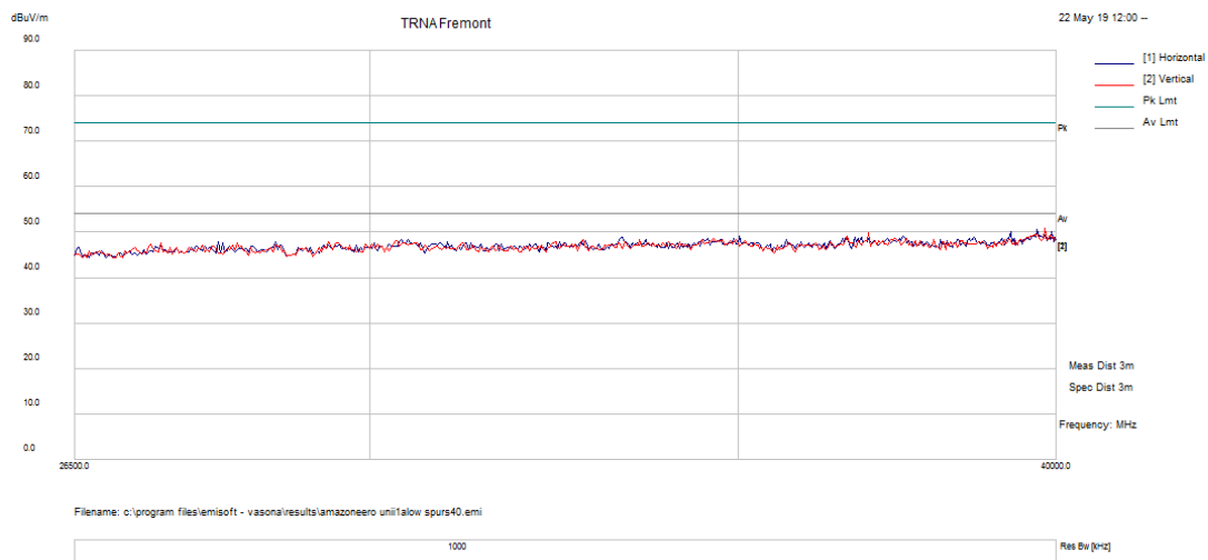
Figure 132: 26.5-40 GHz 802.11a Mode Channel 36
