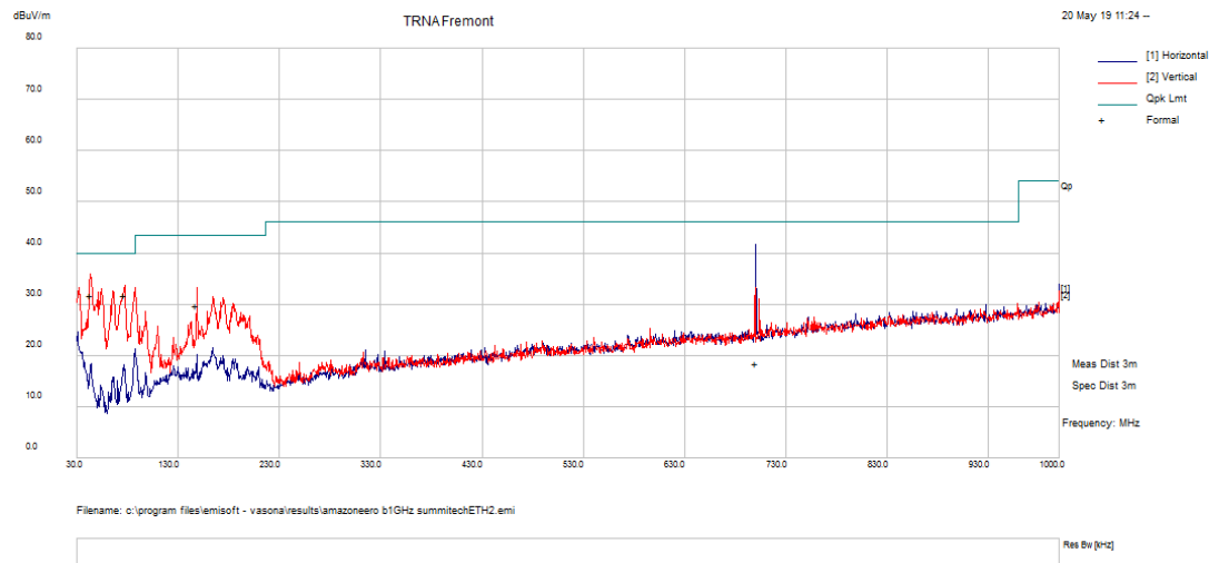
Figure 142: 30MHz-1GHz 802.11a Mode Channel 149
