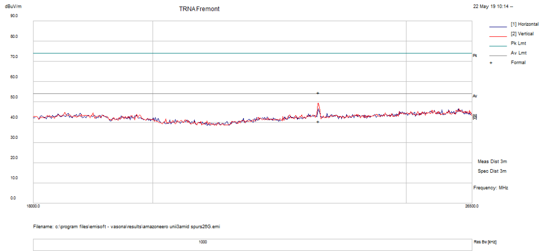
Figure 147: 18-26.5 GHz 802.11a Mode Channel 157
