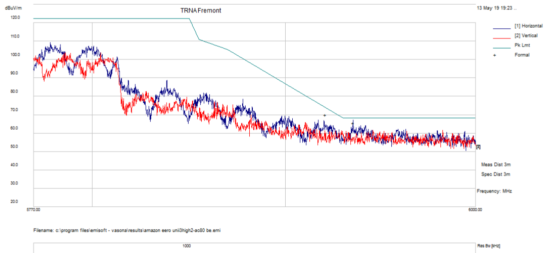
Figure 128: High U-NII-3 band edge for 802.11ac VHT80 MCS0 at Channel 155
