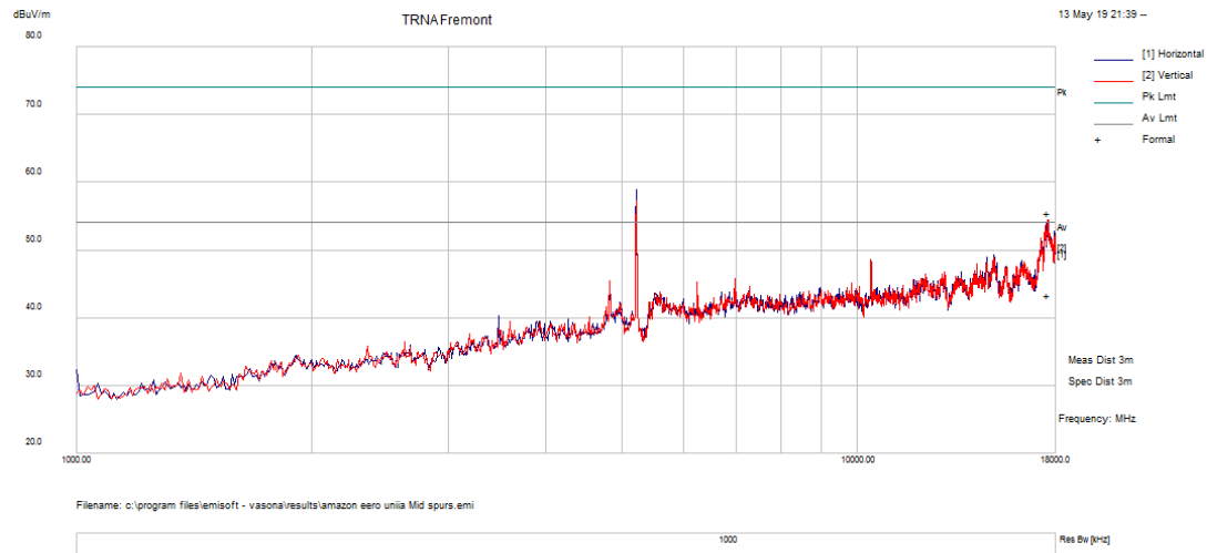
Figure 133: 1-18GHz 802.11a Mode Channel 44
