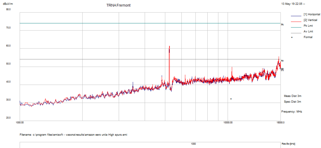
Figure 136: 1-18GHz 802.11a Mode Channel 48
