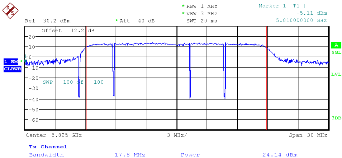
Figure 4: Output Power, Channel 165 802.11 HT20, Chain 1
