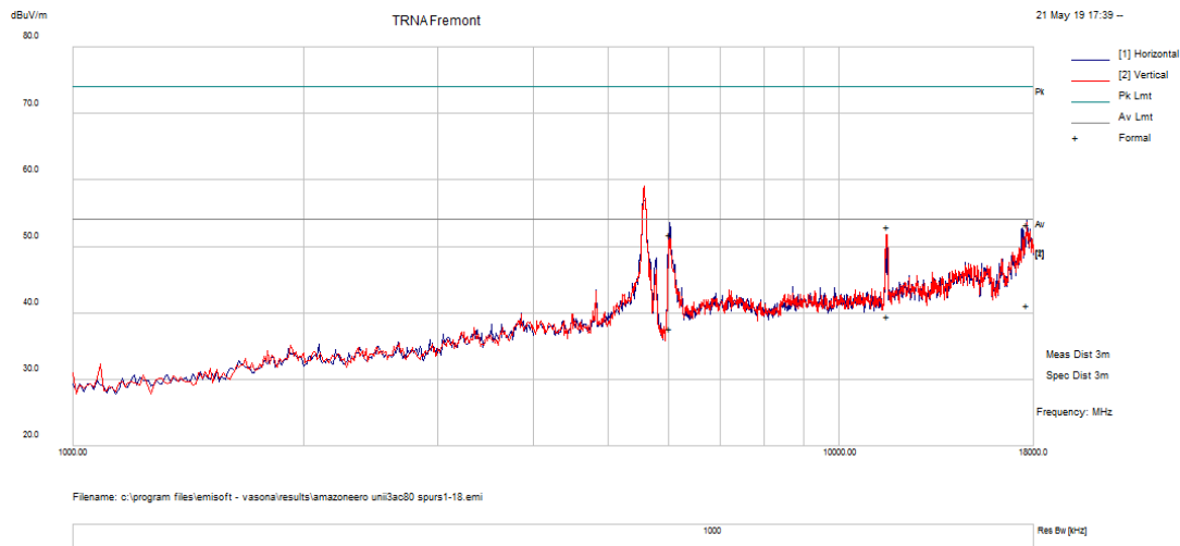
Figure 152: 1-18GHz 802.11ac80 Mode Channel 155
