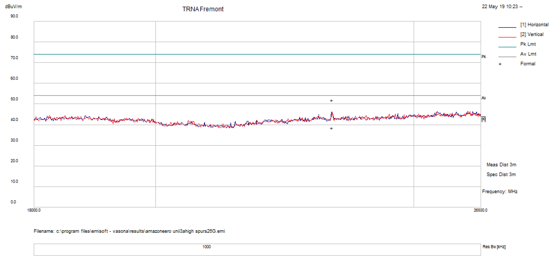
Figure 150: 18-26.5 GHz 802.11a Mode Channel 165
