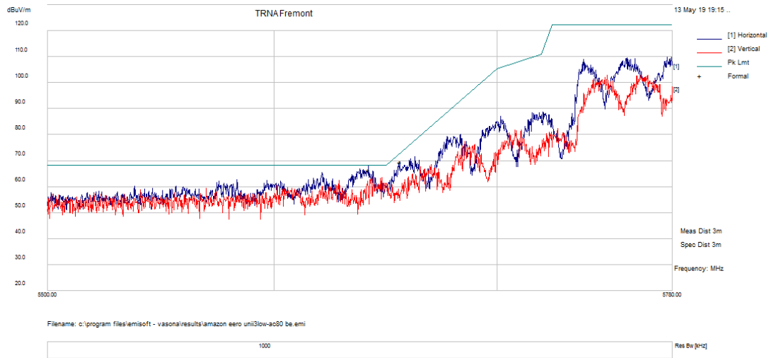
Figure 127: Low U-NII-3 band edge for 802.11ac VHT80 MCS0 at Channel 155
