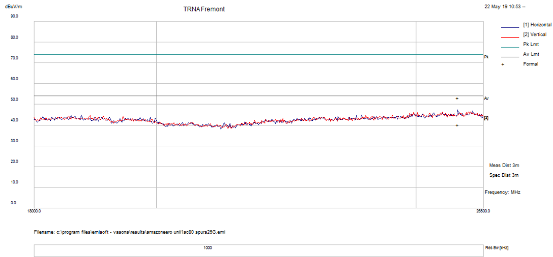
Figure 140: 18-26.5 GHz 802.11ac80 Mode Channel 42
