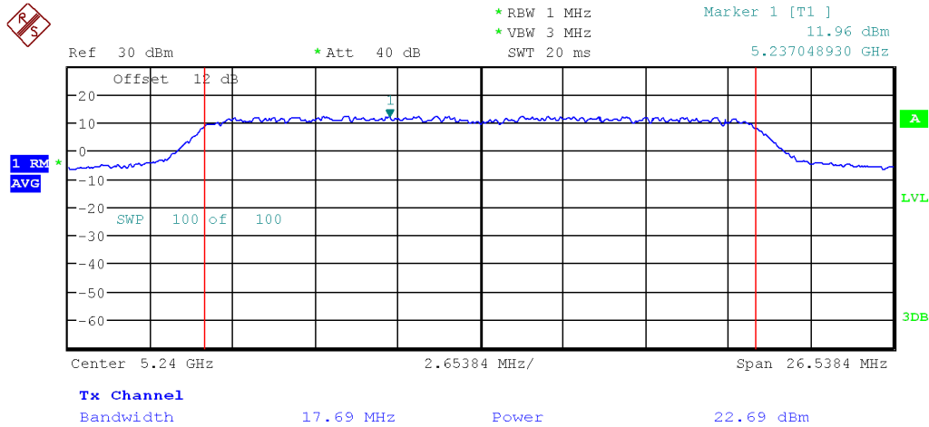
Figure 1: Output Power, Channel 48 802.11 HT20, Chain 0
