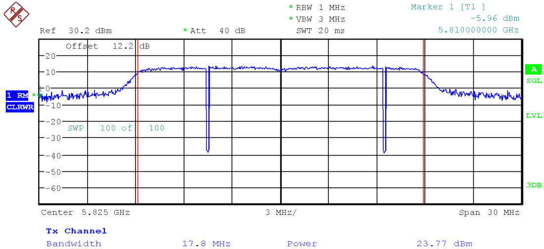
Figure 7: Output Power, Channel 165 802.11 HT20, Chain 0
