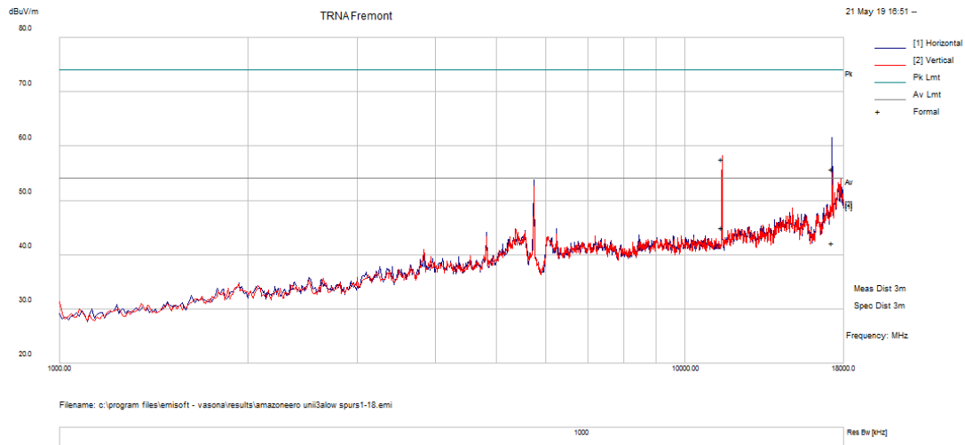
Figure 143: 1-18GHz 802.11a Mode Channel 149
