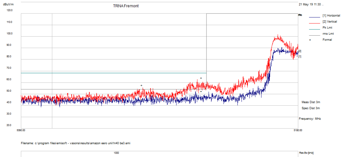
Figure 119: UNII-1 Low Band Edge for 802.11n HT40 MCS0 at 5190 MHz-Peak
