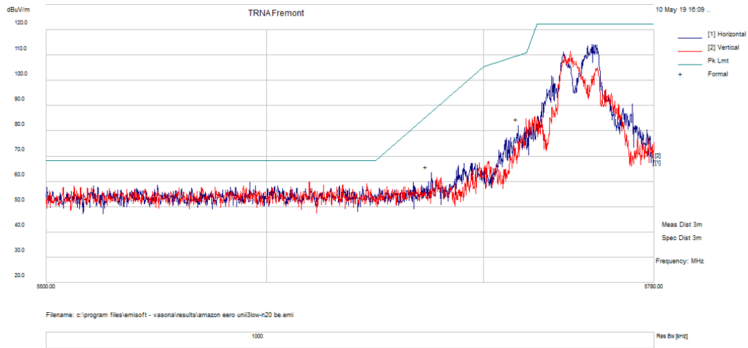
Figure 123: Low U-NII-3 band edge for 802.11n HT20 6.5Mbps at Channel 149
