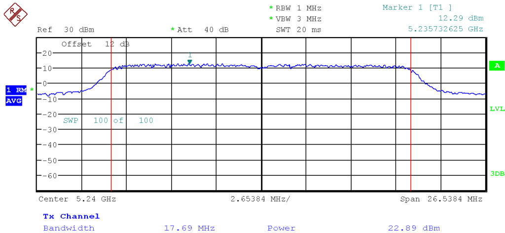
Figure 2: Output Power, Channel 48 802.11 HT20, Chain 1
