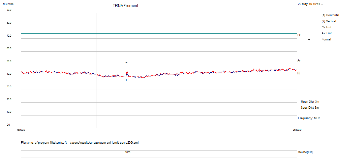
Figure 134: 18-26.5 GHz 802.11a Mode Channel 44
