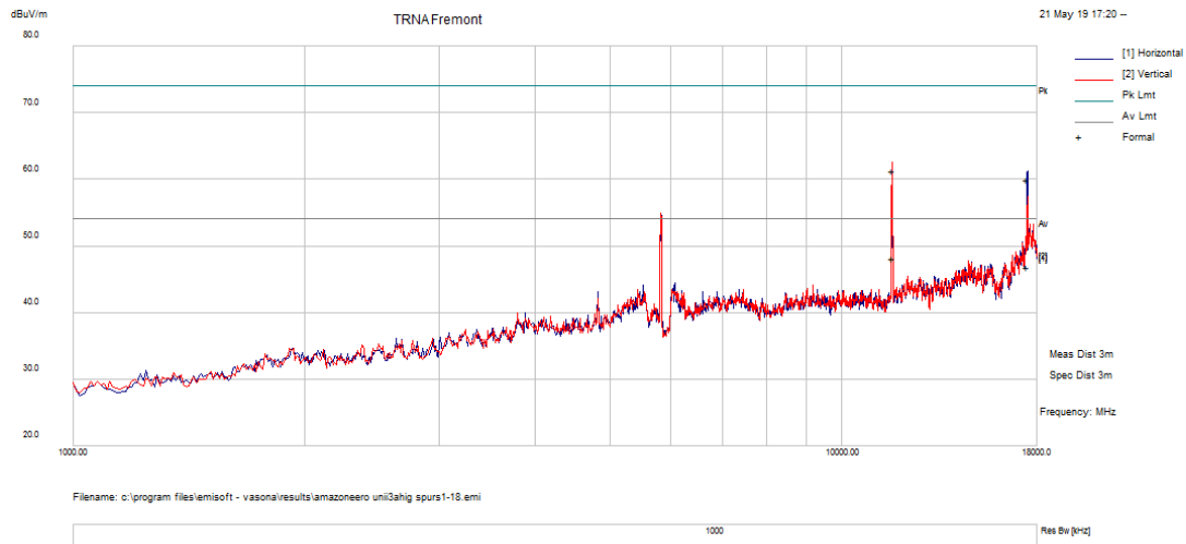
Figure 149: 1-18GHz 802.11a Mode Channel 165
