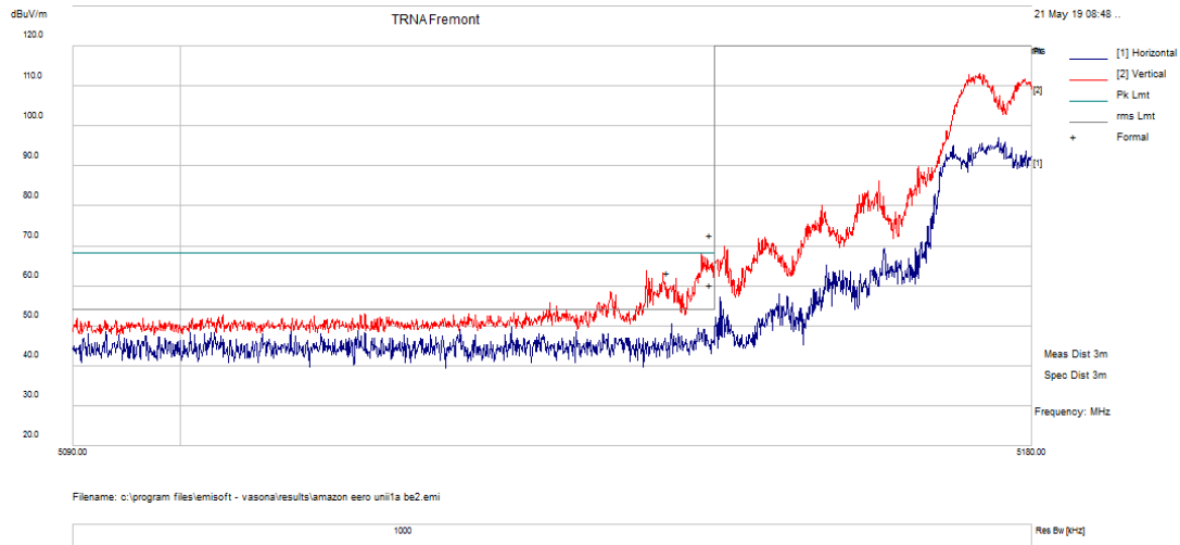
Figure 117: UNII-1 Low Band Edge for 802.11a No HT 6Mbps at 5180 MHz-peak
