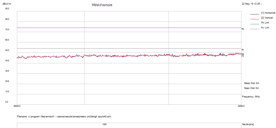
Figure 151: 26.5-40 GHz 802.11a Mode Channel 165
