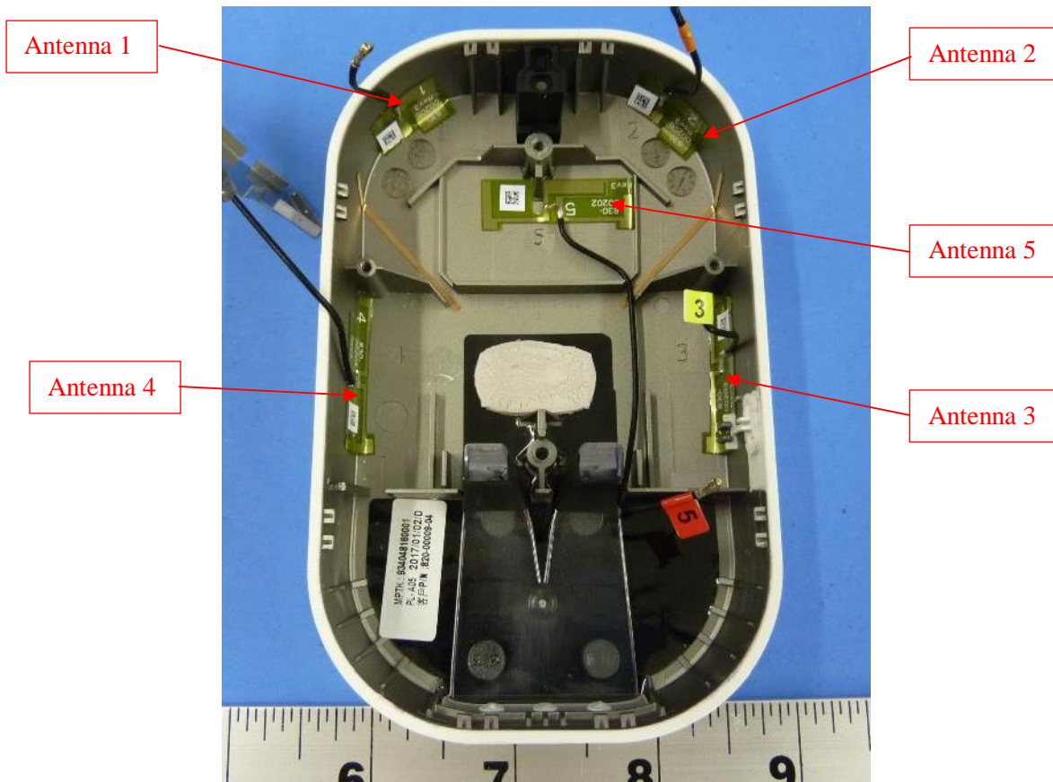
Figure 5: FPCB Antenna Location (Top – chassis)
