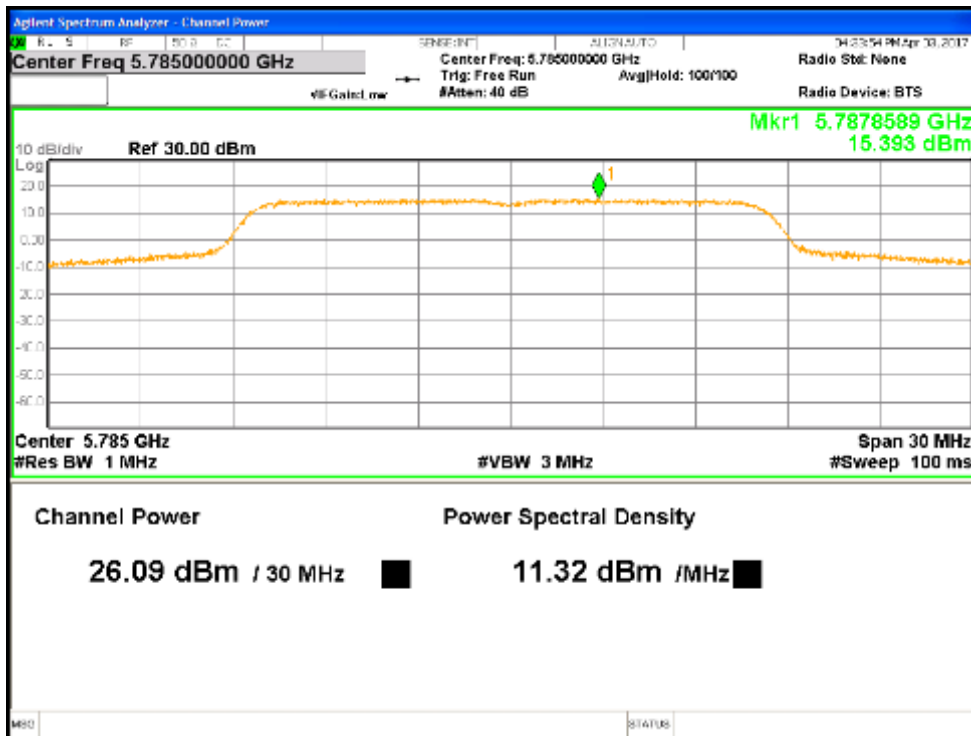
Figure 1: Non-Beamforming Max Transmitted Power, 5785 MHz at 11a, Chain 0
