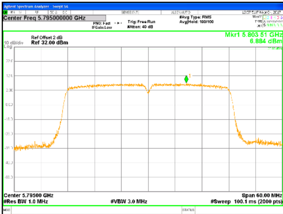
Figure 24: Beamforming Power Spectral Density, 5795 MHz at VHT40, Chain 0
