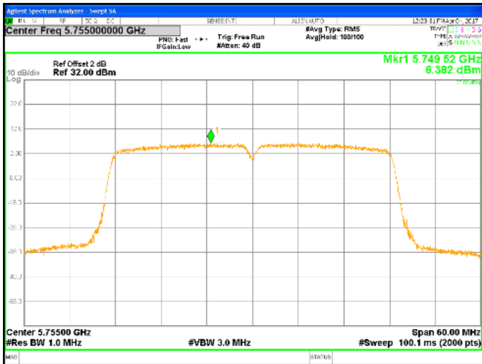
Figure 18: Non Beamforming Power Spectral Density, 5755 MHz at HT40, Chain 0
