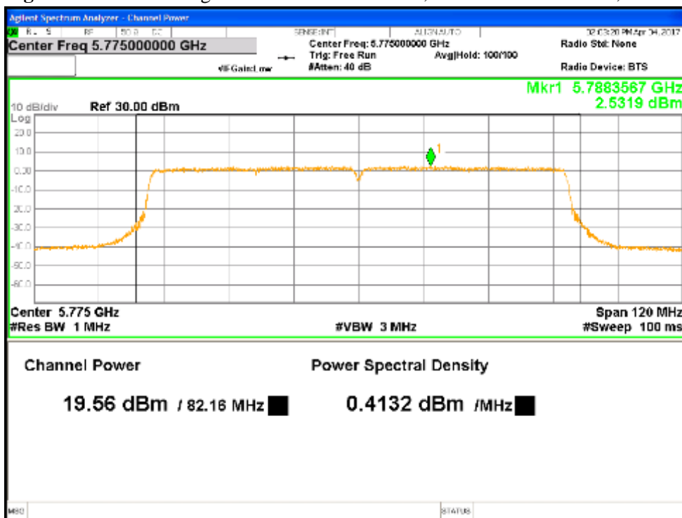
Figure 10: Beamforming Max Transmitted Power, 5775 MHz at VHT80, Chain 0
