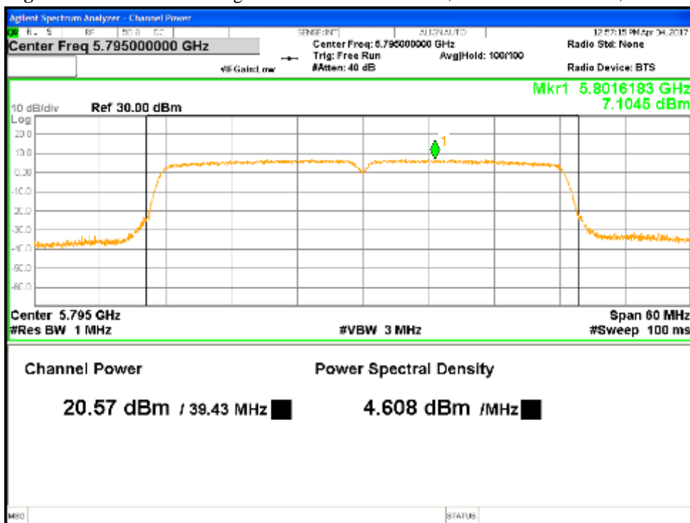
Figure 4: Non Beamforming Max Transmitted Power, 5795 MHz at VHT40, Chain 0
