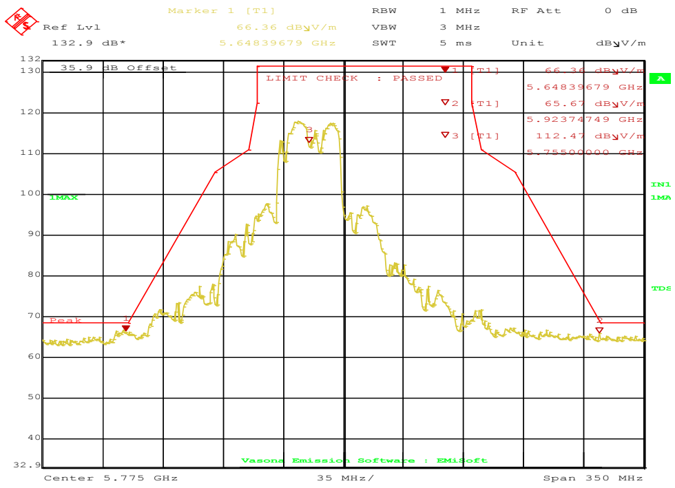
Figure 90: Radiated Emission Below Edge for VHT40 5755 MHz – Vert. (Pk)
