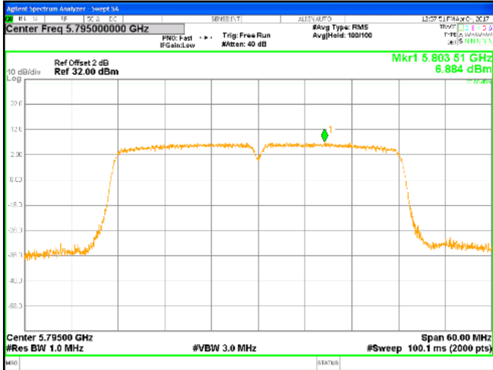
Figure 19: Non Beamforming Power Spectral Density, 5795 MHz at VHT40, Chain 0
