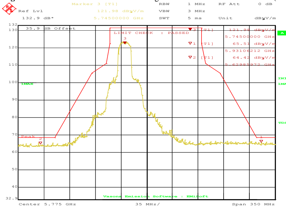
Figure 83: Radiated Emission Below Edge for HT20 5745 MHz – Horz. (Pk)
