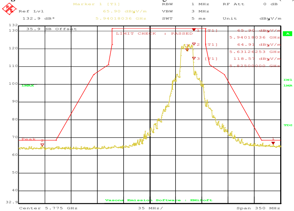
Figure 81: Radiated Emission Above Edge for 11a 5825 MHz – Horz. (Pk)
