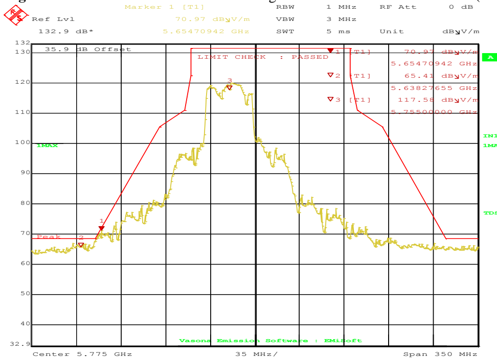
Figure 87: Radiated Emission Below Edge for HT40 5755 MHz – Horz. (Pk)
