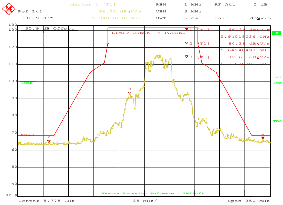
Figure 92: Radiated Emission Above Edge for VHT40 5795 MHz – Vert. (Pk)
