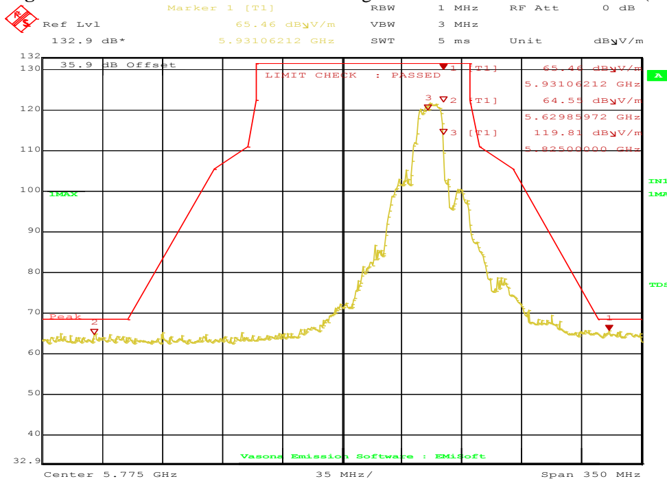
Figure 85: Radiated Emission Above Edge for HT20 5825 MHz – Vert. (Pk)
