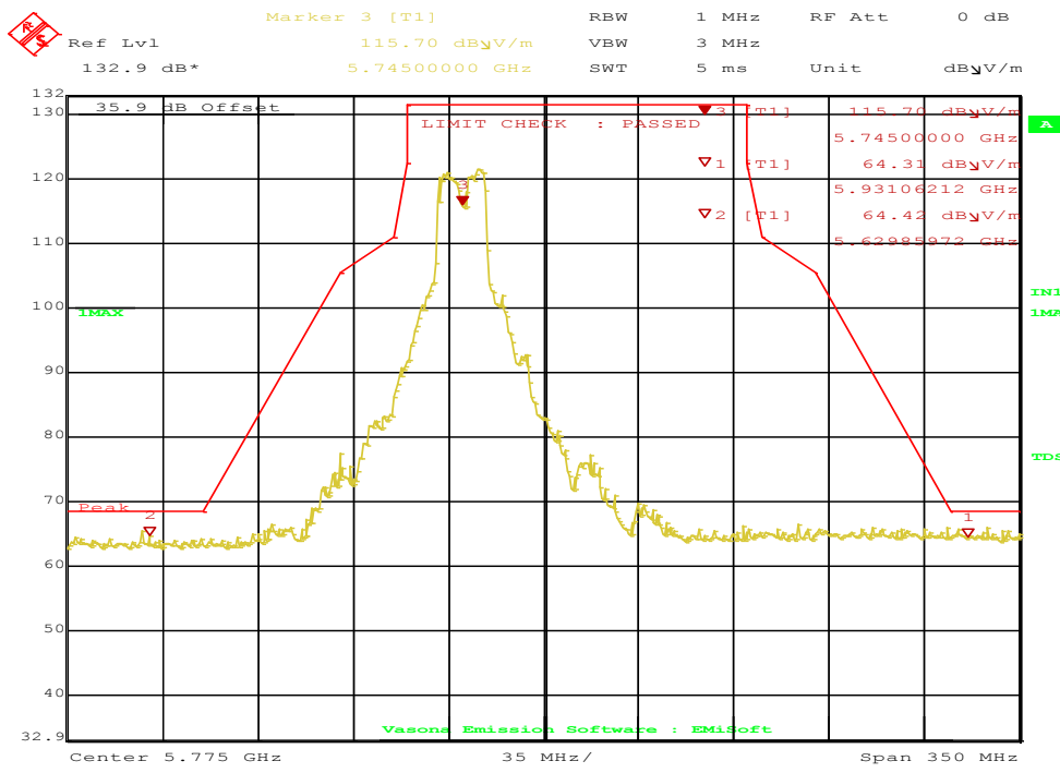
Figure 82: Radiated Emission Below Edge for HT20 5745 MHz – Vert. (Pk)
