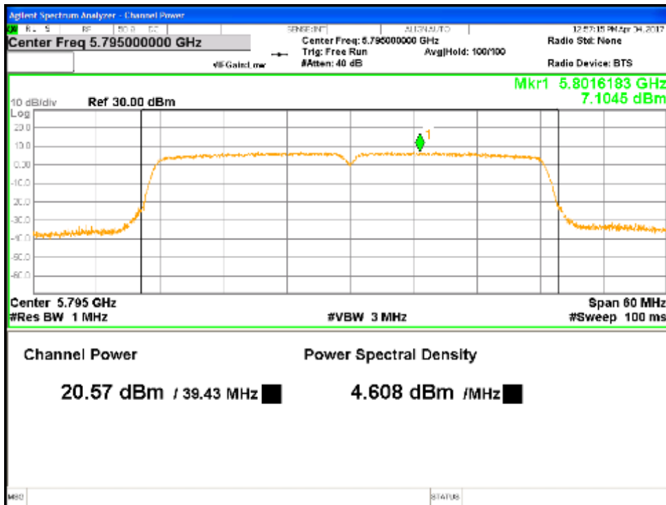
Figure 9: Beamforming Max Transmitted Power, 5795 MHz at VHT40, Chain 0
