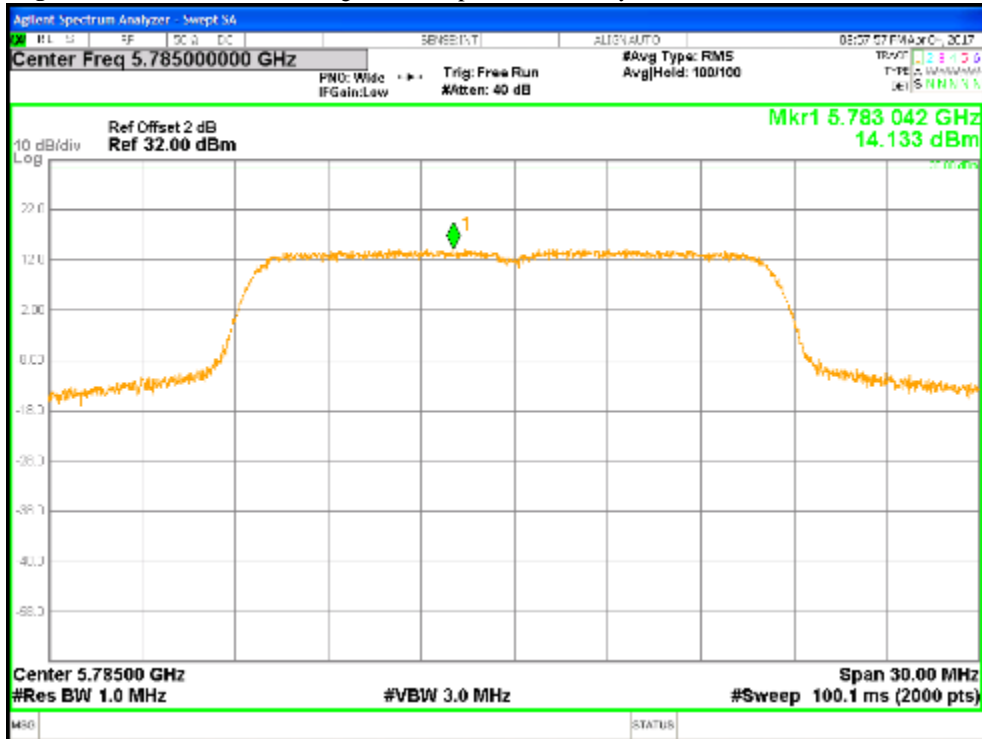
Figure 21: Beamforming Power Spectral Density, 5785 MHz at 802.11a, Chain 0
