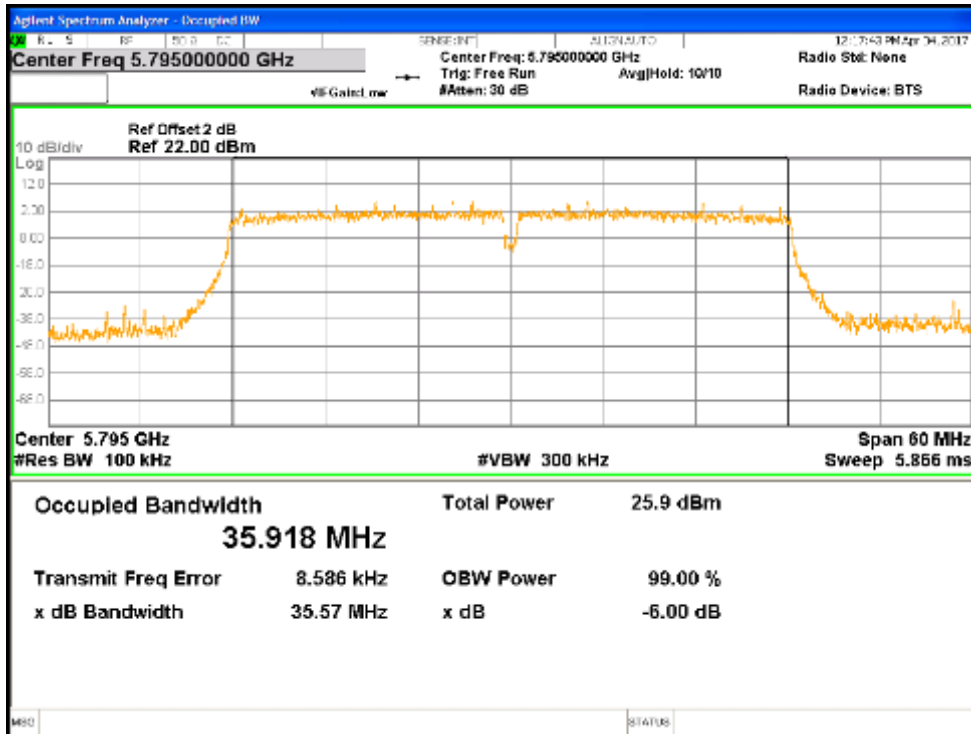
Figure 13: 6dB & 99% Occupied Bandwidth, 5795 MHz at HT40 MCS0, Chain 0
