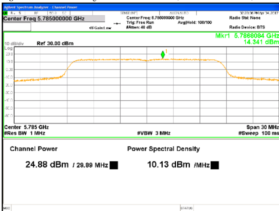
Figure 6: Beamforming Max Transmitted Power, 5785 MHz at 11a, Chain 0
