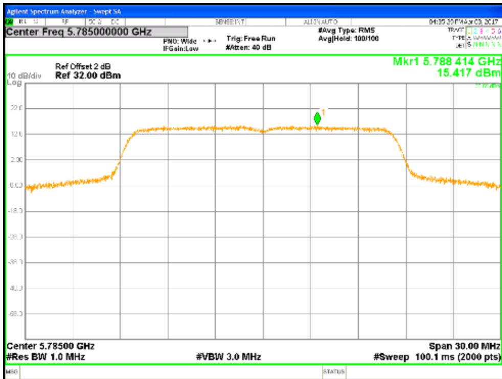
Figure 16: Non Beamforming Power Spectral Density, 5785 MHz at 802.11a, Chain 0
