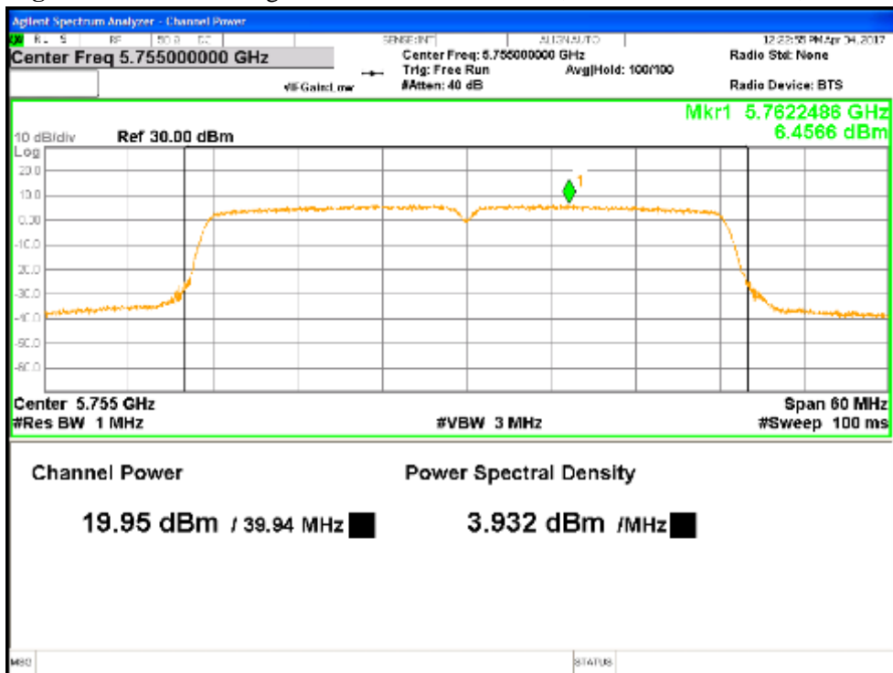
Figure 8: Beamforming Max Transmitted Power, 5755 MHz at HT40, Chain 0
