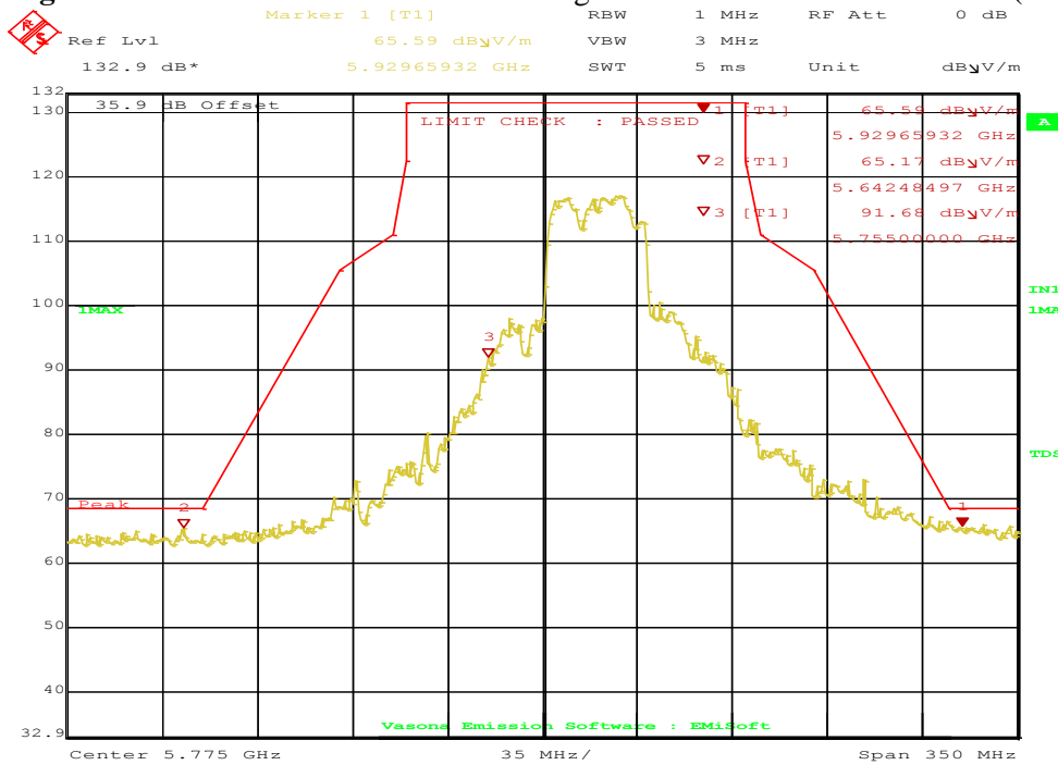
Figure 89: Radiated Emission Above Edge for HT40 5795 MHz – Horz. (Pk)
