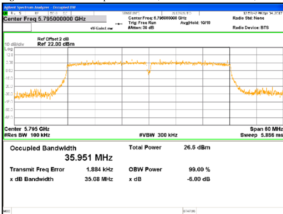
Figure 14: 6dB & 99% Occupied Bandwidth, 5795 MHz at VHT40 MCS0, Chain 0
