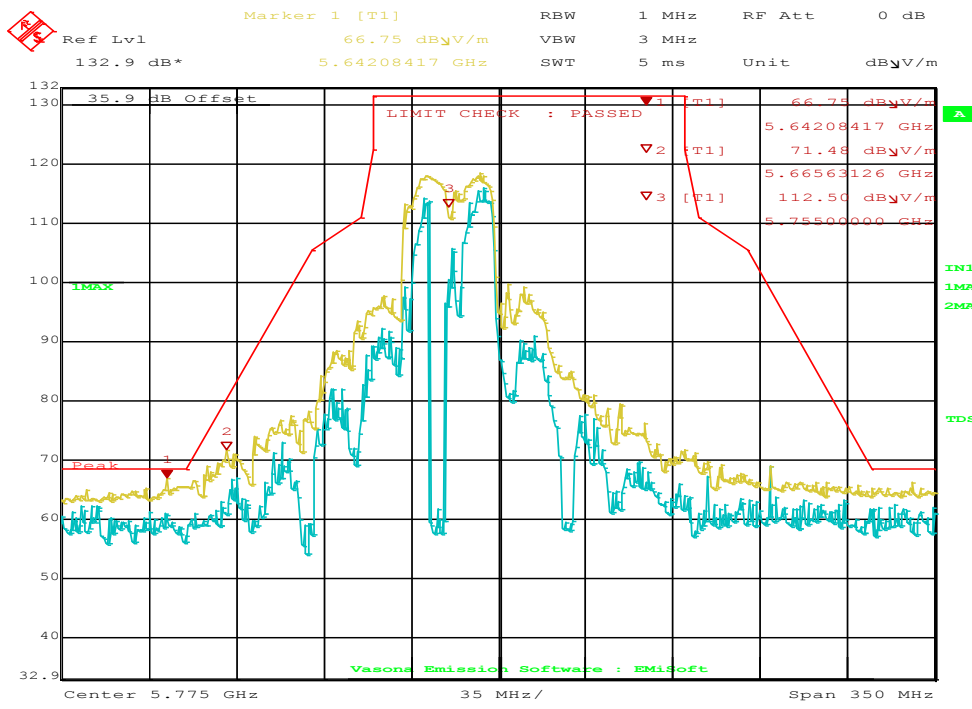
Figure 86: Radiated Emission Below Edge for HT40 5755 MHz – Vert. (Pk)
