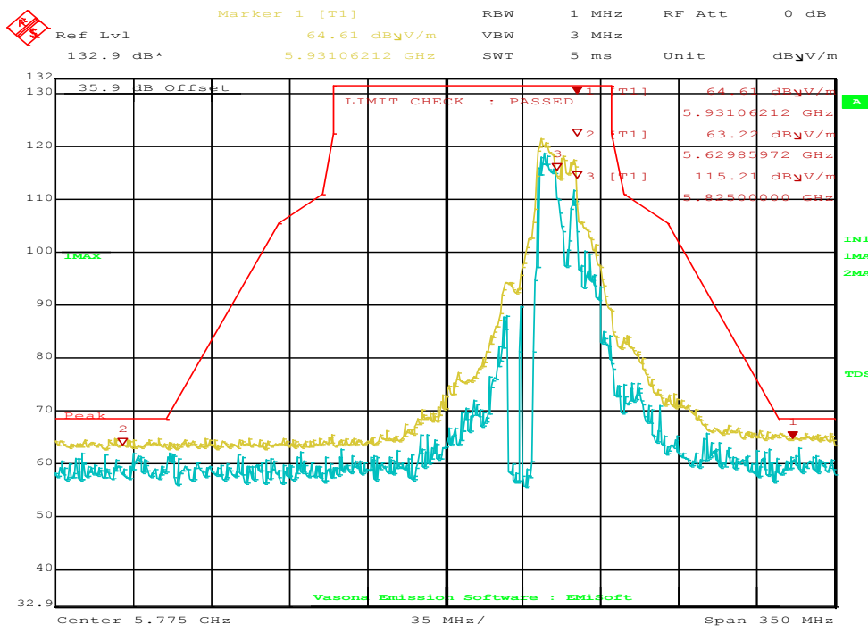
Figure 84: Radiated Emission Above Edge for HT20 5825 MHz – Horz. (Pk)
