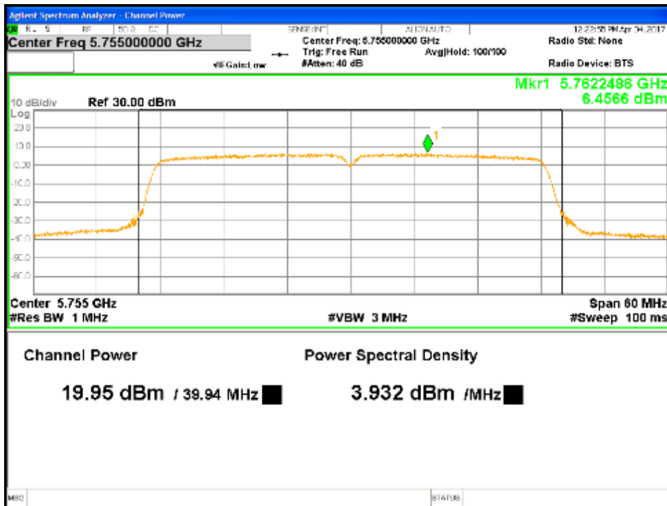
Figure 3: Non Beamforming Max Transmitted Power, 5755 MHz at HT40, Chain 0
