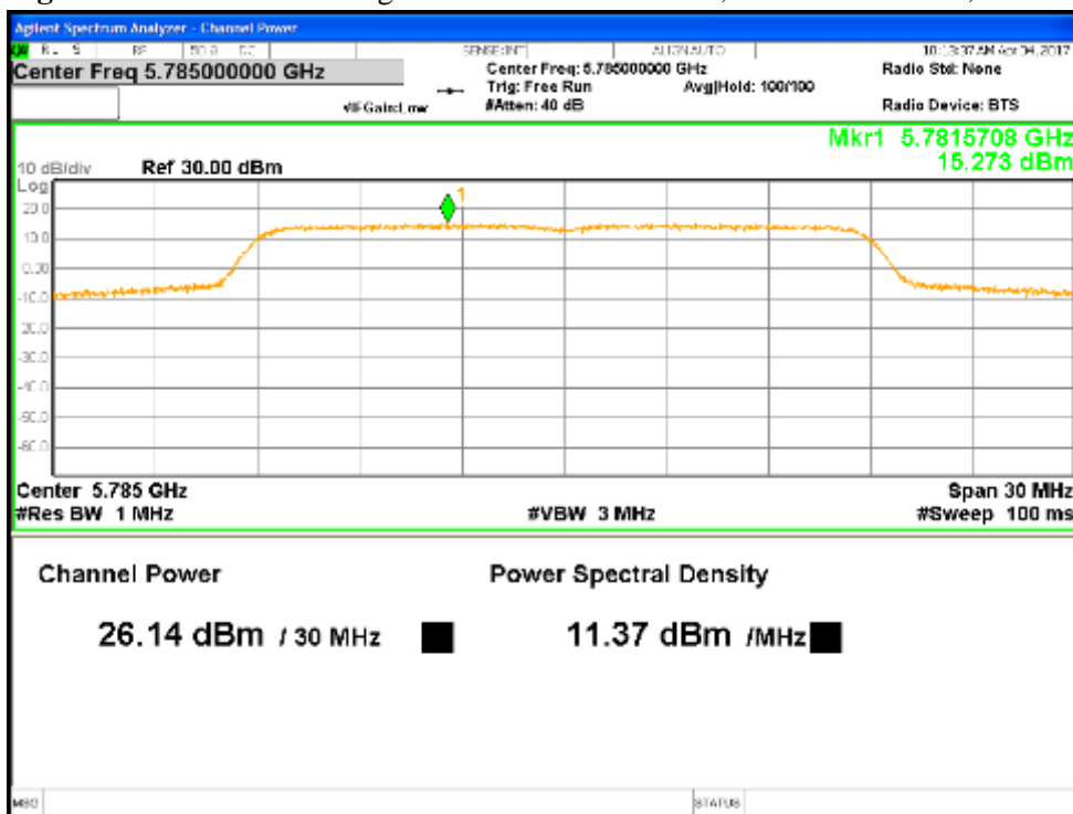
Figure 2: Non-Beamforming Max Transmitted Power, 5785 MHz at HT20, Chain 0
