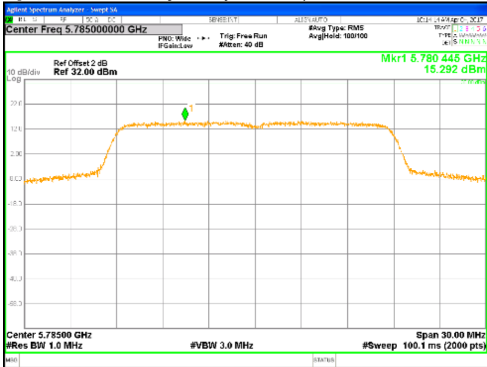
Figure 17: Non Beamforming Power Spectral Density, 5785 MHz at HT20, Chain 0
