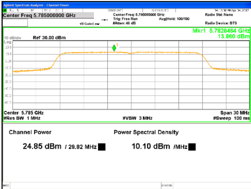
Figure 7: Beamforming Max Transmitted Power, 5785 MHz at HT20, Chain 0
