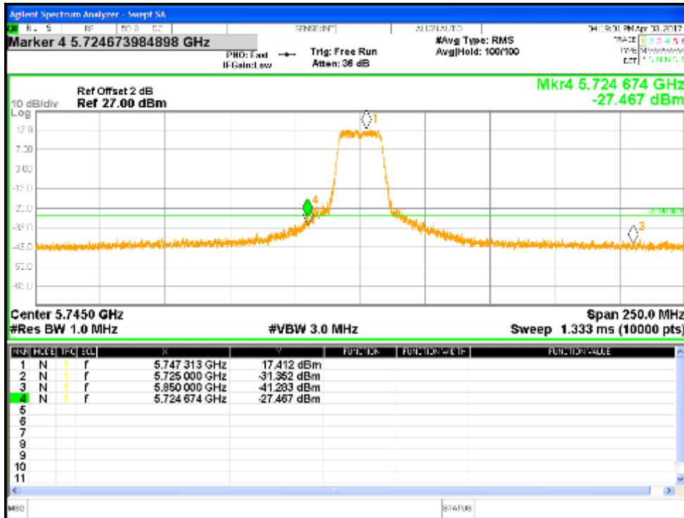
Figure 26: Measured Below Edge for 802.11a-6Mbps at 5745 MHz, Chain 0
