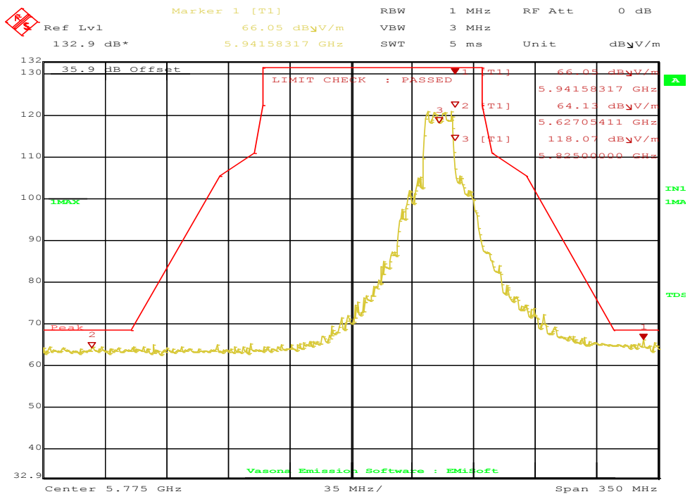
Figure 80: Radiated Emission Above Edge for 11a 5825 MHz – Vert. (Pk)
