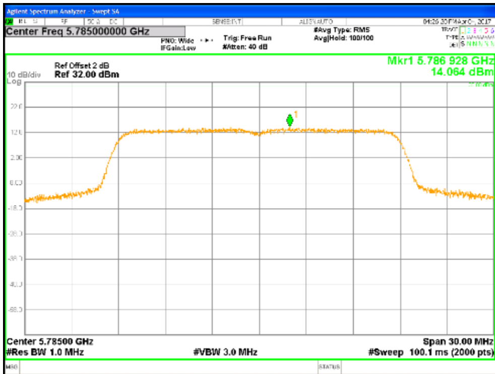
Figure 22: Beamforming Power Spectral Density, 5785 MHz at HT20, Chain 0
