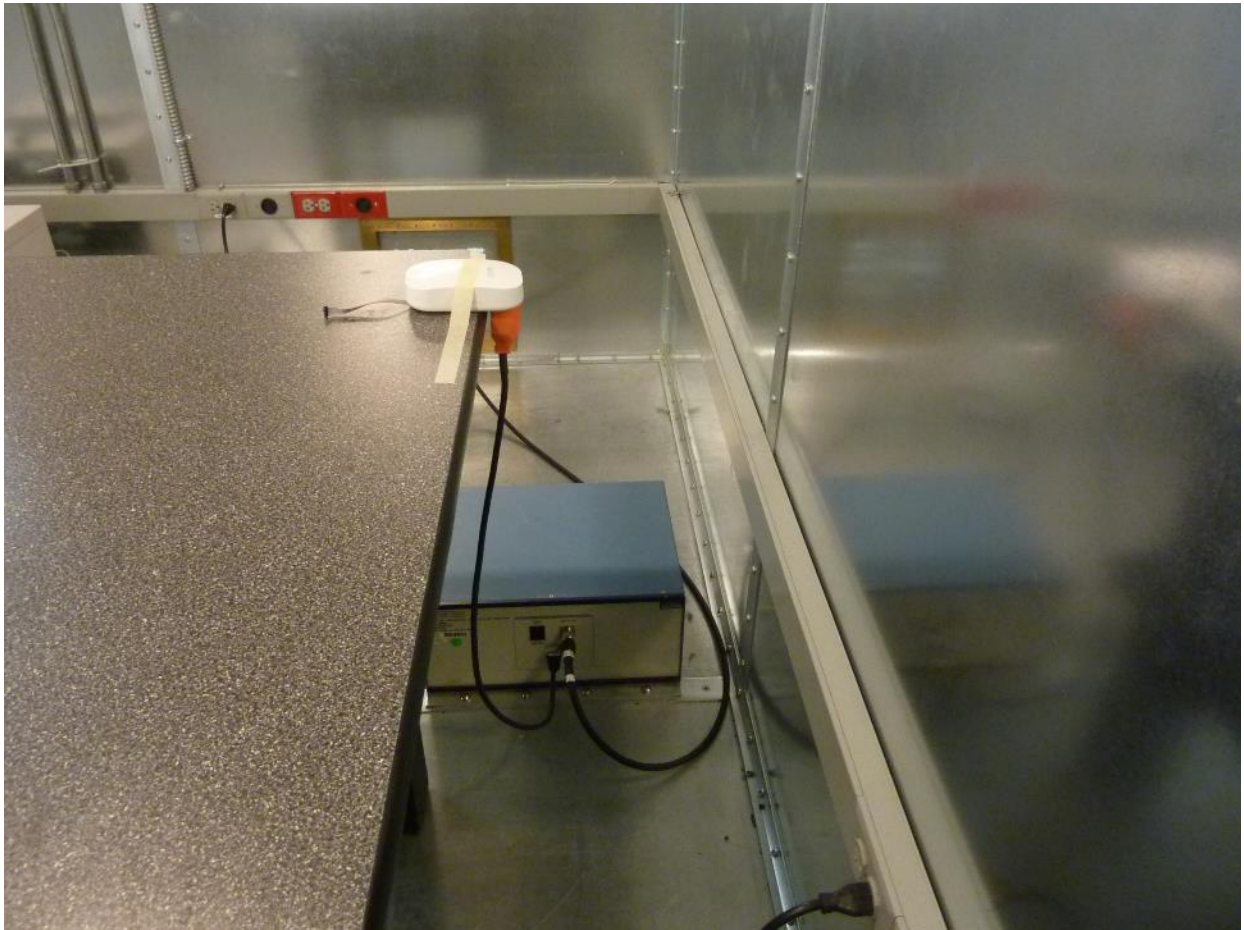
Figure 9: Conducted Emission Test Setup (Side)
