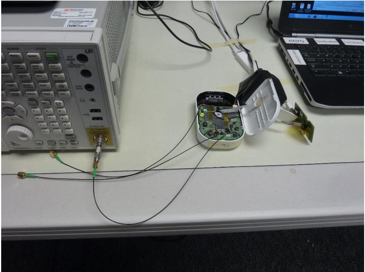
Figure 7: RF Conducted Test Setup – Closeup
