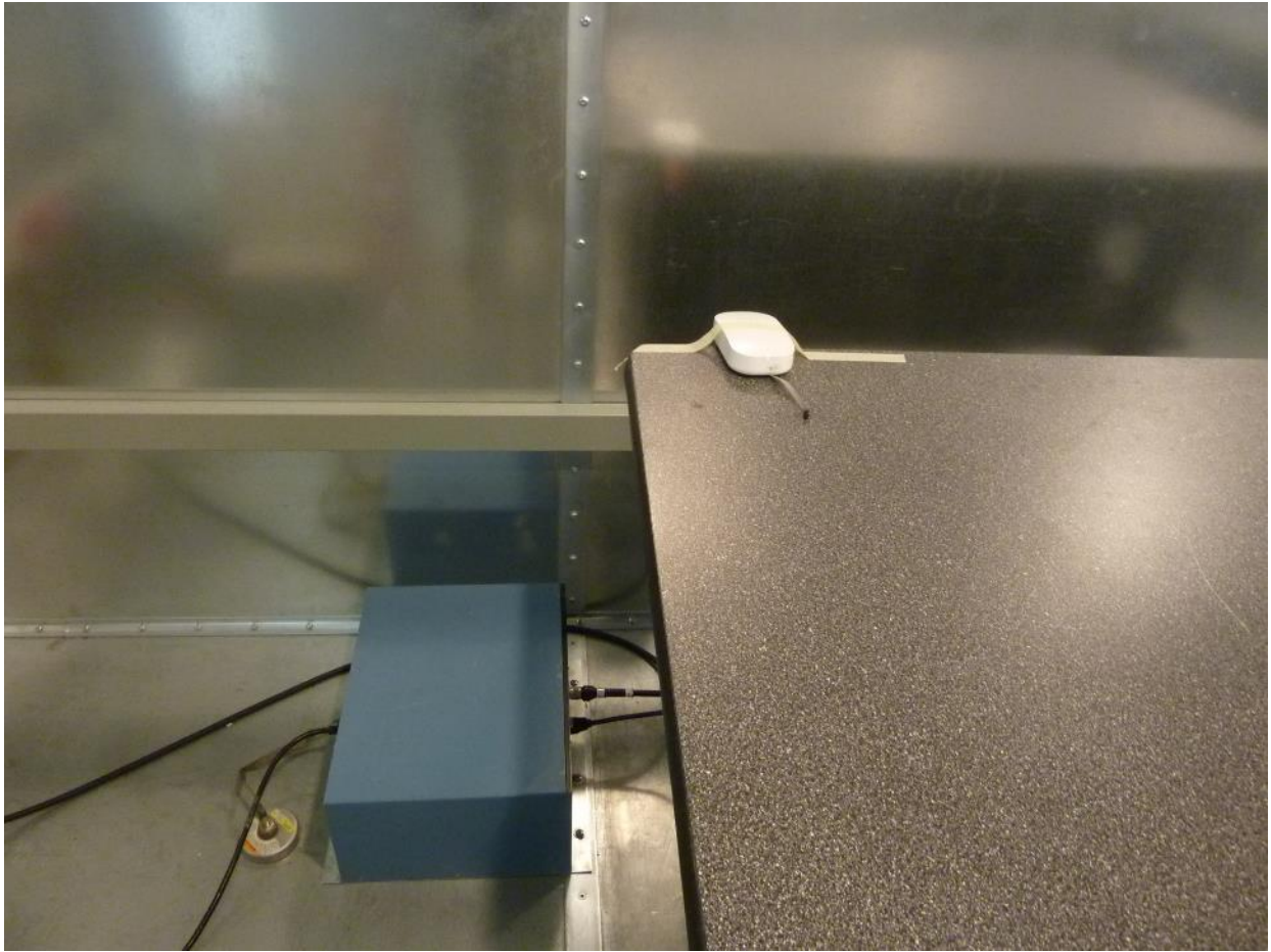
Figure 8: Conducted Emission Test Setup (Front)
