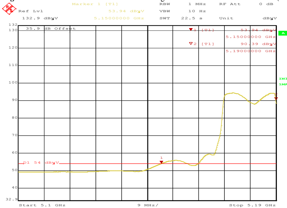
Figure 90: Radiated Emission 5150.0 MHz Edge for VHT40 5190 MHz – Horiz. (Ave)
