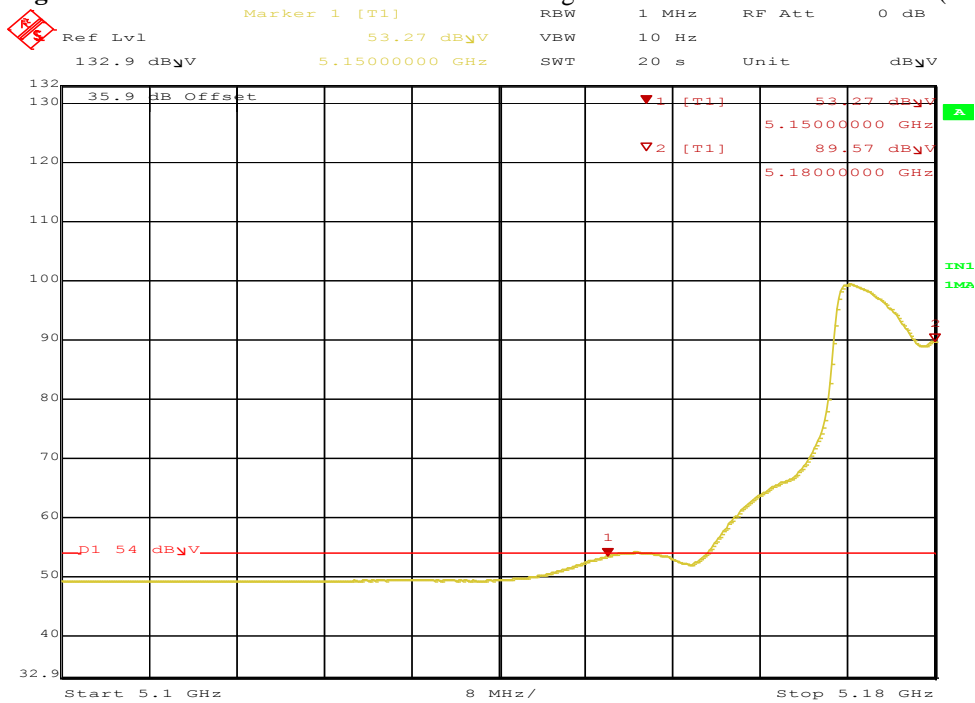
Figure 84: Radiated Emission 5150.0 MHz Edge for HT20 5180 MHz – Vert. (Ave)
