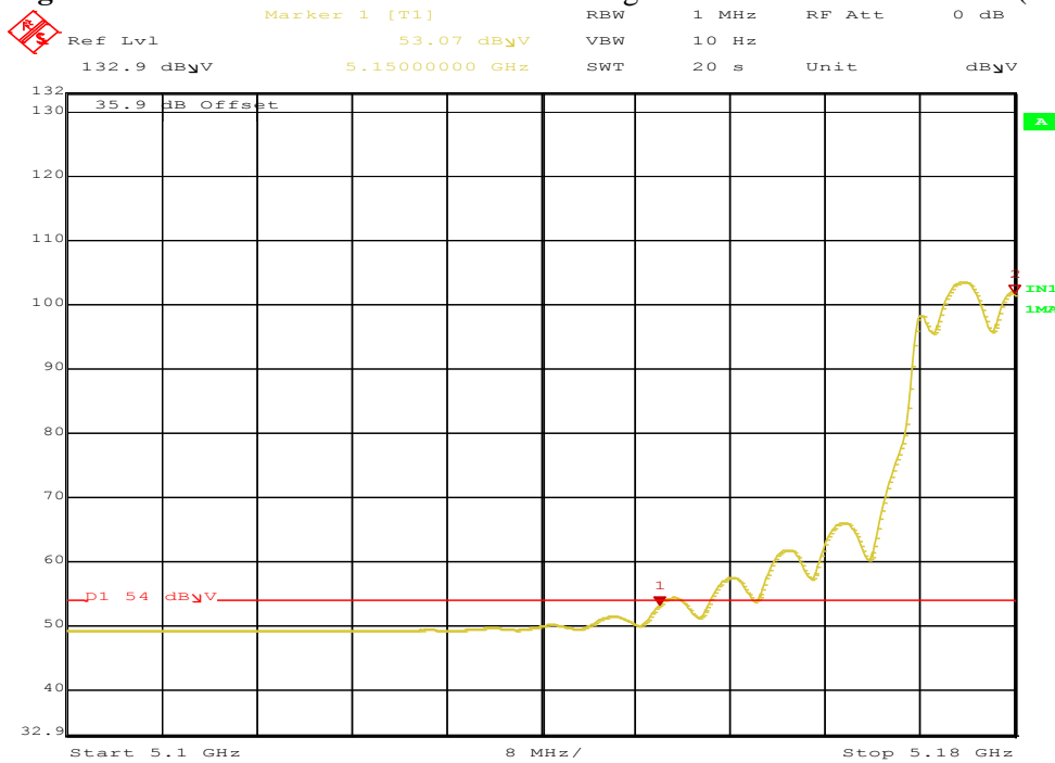
Figure 78: Radiated Emission 5150.0 MHz Edge for 11a 5180 MHz – Horz. (Ave)
