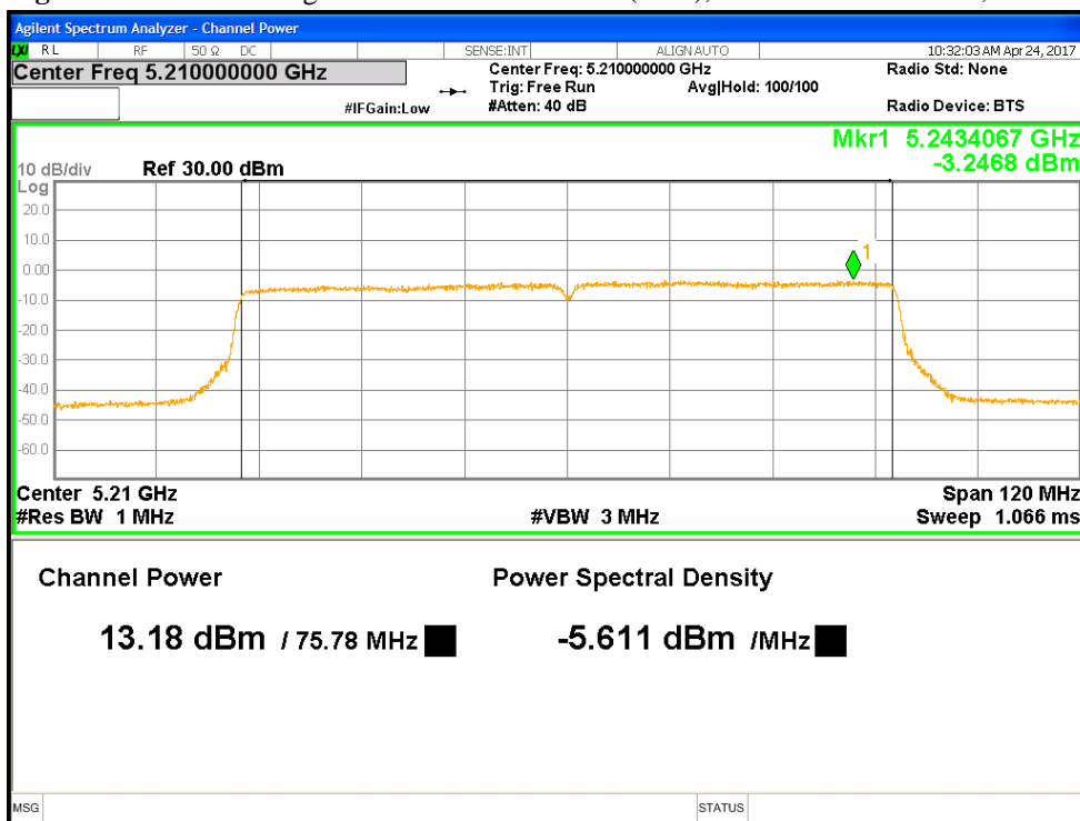
Figure 20: Beamforming Max Transmitted Power (RSS), 5210 MHz at VHT80, Chain 1
