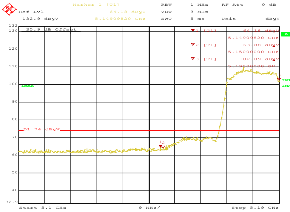
Figure 87: Radiated Emission 5149.1 MHz Edge for HT40 5190 MHz – Vert. (Pk)
