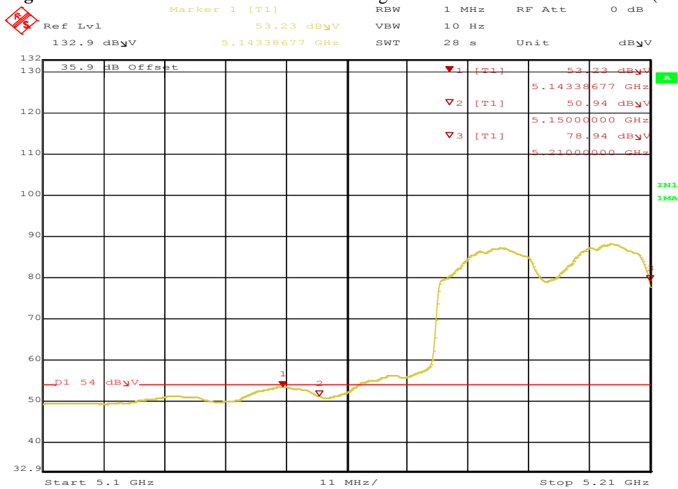
Figure 94: Radiated Emission 5143.4 MHz Edge for VHT80 5210 MHz – Horz. (Ave)
