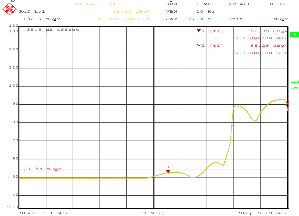
Figure 92: Radiated Emission 5150.0 MHz Edge for VHT40 5190 MHz – Vert. (Ave)
