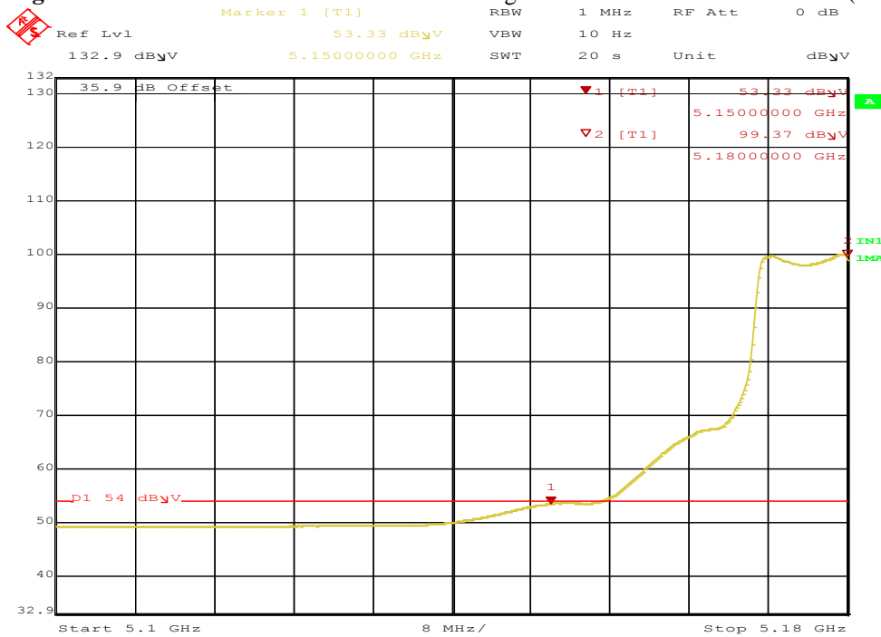
Figure 82: Radiated Emission 5150.0 MHz Edge for HT20 5180 MHz – Horz. (Ave)
