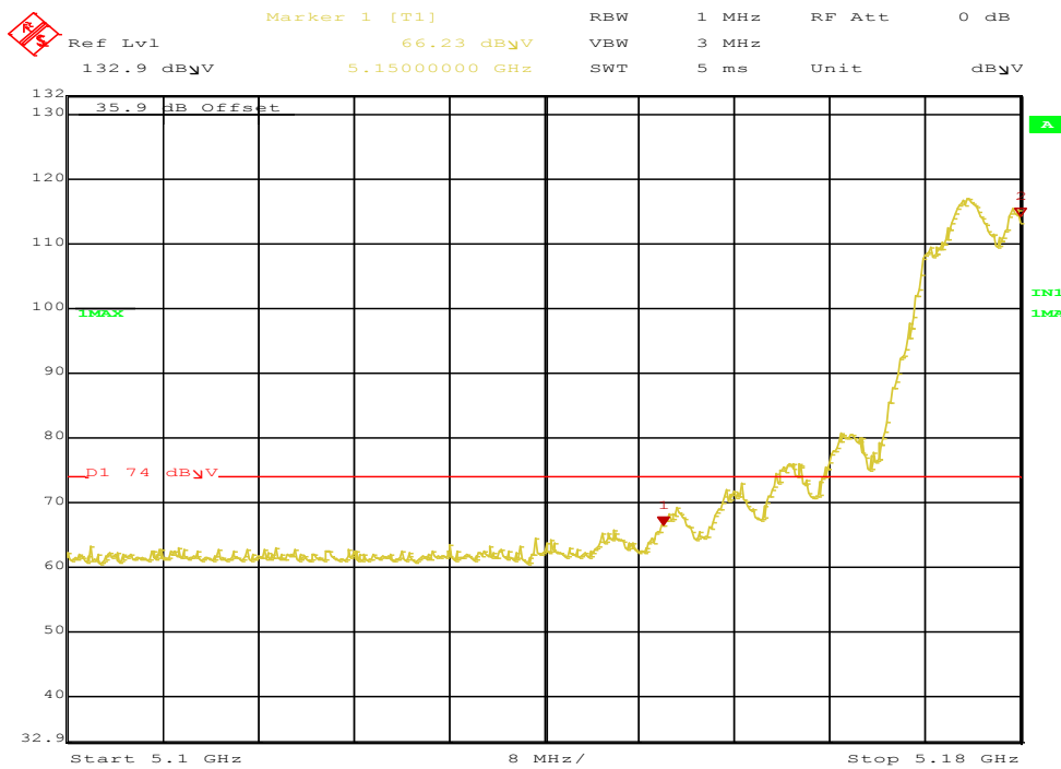
Figure 77: Radiated Emission 5150.0 MHz Edge for 11a 5180 MHz – Horz. (Pk)
