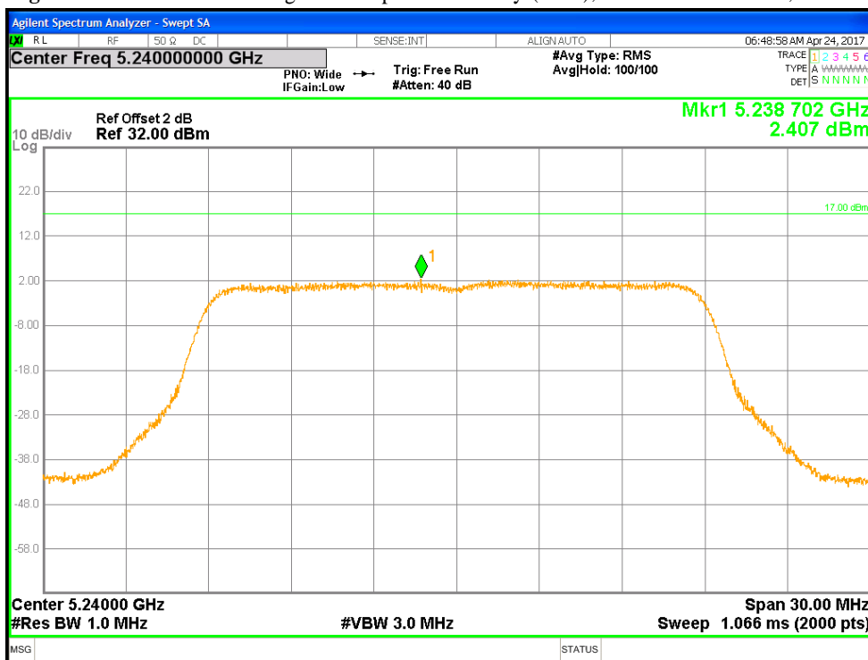
Figure 29: Non-Beamforming Power Spectral Density (RSS), 5240 MHz at HT20, Chain 1
