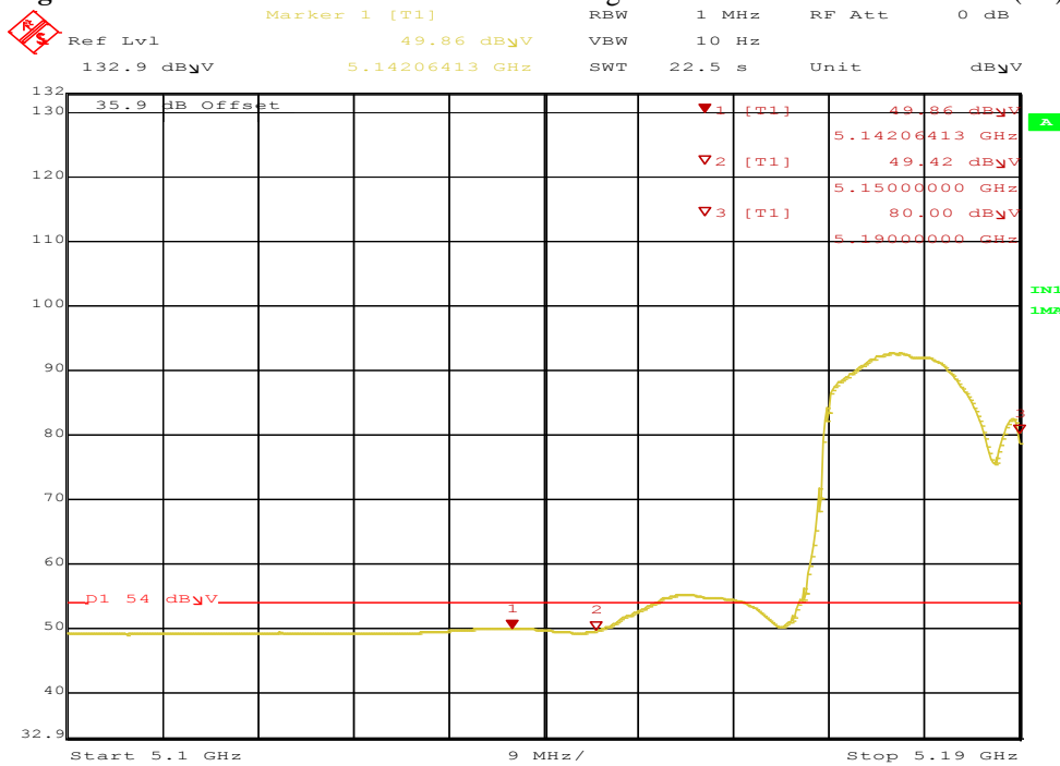
Figure 88: Radiated Emission 5142.1 MHz Edge for HT40 5190 MHz – Vert. (Ave)
