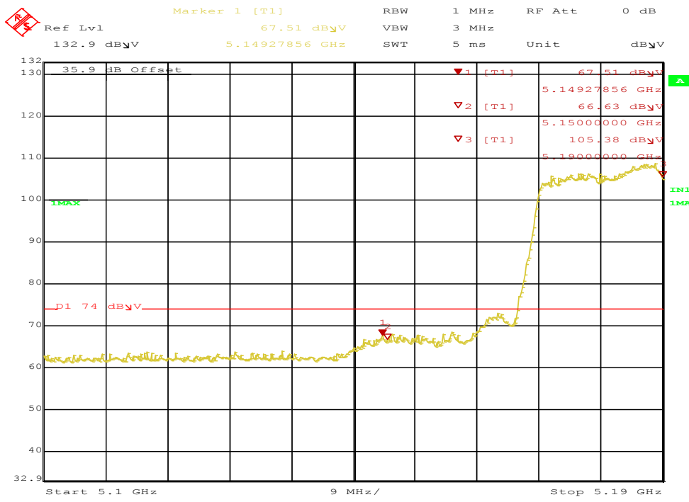
Figure 91: Radiated Emission 5149.3 MHz Edge for VHT40 5190 MHz – Vert. (Pk)
