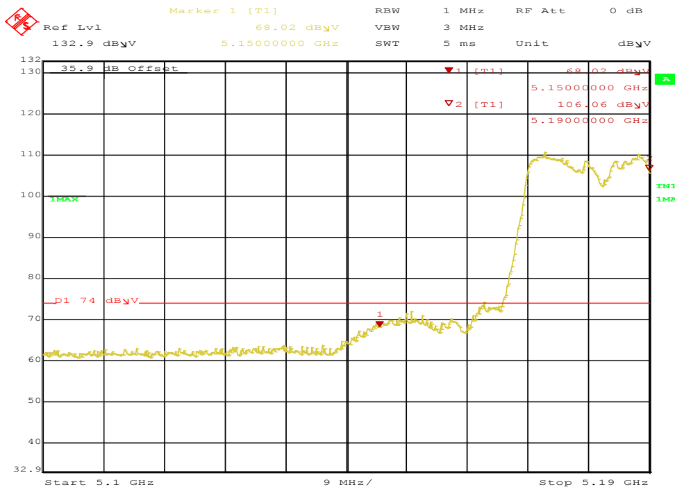
Figure 89: Radiated Emission 5150.0 MHz Edge for VHT40 5190 MHz – Horiz. (Pk)
