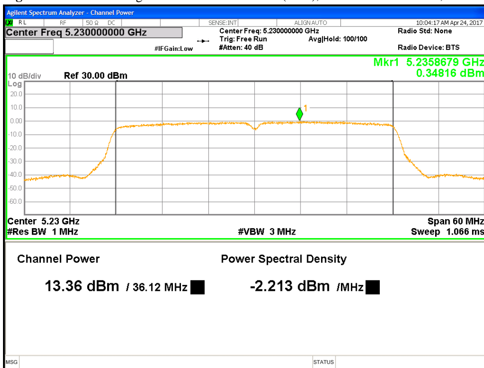
Figure 18: Beamforming Max Transmitted Power (RSS), 5230 MHz at VHT40, Chain 1
