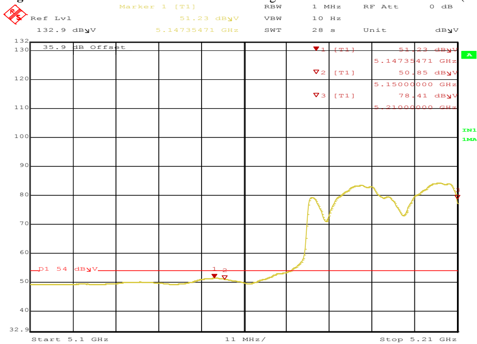
Figure 96: Radiated Emission 5147.4 MHz Edge for VHT80 5210 MHz – Vert. (Ave)
