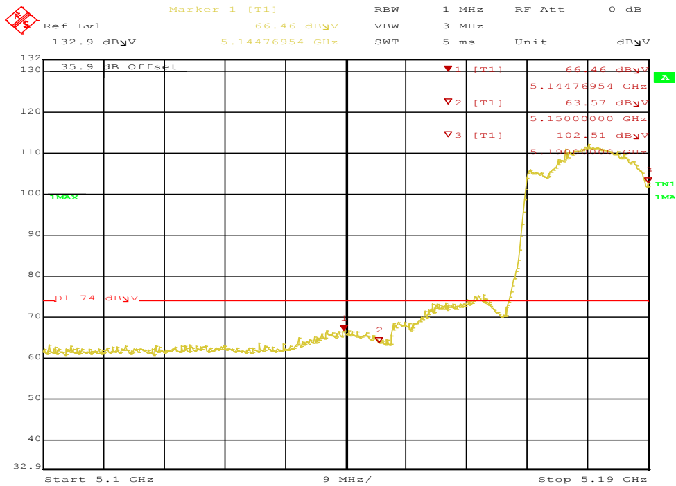
Figure 85: Radiated Emission 5144.8 MHz Edge for HT40 5190 MHz – Horz. (Pk)
