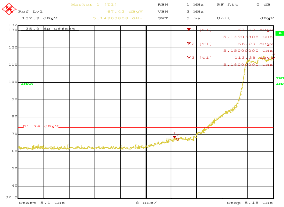
Figure 81: Radiated Emission 5149.0 MHz Edge for HT20 5180 MHz – Horz. (Pk)
