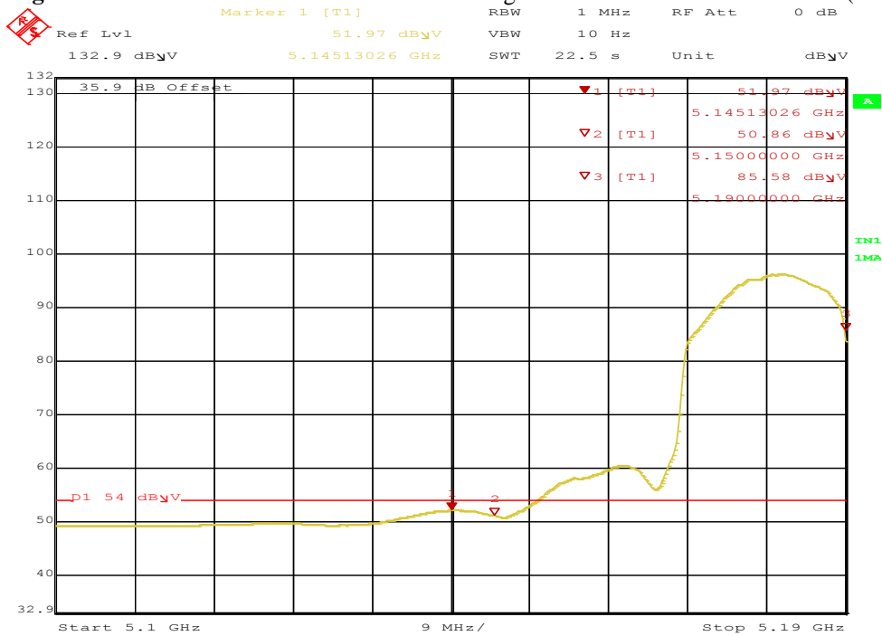
Figure 86: Radiated Emission 5145.1 MHz Edge for HT40 5190 MHz – Horz. (Ave)
