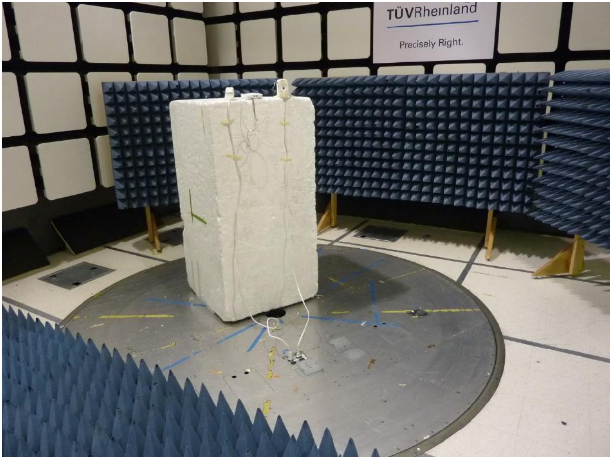
Figure 5: Test Setup for 1 GHz to 25 GHz
