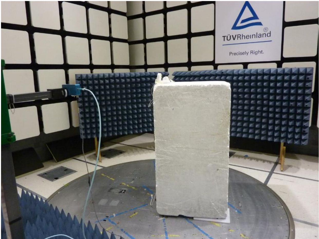
Figure 4: Test Setup for 18 GHz to 25 GHz
