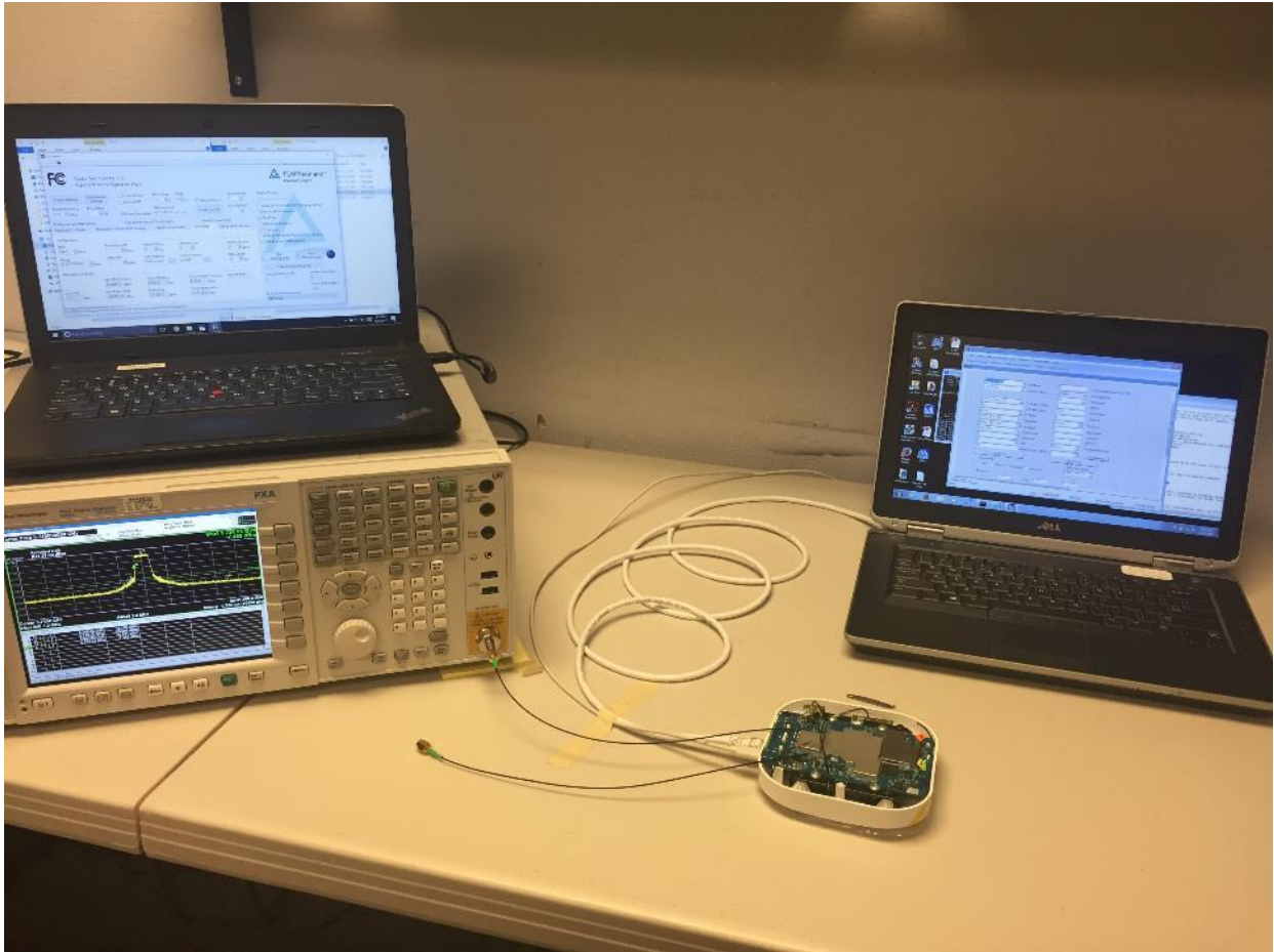
Figure 6: RF Conducted Test Setup
