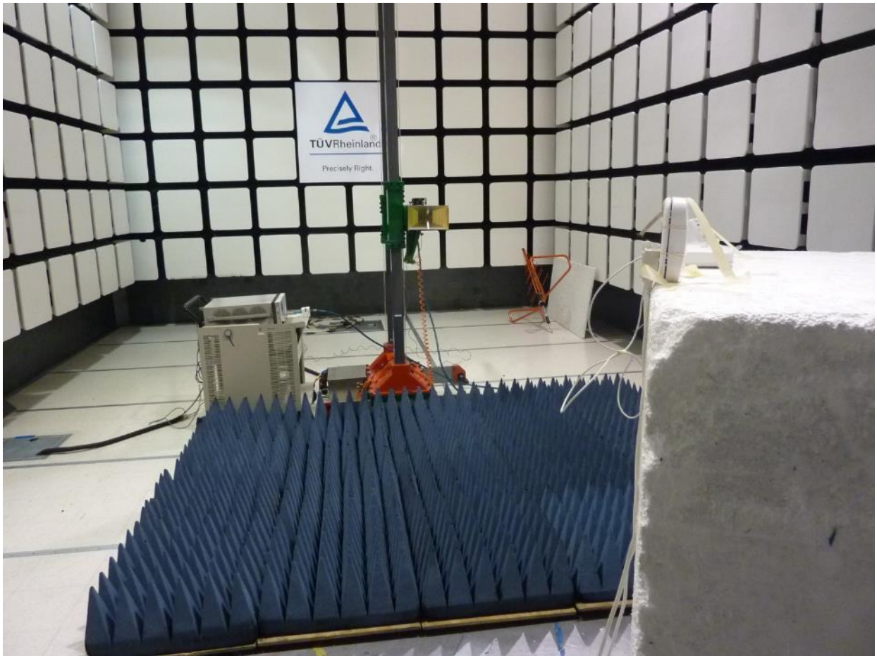
Figure 3: Test Setup for 1 GHz to 18 GHz
