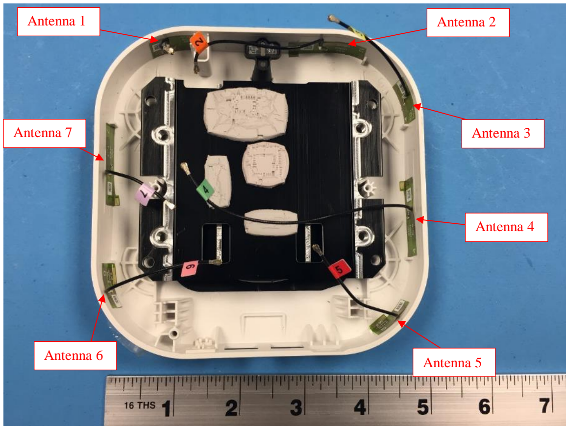
Figure 7: PCB Antenna Location (Top – chassis)
