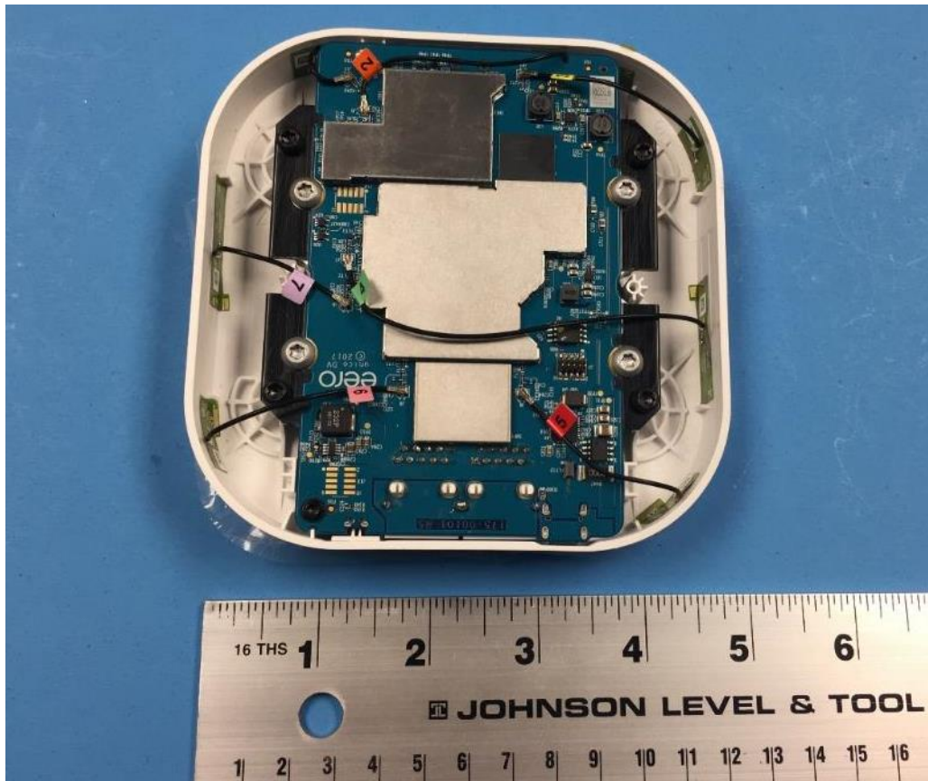
Figure 1: Photo of EUT (Open Chassis)
