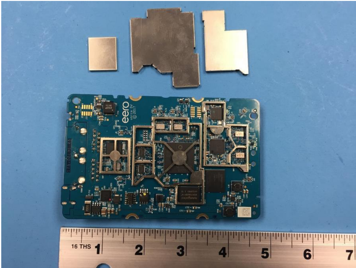
Figure 4: Photo of PCB (Top – removed shield cover)
