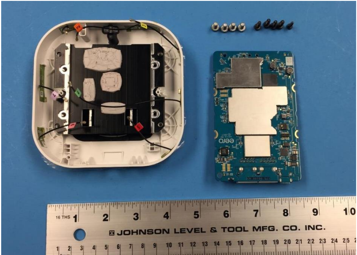
Figure 2: Photo of EUT - PCB removed
