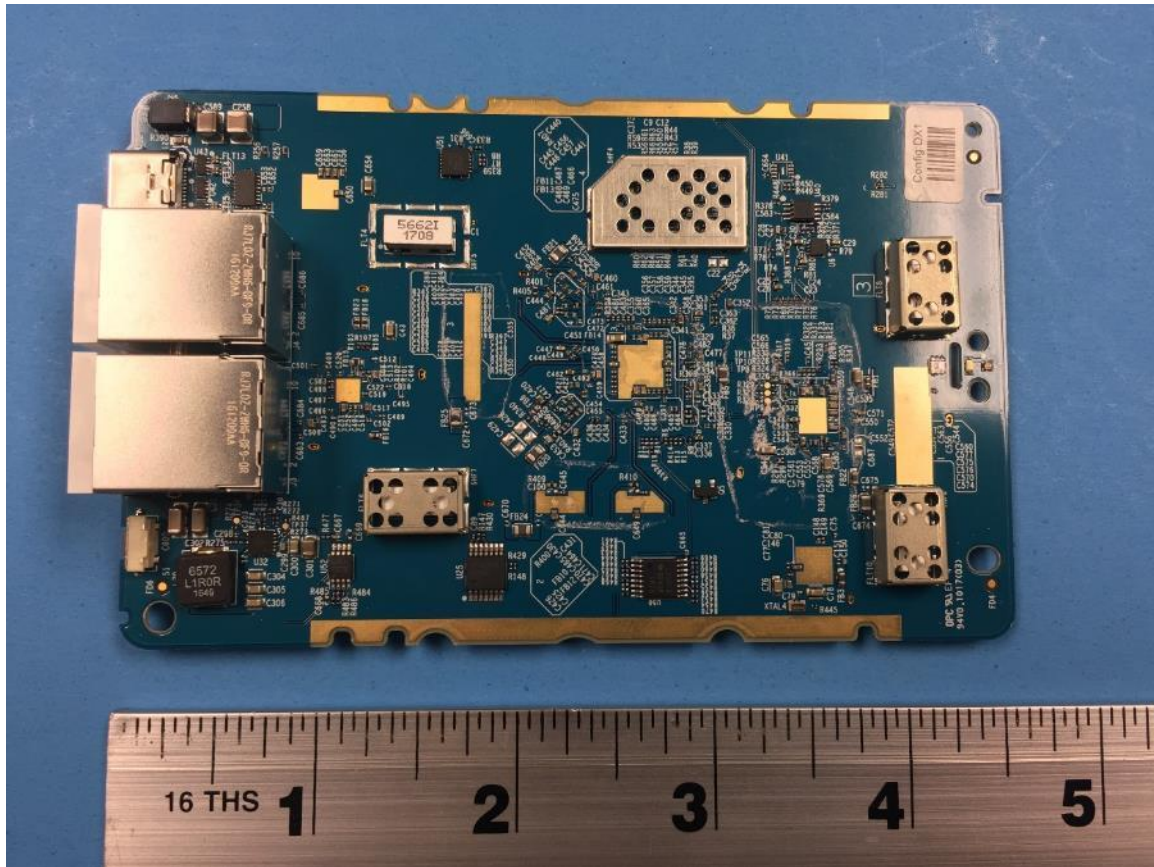
Figure 5: Photo of PCB (Bottom)
