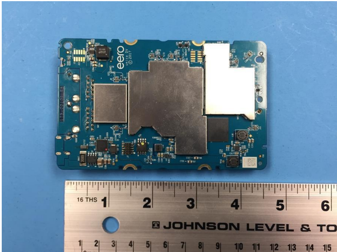
Figure 3: Photo of PCB (Top)
