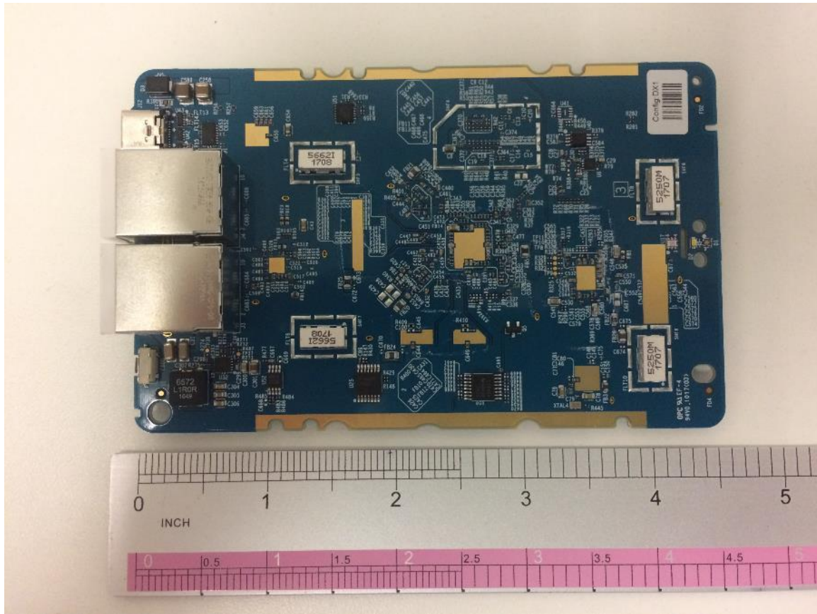
Figure 6: Photo of PCB (Bottom – removed shield cover)
