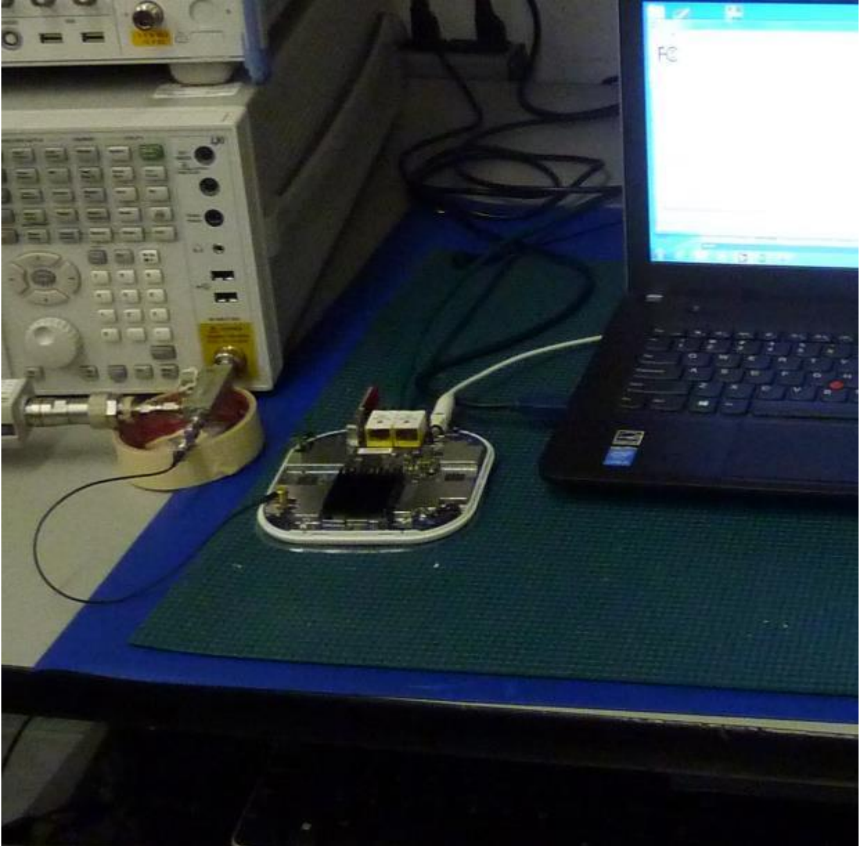
Figure 8: RF Conducted Test Setup – Closeup
