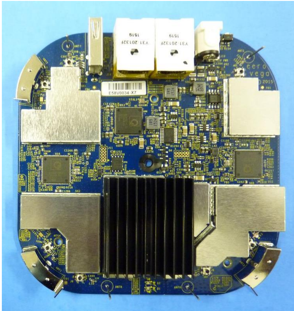
Figure 1: Photo of PCB (Top)
