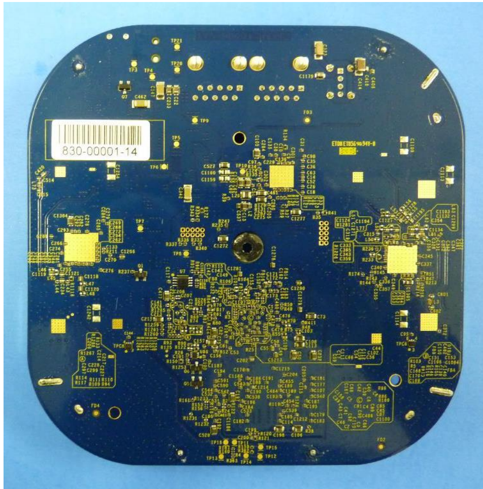
Figure 3: Photo of PCB (Bottom)
