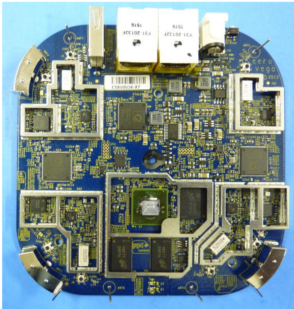
Figure 2: Photo of PCB (Top – removed shield cover)
