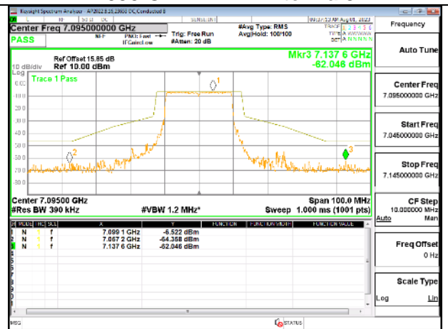
7095 CHANNEL Antenna 10
