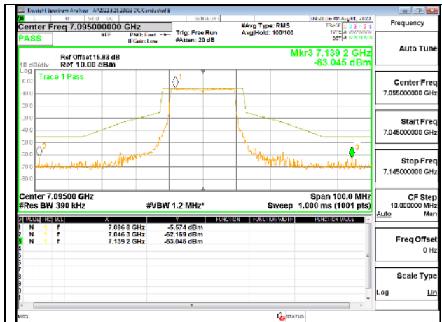
7095 CHANNEL Antenna 5
