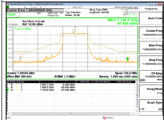
7095 CHANNEL Antenna 3
