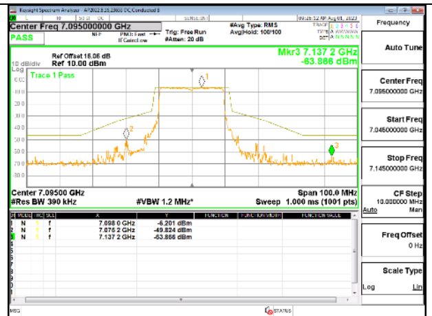
7095 CHANNEL Antenna 8
