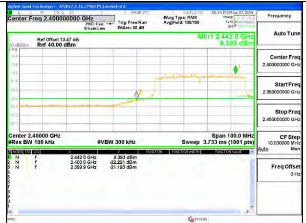
OUT-OF-BAND LOW CHANNEL 4 CHAIN 0
