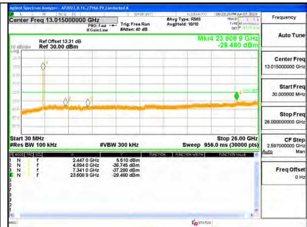
OUT-OF-BAND HIGH CHANNEL 8 CHAIN 0
