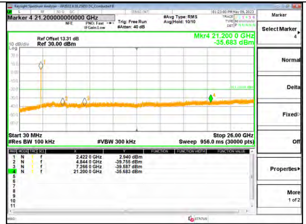
OUT-OF-BAND LOW CHANNEL 3 CHAIN 0
