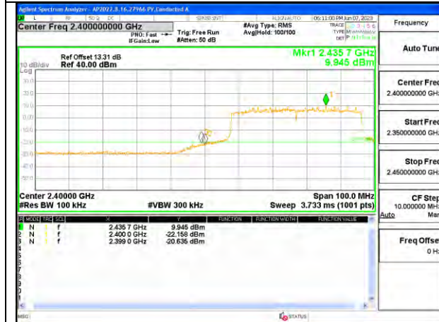
LOW CHANNEL 4 BANDEDGE CHAIN 0
