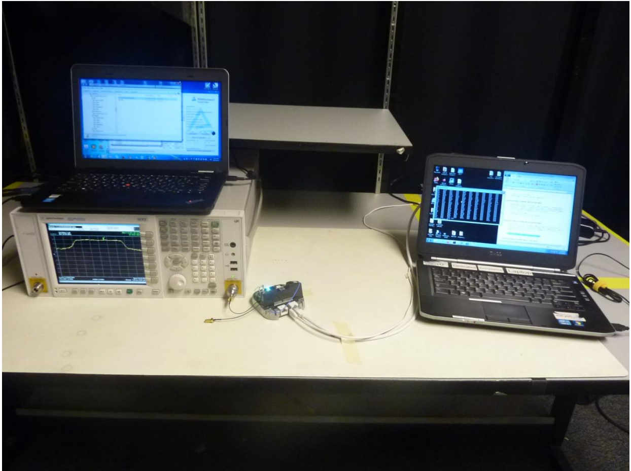
Figure 11: RF Conducted Test Setup (WiFi)
