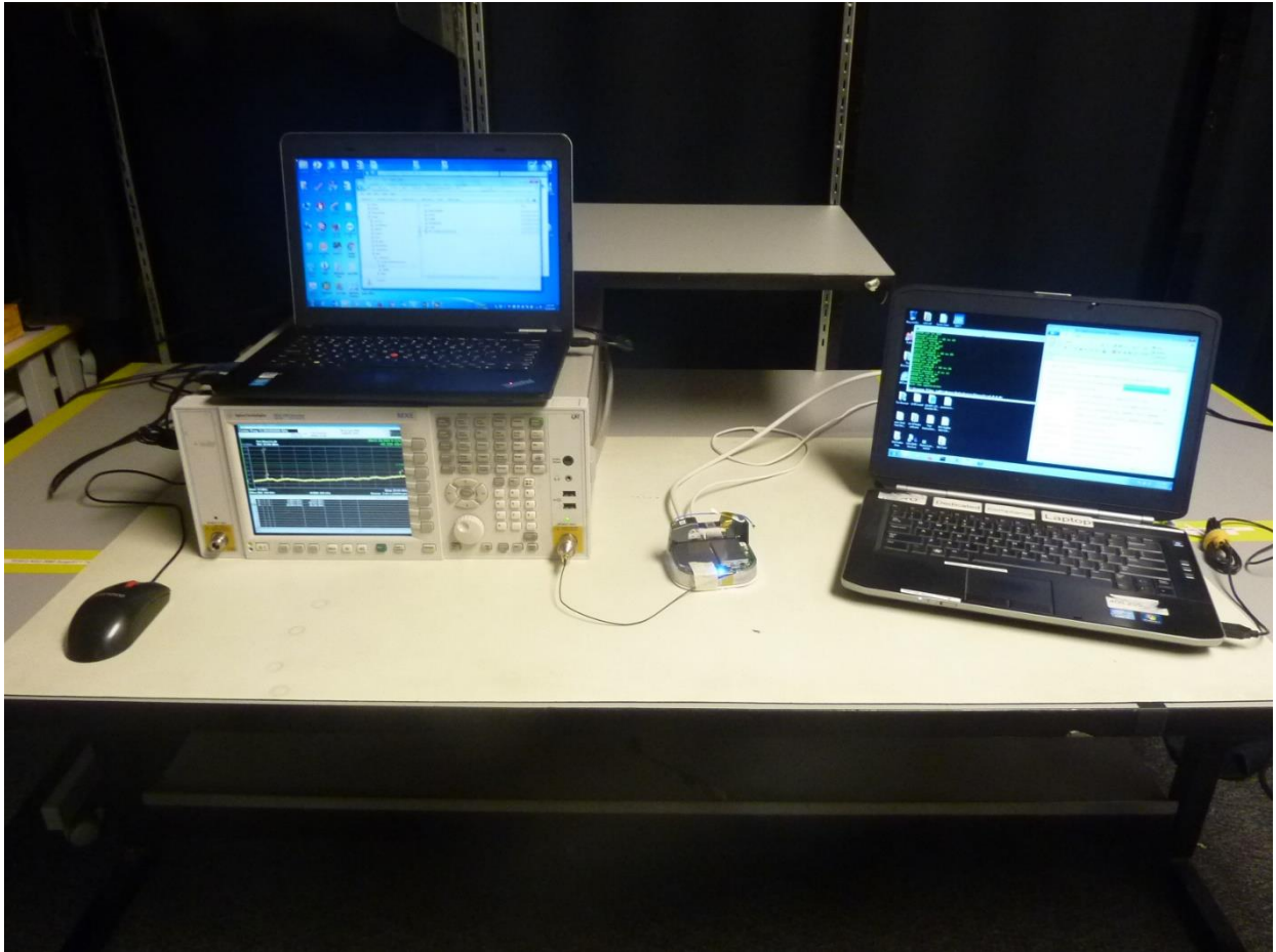
Figure 9: RF Conducted Test Setup (BLE/Zigbee)
