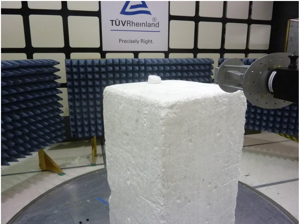
Figure 8: Test Setup for 18 GHz to 26GHz or 40 GHz (View 2)
