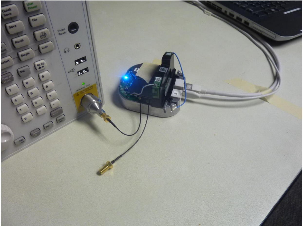
Figure 12: RF Conducted Test Setup – Closeup (WiFi)
