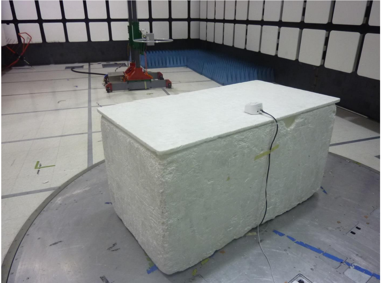
Figure 1: Test Setup for 9 kHz to 30 MHz (View 1)
