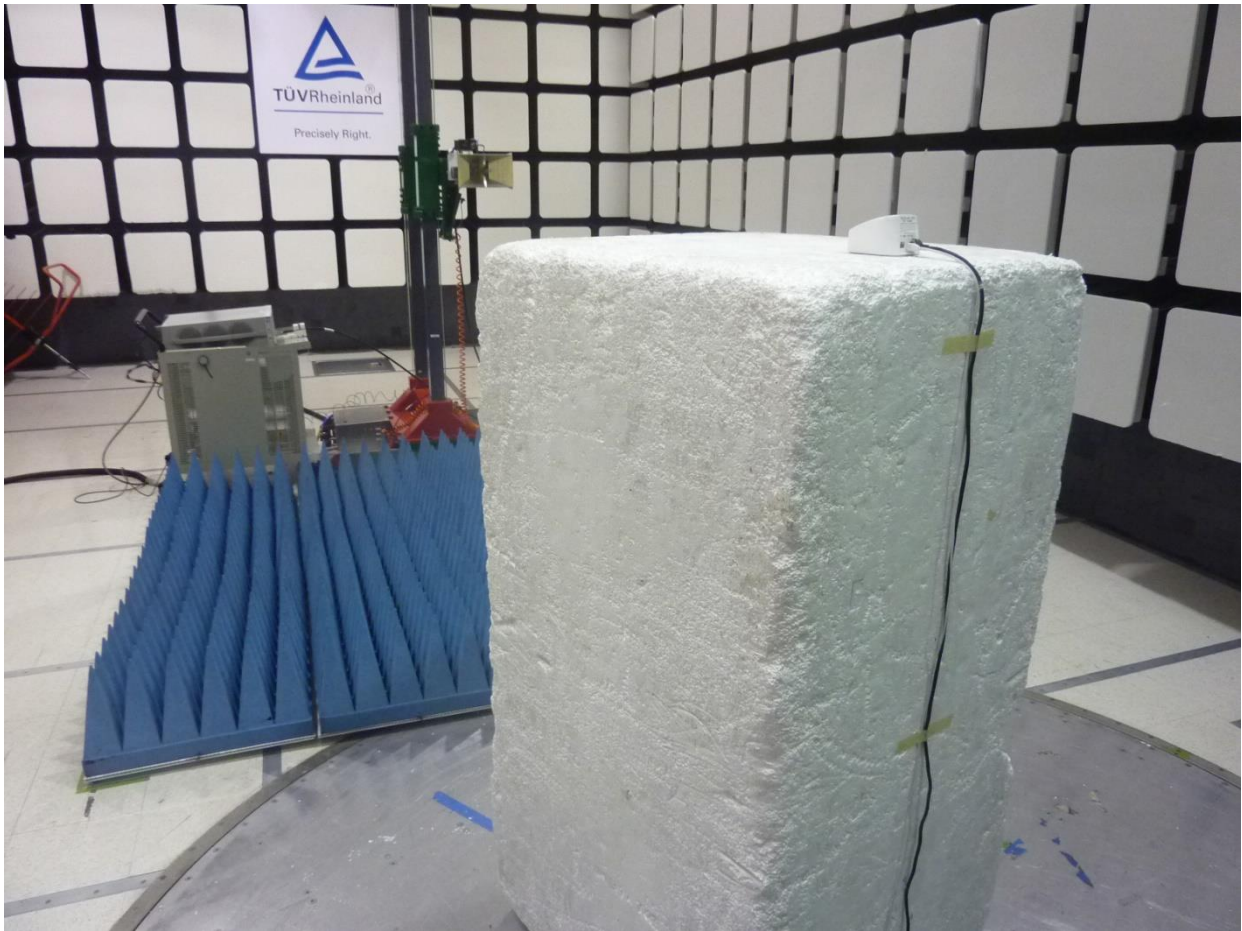
Figure 5: Test Setup for 1 GHz to 18 GHz (View 1)
