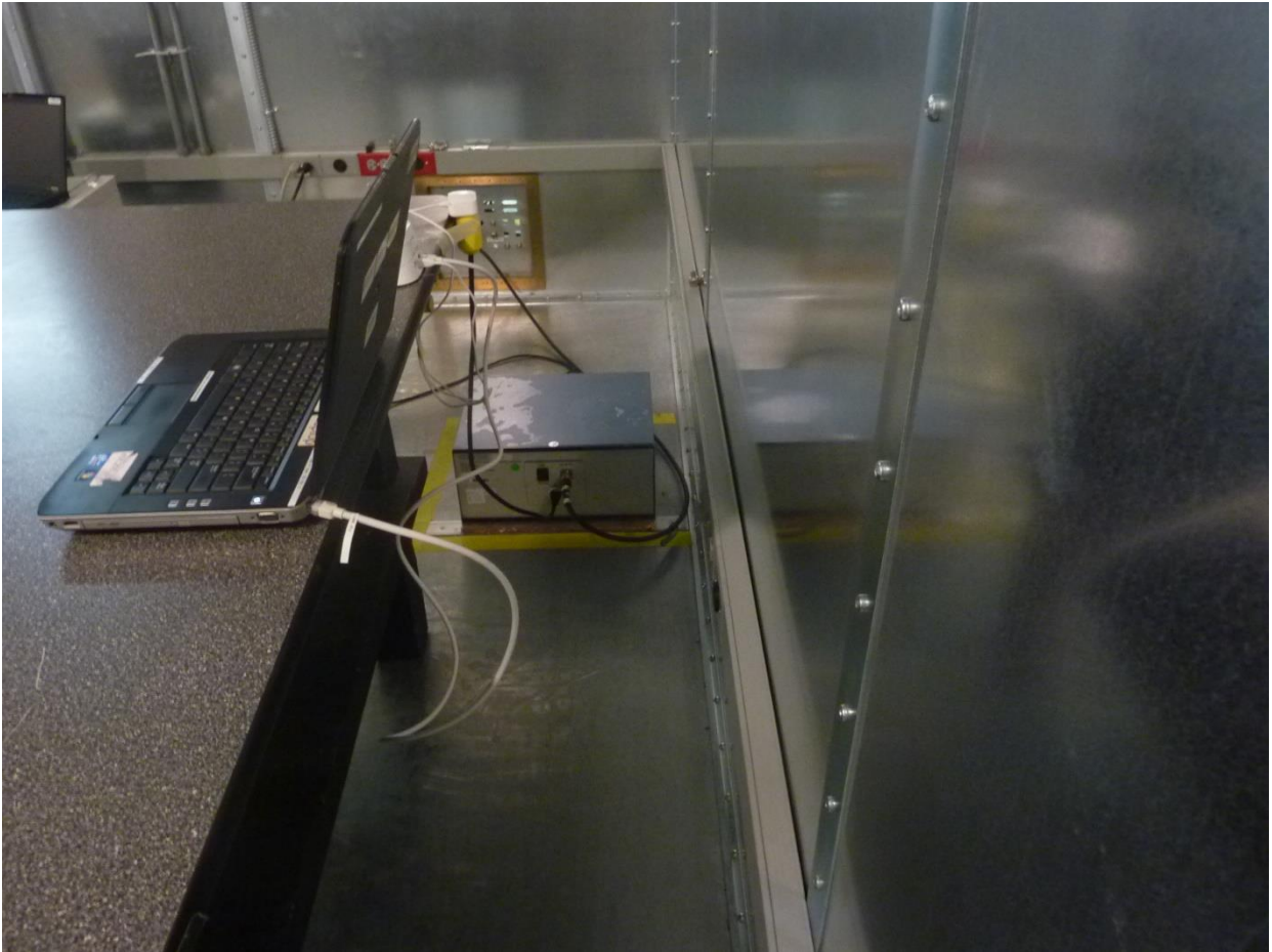
Figure 14: Conducted Emission Test Setup (Side)
