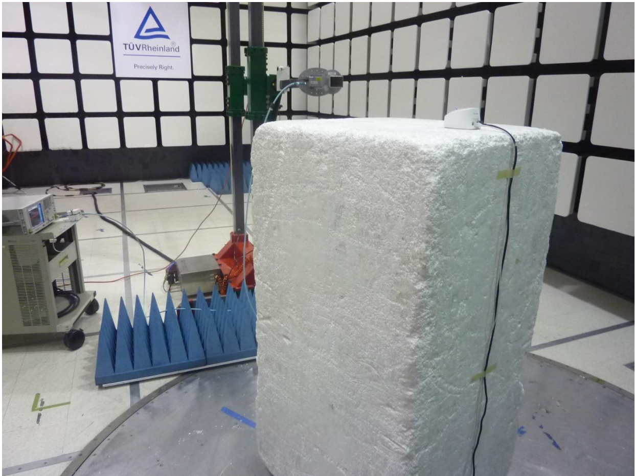
Figure 7: Test Setup for 18 GHz to 26GHz or 40 GHz (View 1)
