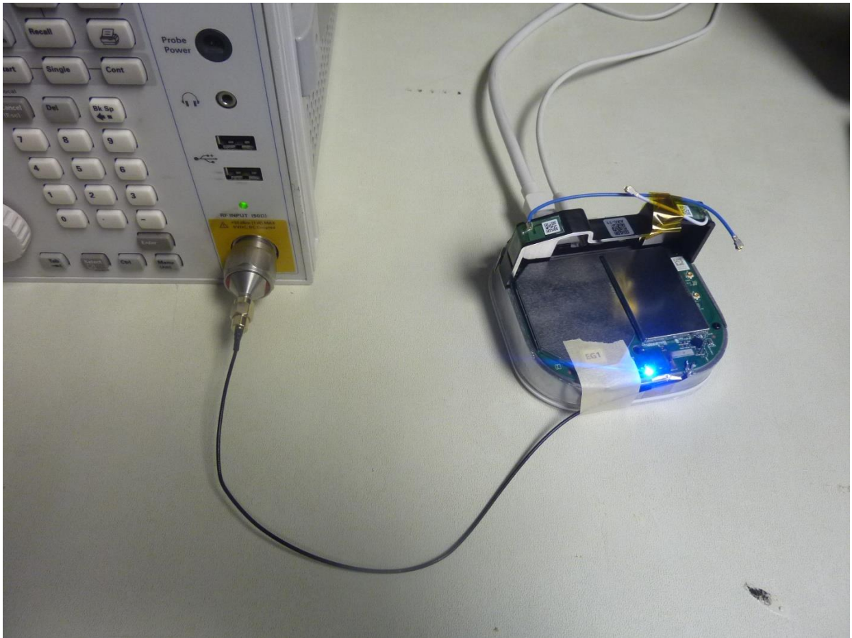
Figure 10: RF Conducted Test Setup – Closeup (BLE/Zigbee)
