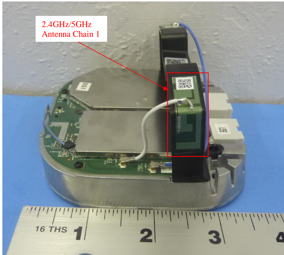
Figure 2: Photo of EUT
