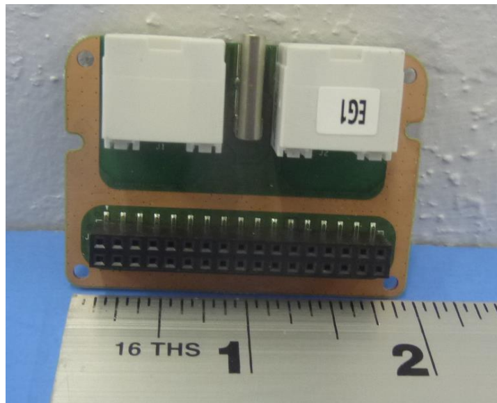
Figure 5: Photo of PCB (located at bottom of chassis – Interface side)
