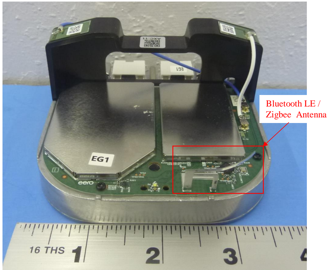
Figure 3: Photo of EUT
