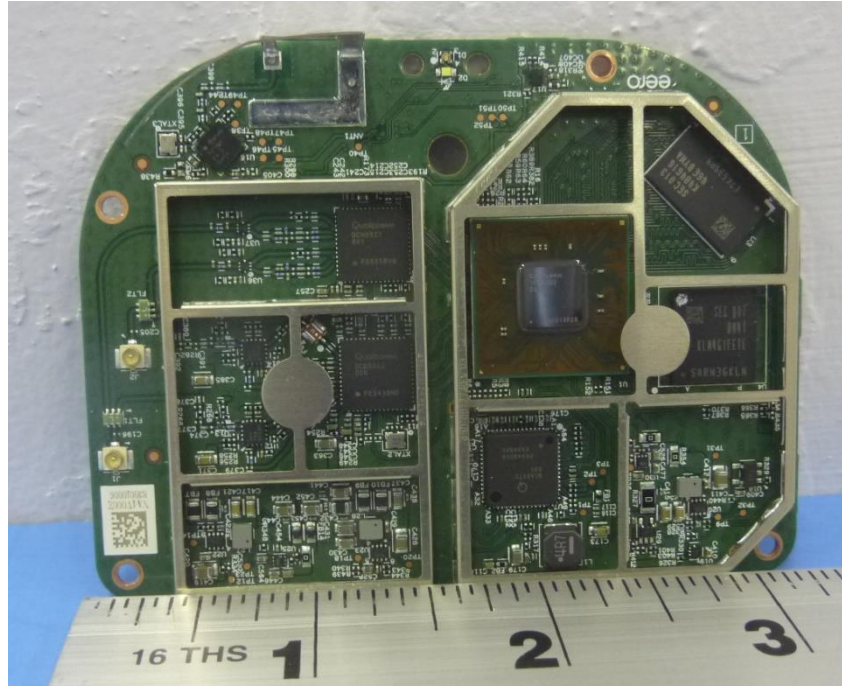
Figure 7: Photo of PCB (located at top of chassis – top side of PCB, shield cover removed)
