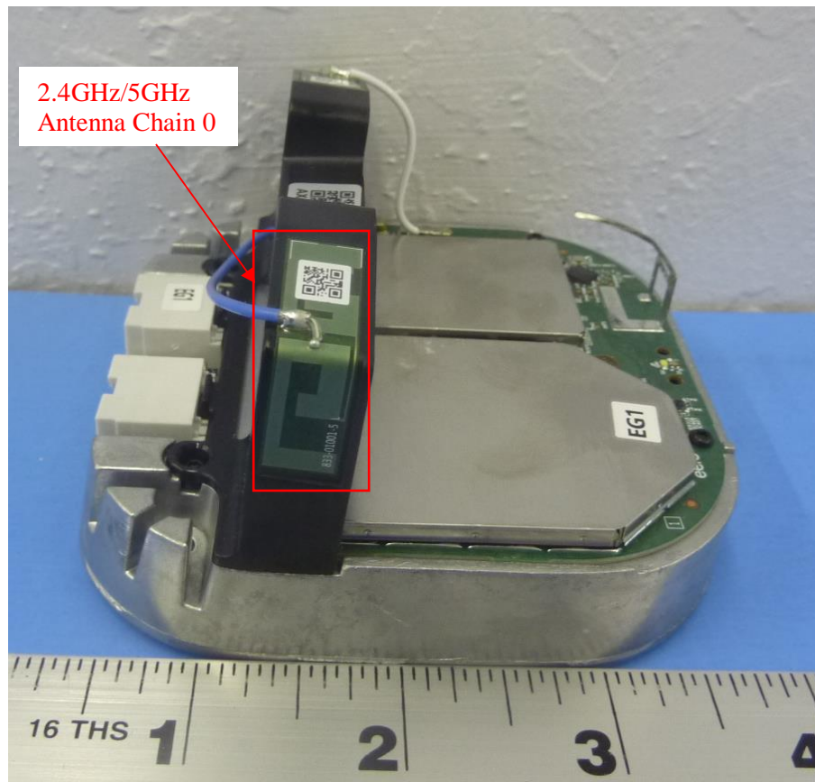
Figure 1: Photo of EUT
