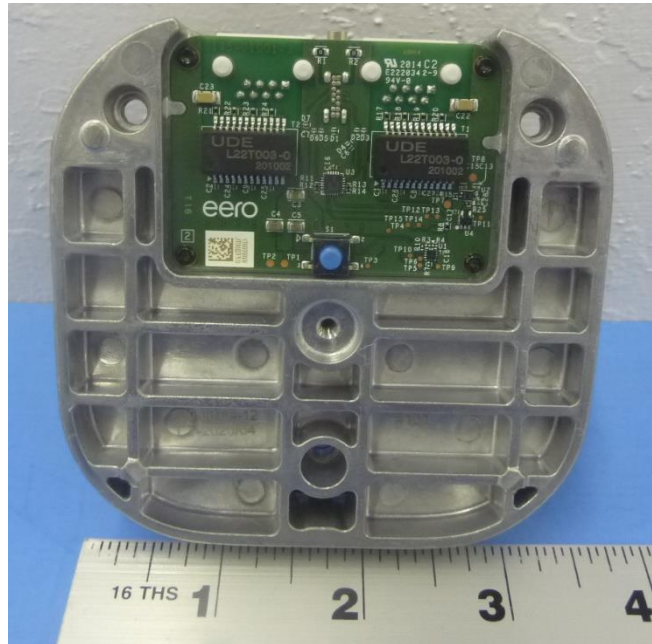
Figure 4: Photo of PCB (located at bottom of chassis – Component side)
