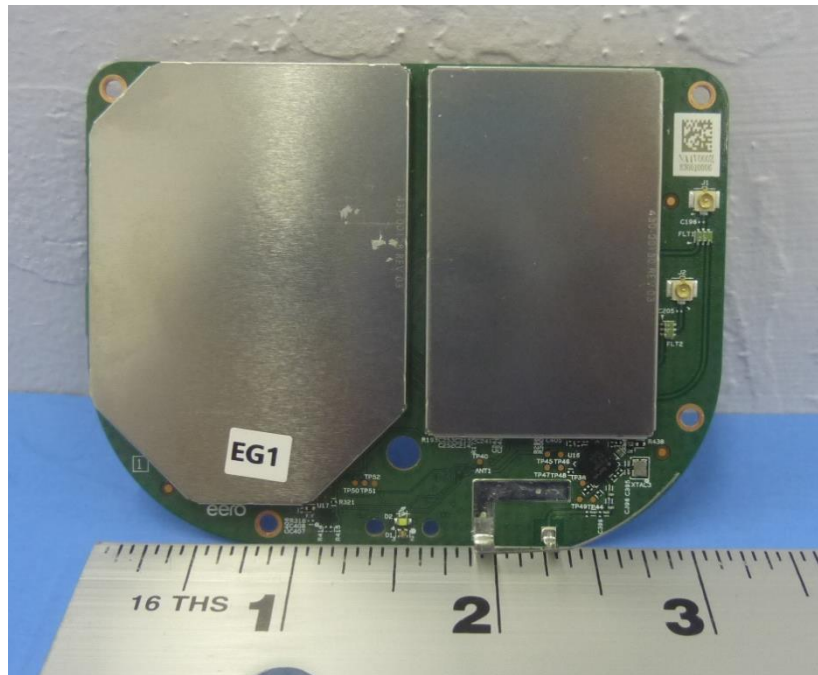
Figure 6: Photo of PCB (located at top of chassis – top side of PCB)
