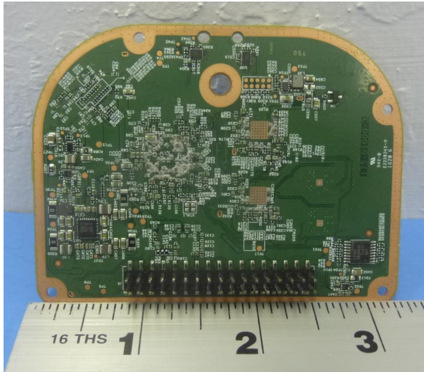
Figure 8: Photo of PCB (located at top of chassis – bottom side of PCB)
