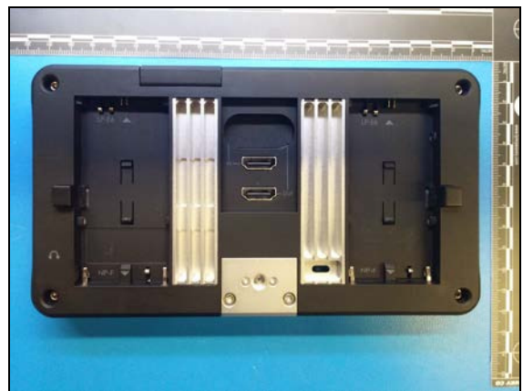
Figure 4: Model M701 - Rear
