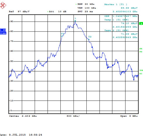
Figure 7.3.2-4: 99% Bandwidth Low Channel
