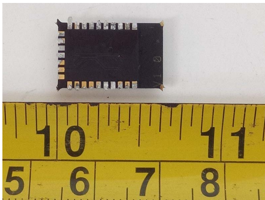
EUT–Rear View
