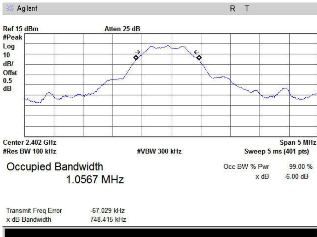
Channel 00 (2402MHz)
