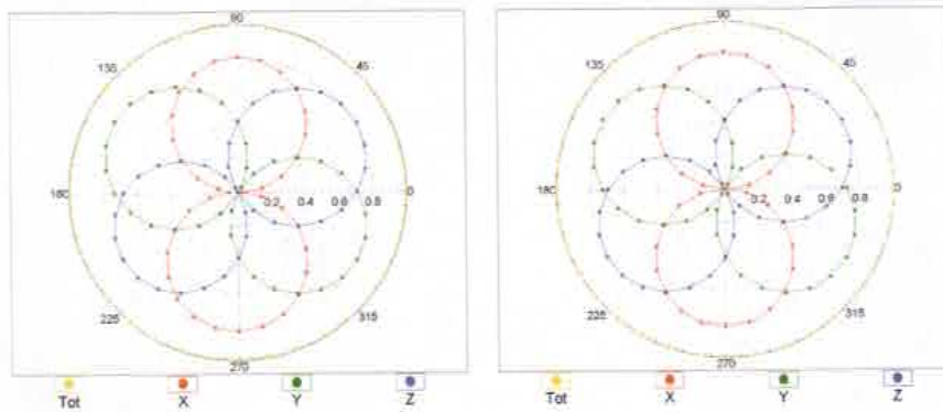
f=600 MHz,TEM
