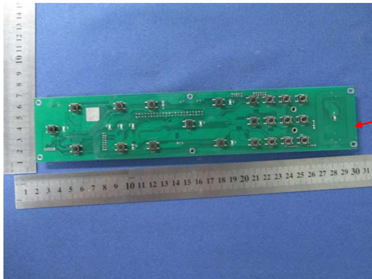
13.56MHz antenna
