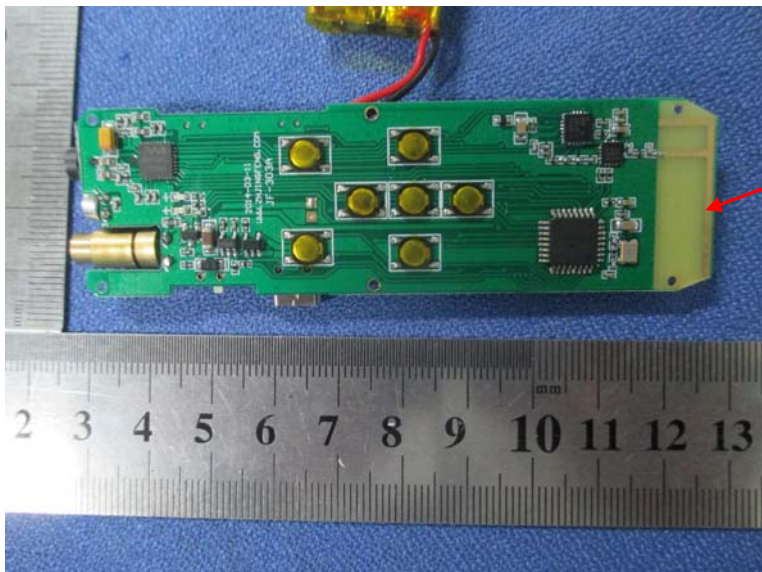
2.4G Transmitter Antenna
