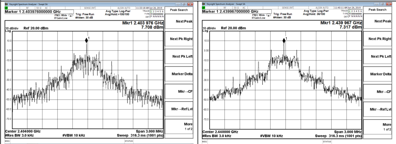
Channel 1 / 2404 MHz
