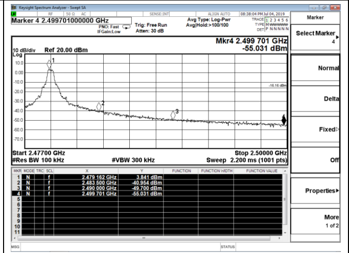
Channel 77 / 2480 MHz
