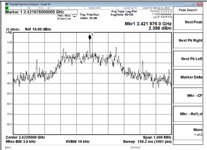
Channel 37 / 2422 MHz
