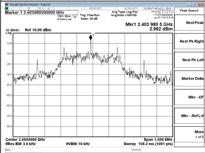
Channel 1 / 2404 MHz
