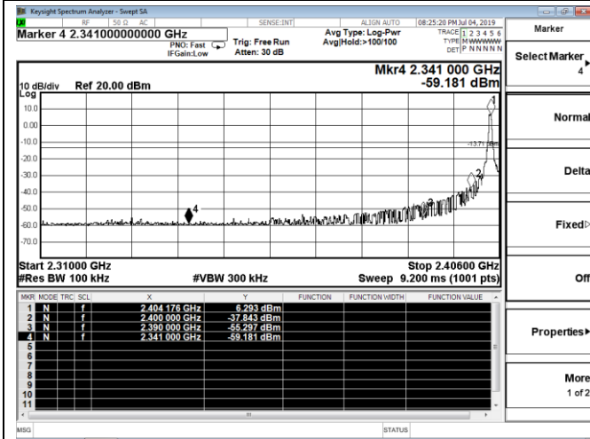
Channel 1 / 2404 MHz
