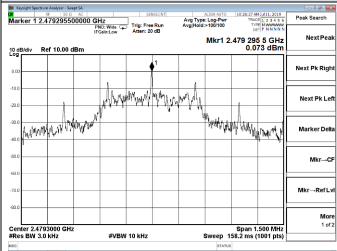
Channel 77 / 2479 MHz
