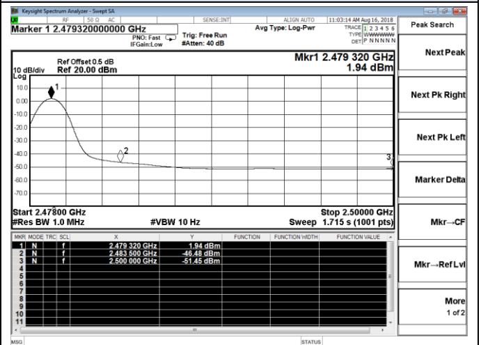
High Channel / 2479MHz - Average
