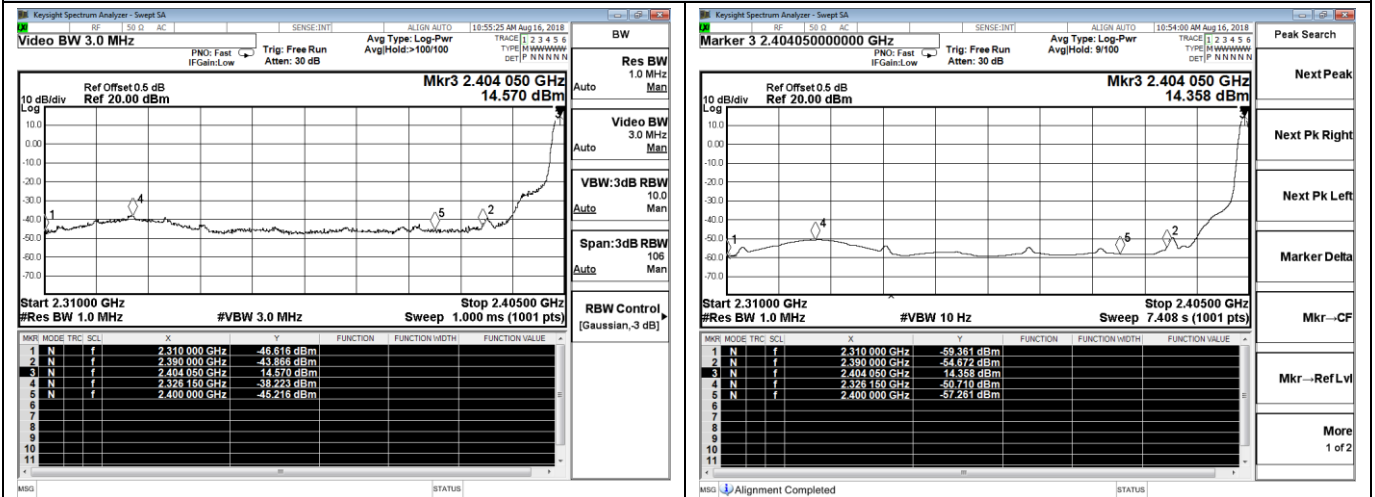
Low Channel / 2404MHz - Peak
