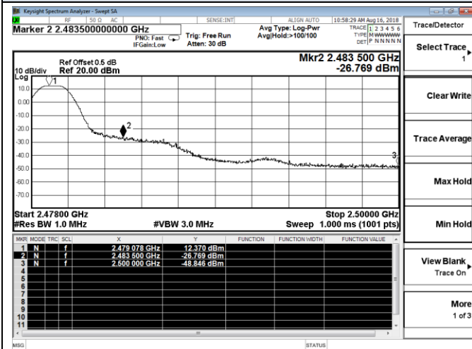
High Channel / 2479MHz - Peak
