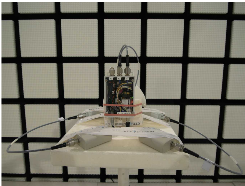
Photo 32: EUT at the anechoic chamber, SPA_5600_40_14_0_V_2 antennas with filters test setup
