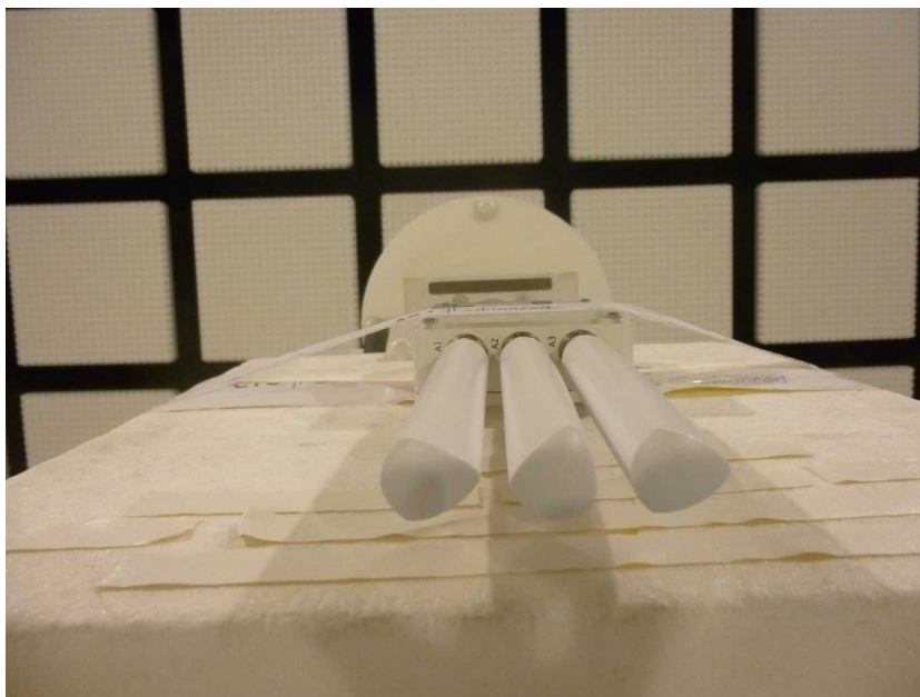
Photo 4: EUT at the anechoic chamber, F51-N antennas test setup
