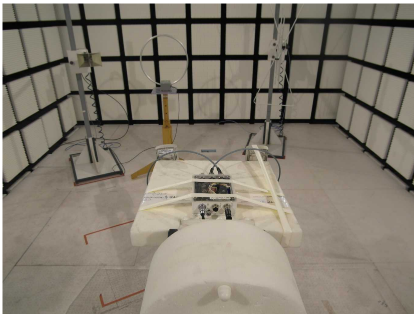
Photo 22: EUT at the anechoic chamber, SPA_5600_40_14_0_V_2 antennas test setup
