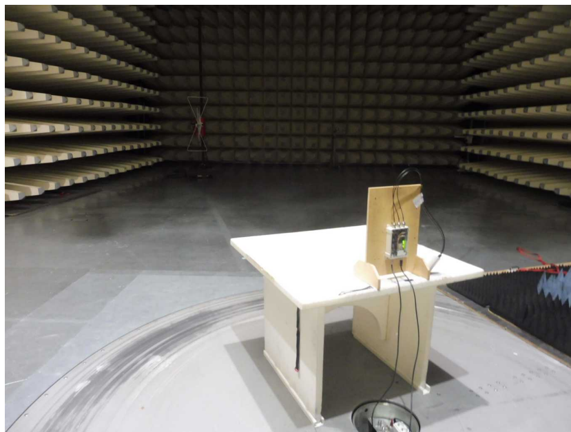
Photo 14: EUT at the semi-anechoic chamber, SPA_5600_65_9_0_MIMO antennas test setup
