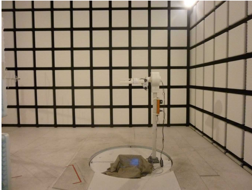
Photo 5: EUT at the anechoic chamber, F51-N antennas test setup
