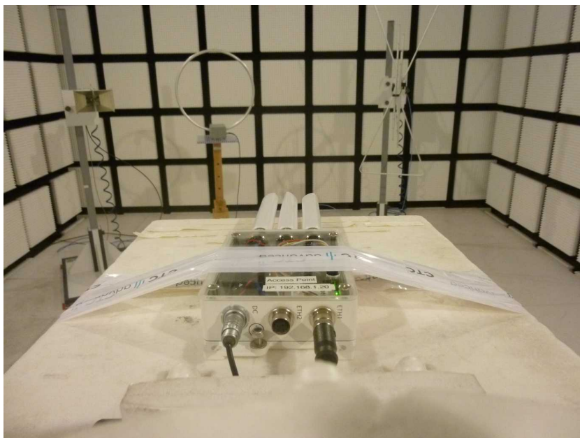
Photo 6: EUT at the anechoic chamber, F51-N antennas test setup
