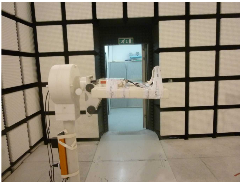
Photo 12: EUT at the anechoic chamber, SPA_5600_65_9_0_MIMO antennas test setup
