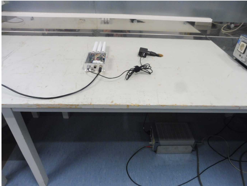
Photo 37: AC conducted emission test setup
