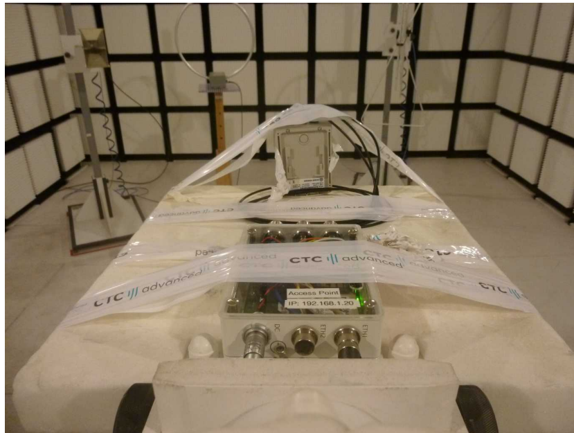
Photo 13: EUT at the anechoic chamber, SPA_5600_65_9_0_MIMO antennas test setup
