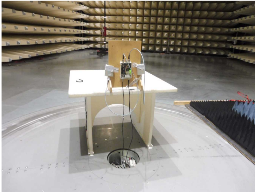
Photo 29: EUT at the semi-anechoic chamber, SPA_5600_40_14_0_V_2 antennas test setup
