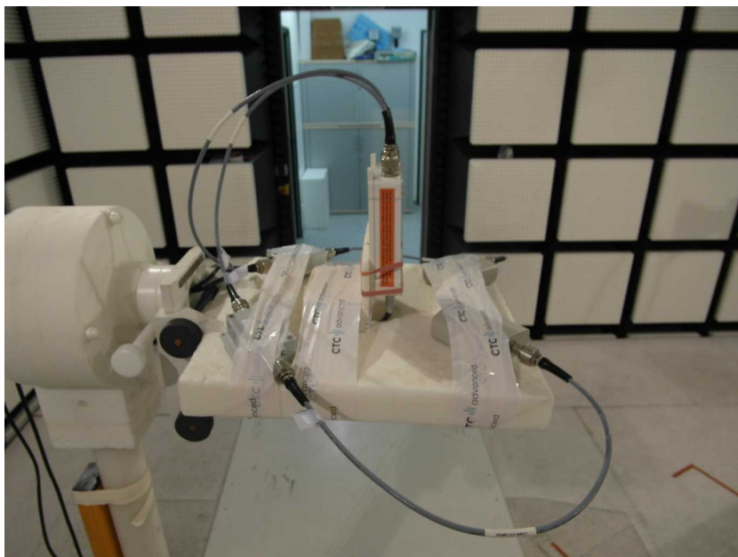
Photo 30: EUT at the anechoic chamber, SPA_5600_40_14_0_V_2 antennas with filters test setup
