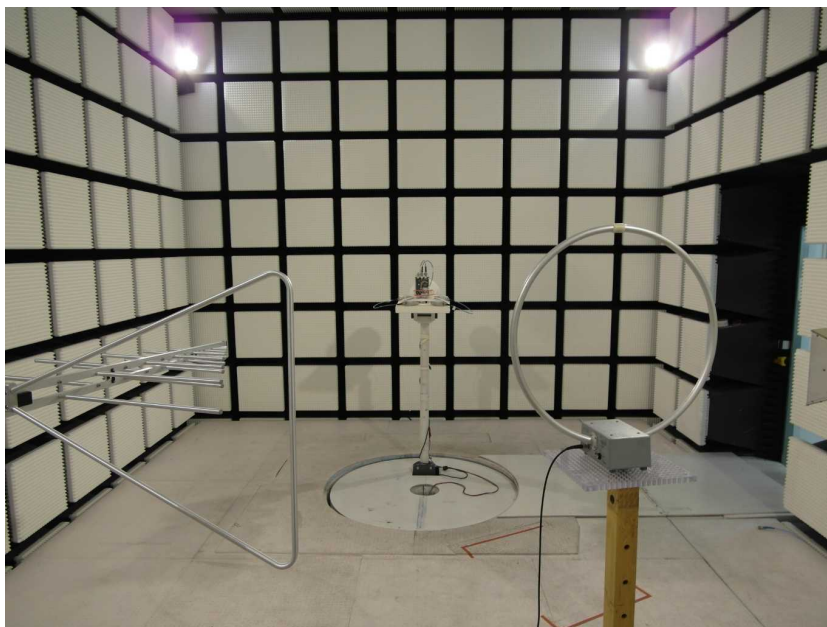
Photo 34: EUT at the anechoic chamber, SPA_5600_40_14_0_V_2 antennas with filters test setup
