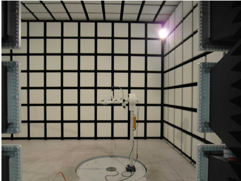
Photo 33: EUT at the anechoic chamber, SPA_5600_40_14_0_V_2 antennas with filters test setup
