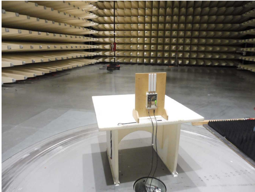
Photo 7: EUT at the semi-anechoic chamber, F51-N antennas test setup
