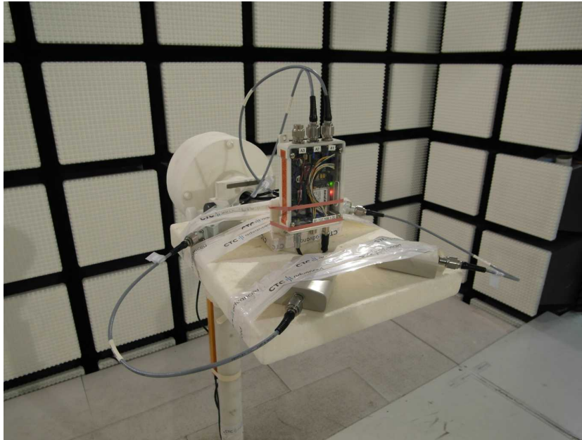
Photo 31: EUT at the anechoic chamber, SPA_5600_40_14_0_V_2 antennas with filters test setup
