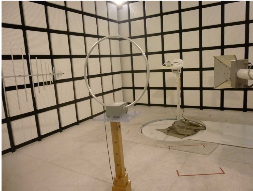
Photo 11: EUT at the anechoic chamber, SPA_5600_65_9_0_MIMO antennas test setup
