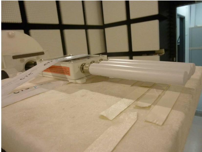
Photo 1: EUT at the anechoic chamber, F51-N antennas test setup
