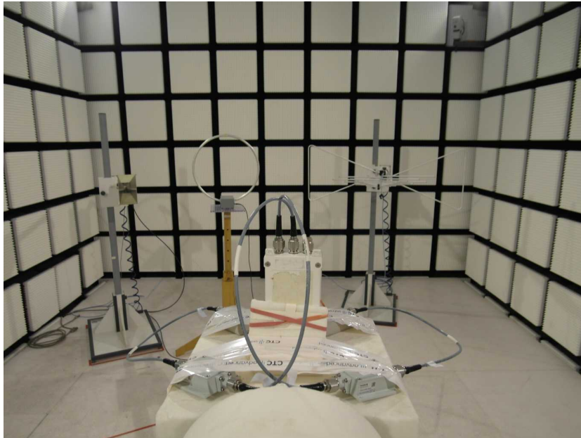
Photo 35: EUT at the anechoic chamber, SPA_5600_40_14_0_V_2 antennas with filters test setup
