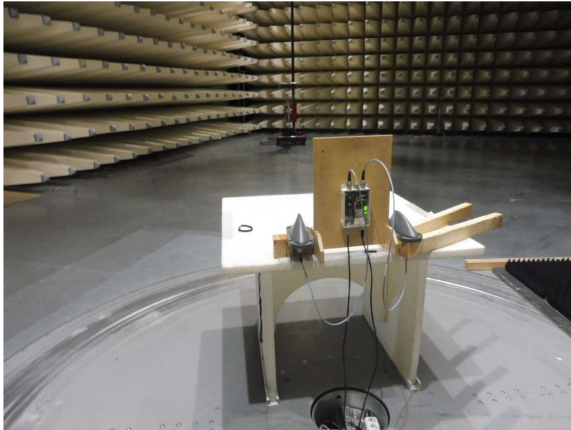
Photo 21: EUT at the semi-anechoic chamber, SPA_5600_45_12_10_V antennas test setup
