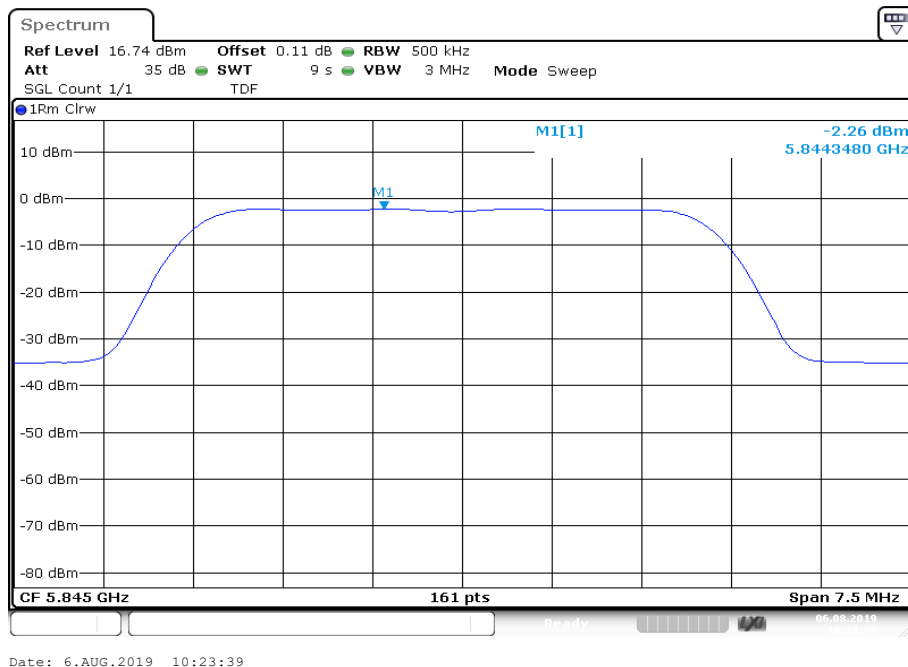
Plot 18: U-NII-3; highest channel
