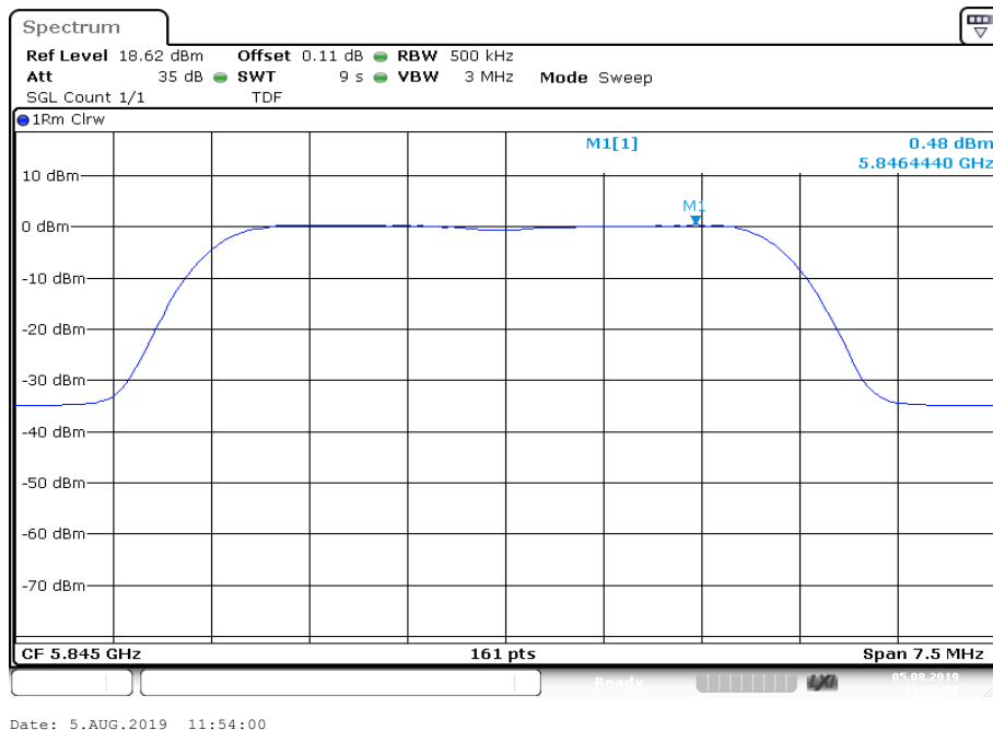
Plot 15: U-NII-3; highest channel
