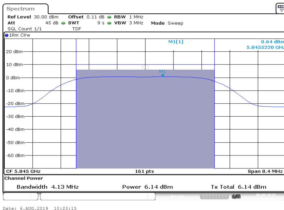
Plot 9: U-NII-3; highest channel
