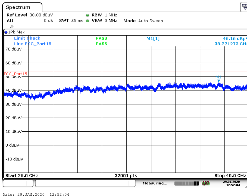
Plot 4: 26 GHz to 40 GHz; vertical & horizontal polarization; U-NII-3; lowest channel
