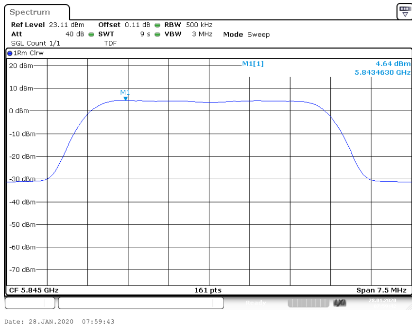
Plot 9: U-NII-3; highest channel
