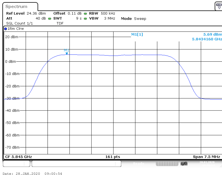
Plot 12: U-NII-3; highest channel
