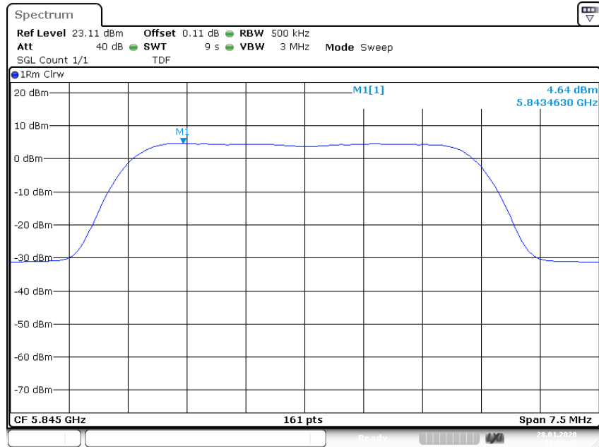
Plot 9: U-NII-3; highest channel
