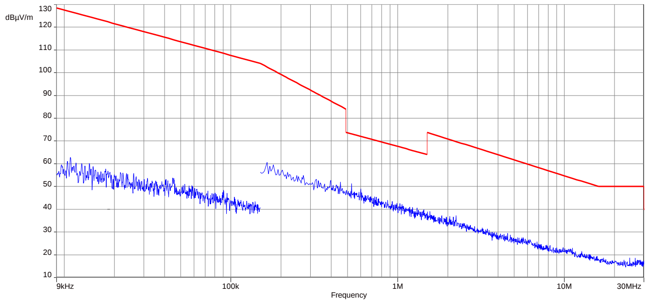
Plot 1: 9 kHz to 30 MHz, U-NII-3; lowest channel
