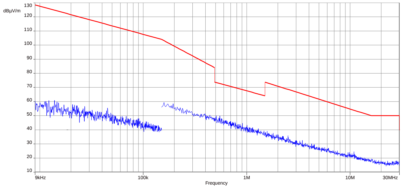
Plot 3: 9 kHz to 30 MHz, U-NII-3; highest channel
