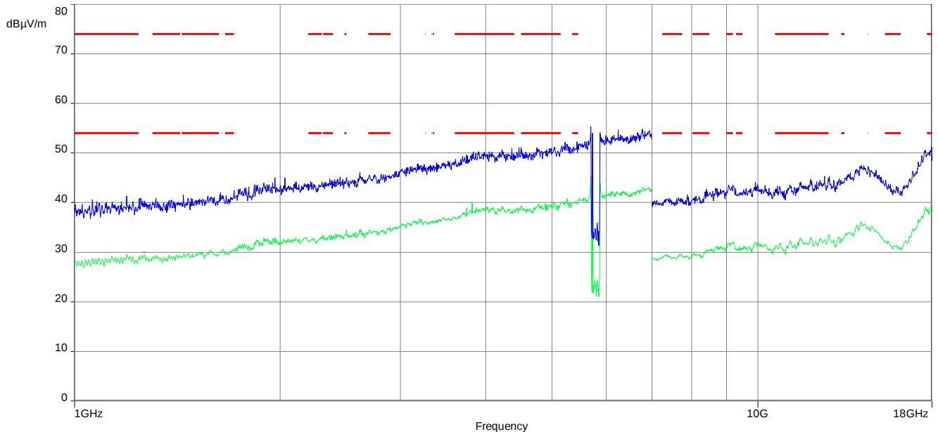
Plot 2: 1 GHz to 18 GHz; vertical & horizontal polarization; U-NII-3; lowest channel
