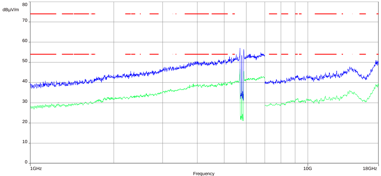
Plot 6: 1 GHz to 18 GHz; vertical & horizontal polarization; U-NII-3; middle channel
