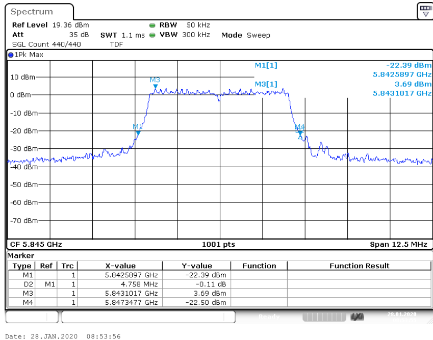
Plot 6: U-NII-3; highest channel
