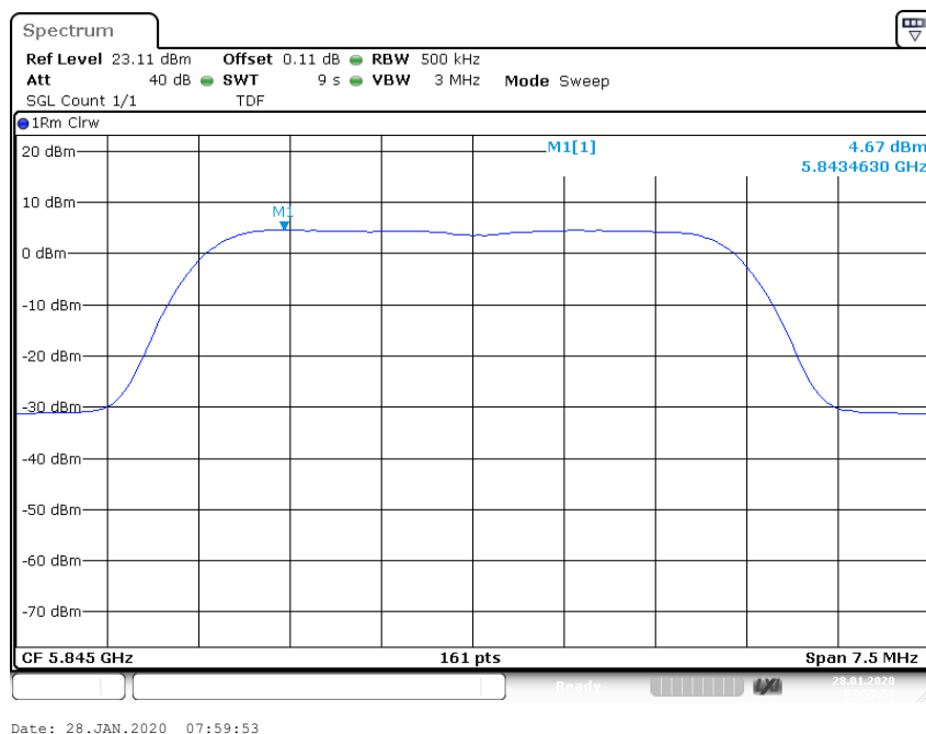
Plot 3: U-NII-3; highest channel
