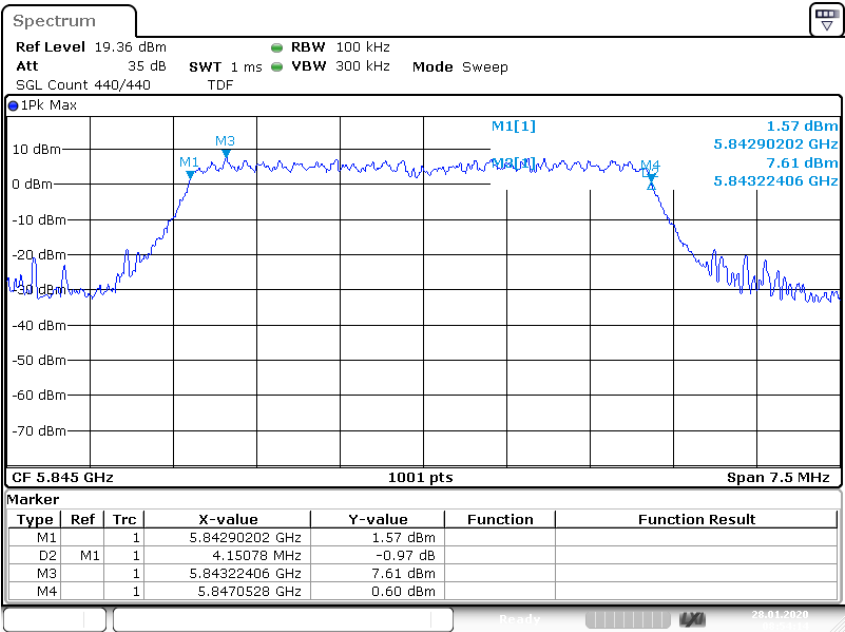
Plot 6: U-NII-3; highest channel
