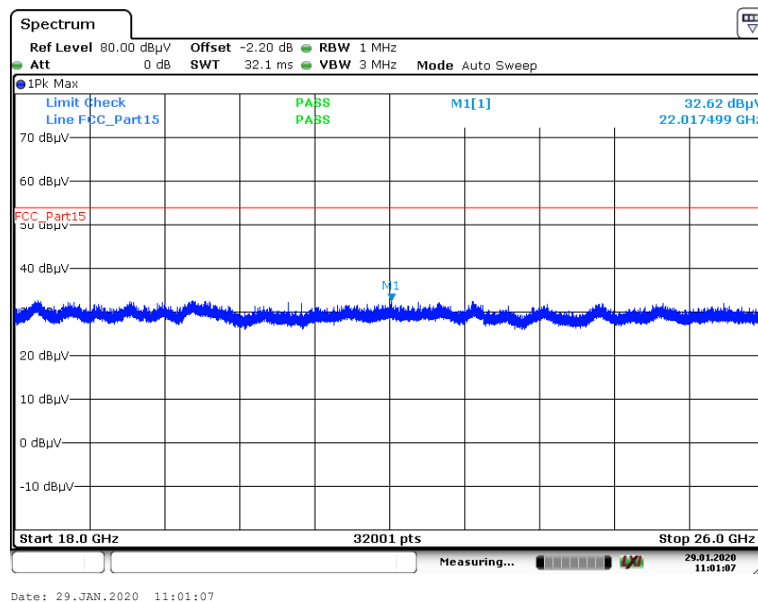
Plot 3: 18 GHz to 26 GHz; vertical & horizontal polarization; U-NII-3; lowest channel
