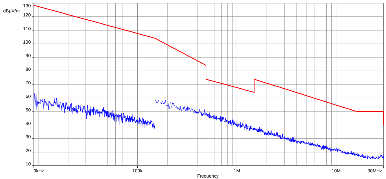
Plot 2: 9 kHz to 30 MHz, U-NII-3; middle channel
