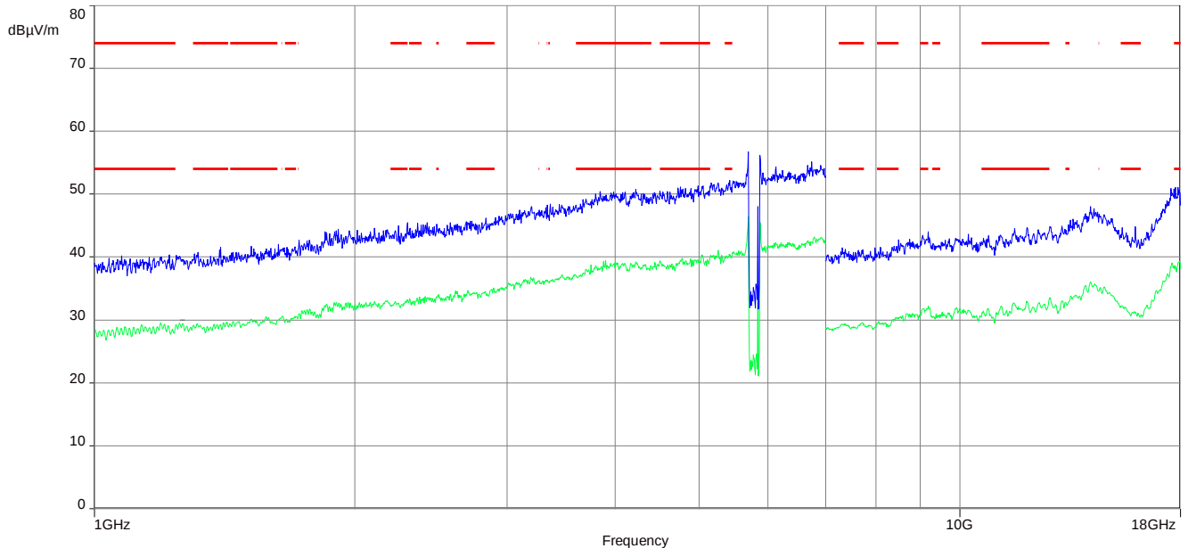
Plot 10: 1 GHz to 18 GHz; vertical & horizontal polarization; U-NII-3; highest channel
