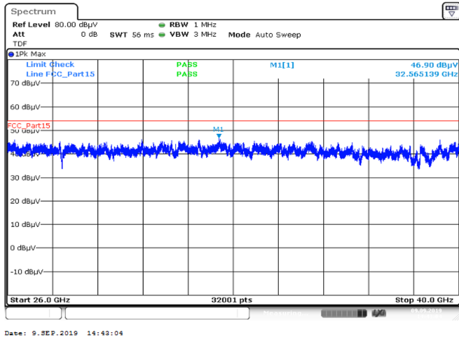
Plot 4: 26 GHz to 40 GHz; vertical & horizontal polarization; U-NII-3; lowest channel
