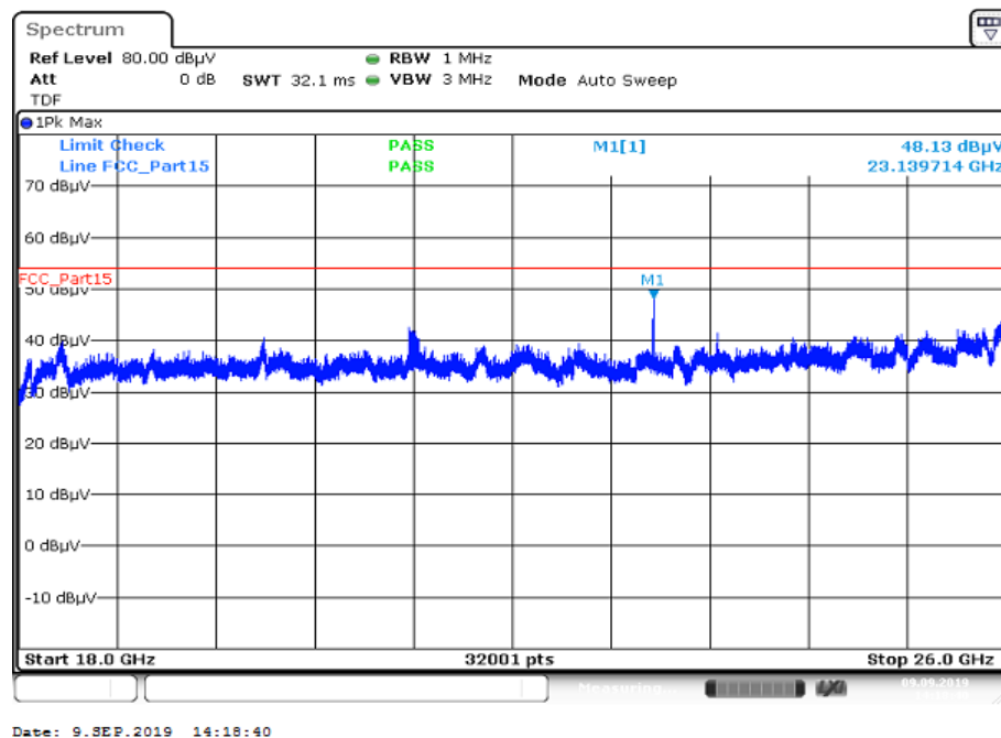
Plot 7: 18 GHz to 26 GHz; vertical & horizontal polarization; U-NII-3; middle channel
