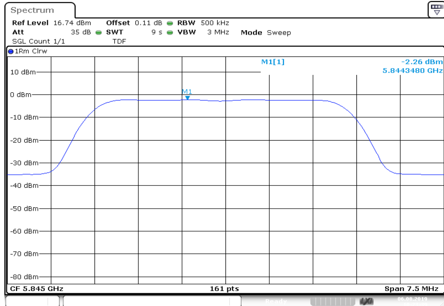
Plot 18: U-NII-3; highest channel
