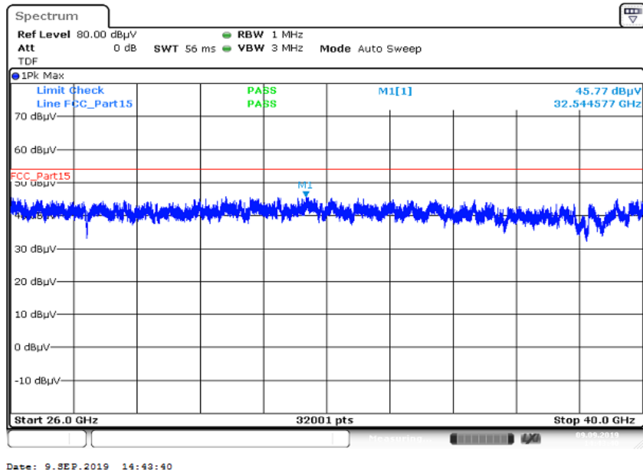
Plot 8: 26 GHz to 40 GHz; vertical & horizontal polarization; U-NII-3; middle channel
