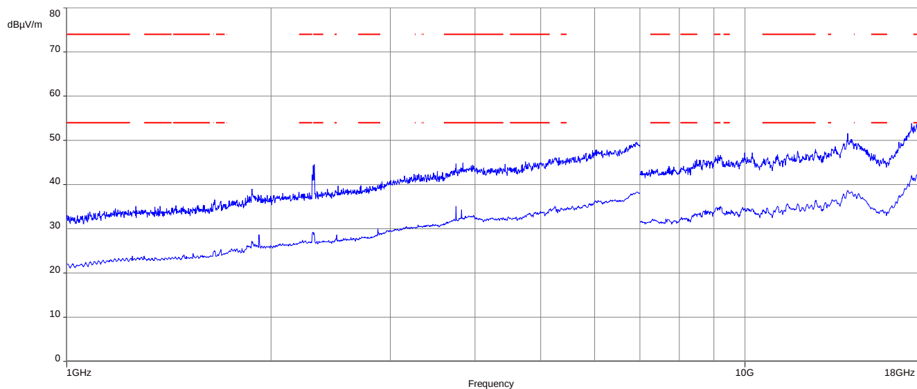
Plot 2: 1 GHz to 18 GHz, vertical & horizontal polarization
