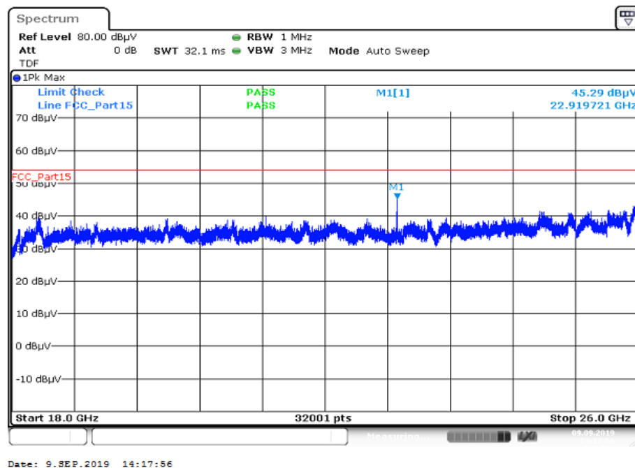
Plot 3: 18 GHz to 26 GHz; vertical & horizontal polarization; U-NII-3; lowest channel
