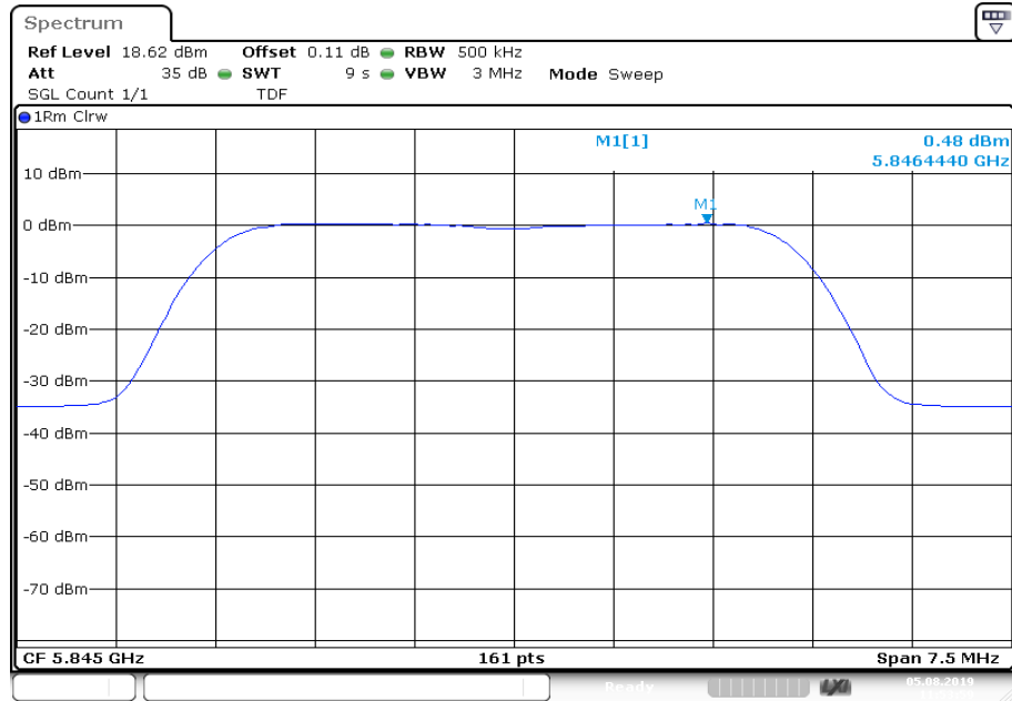
Plot 15: U-NII-3; highest channel
