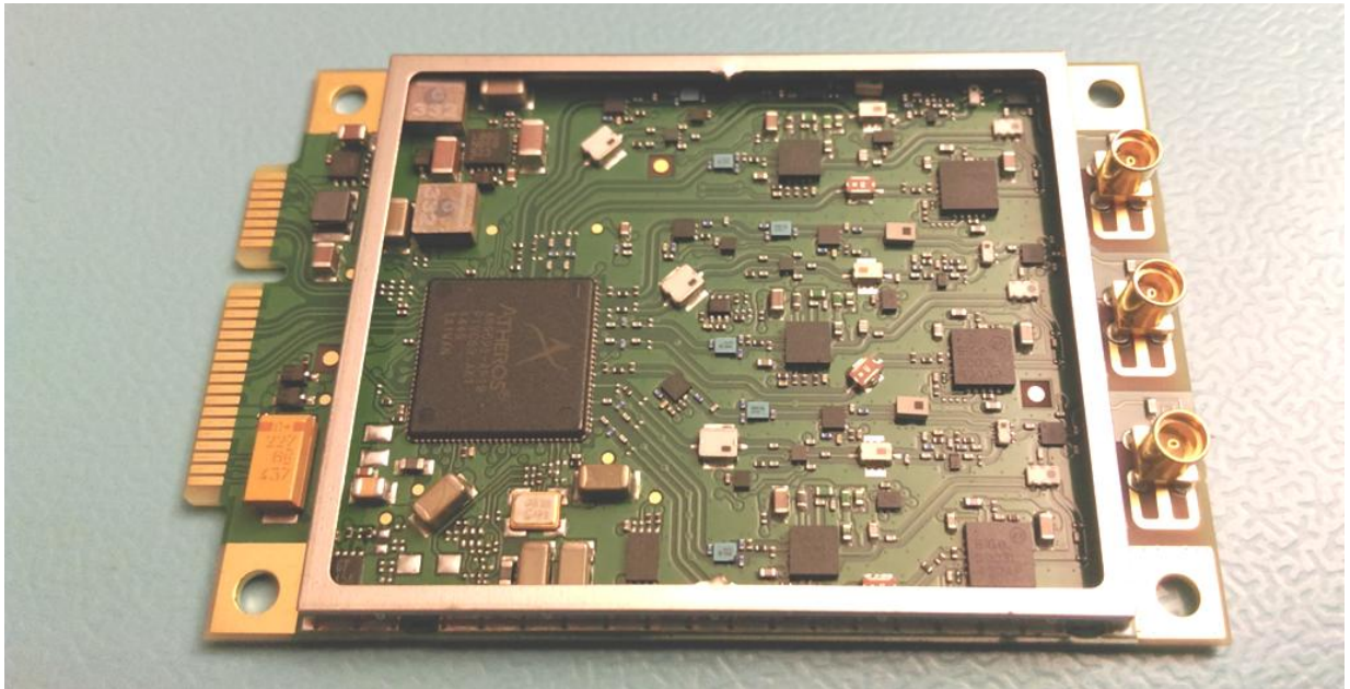
Figure 1: Internal Photo Top-Layer DT50RF
