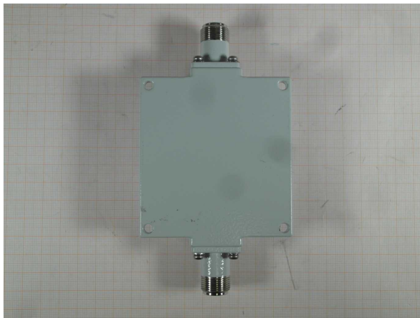
Photo 16: Neratec CAVITY 105072
