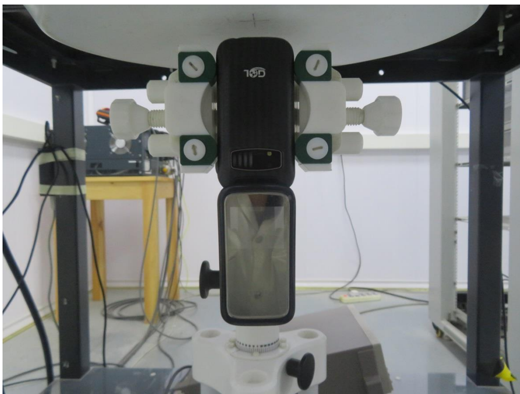
10mm body-worn Bottom Side Setup Photo
