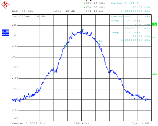
99% Occupancy bandwidth
