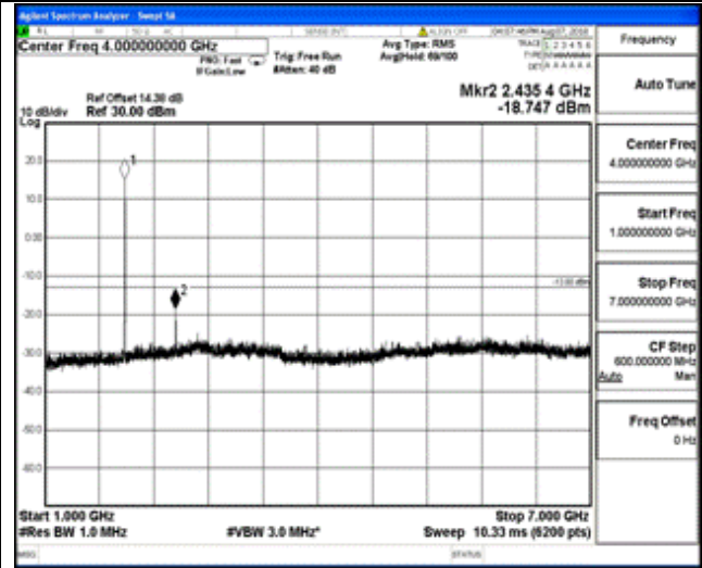
1 GHz – 7 GHz
