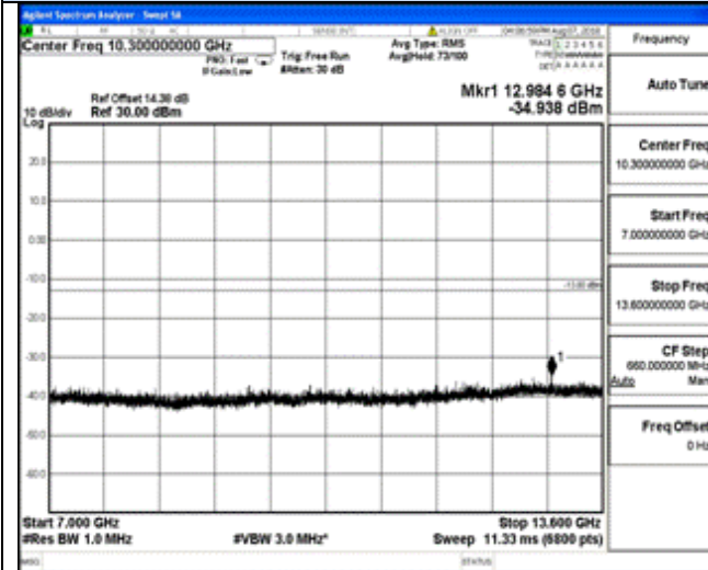
7 GHz – 13.6 GHz
