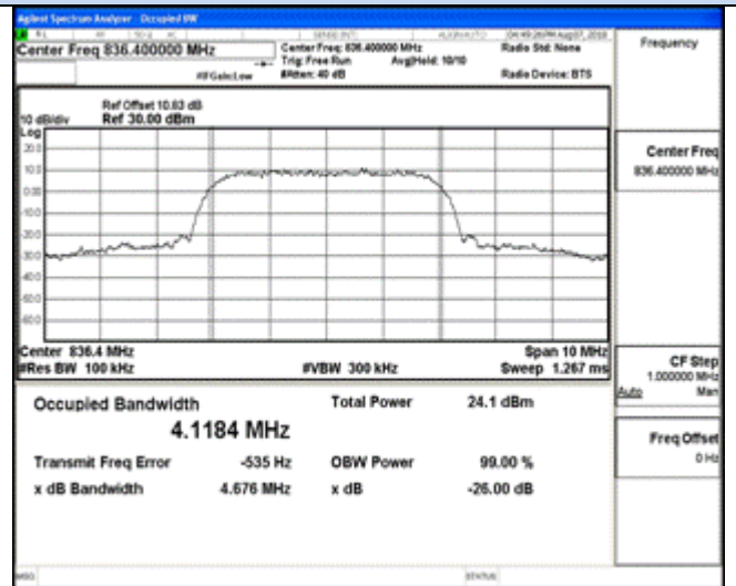
Channel 4182 / 836.4 MHz
