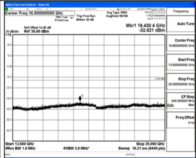
13.6 GHz – 20 GHz
