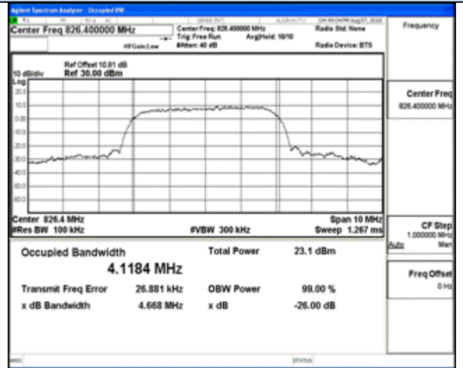
Channel 4132 / 826.4 MHz
