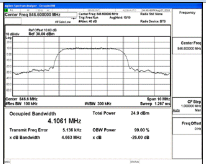
Channel 4233 / 846.6 MHz
