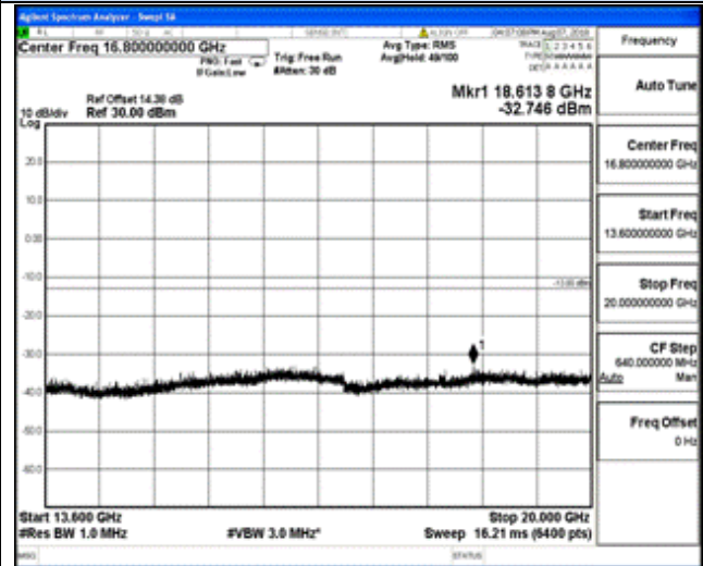
13.6 GHz – 20 GHz
