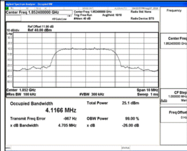
Channel 9262 / 1852.4 MHz
