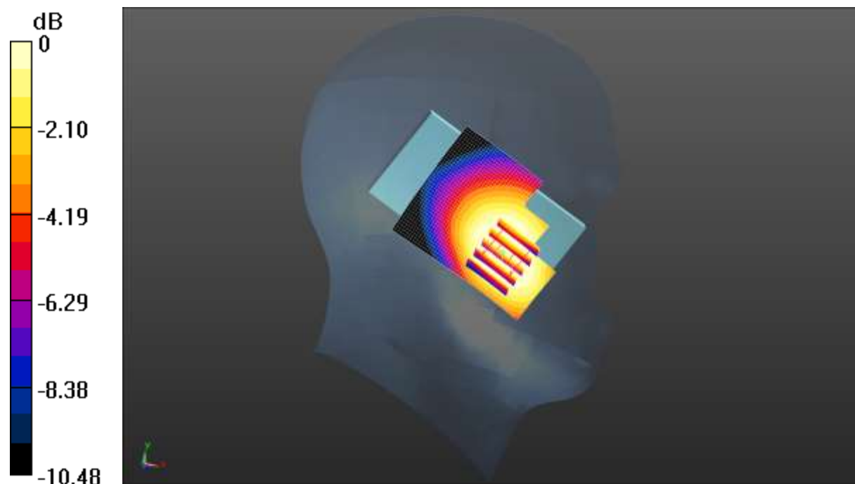
0 dB = 0.253 W/kg = -5.97 dBW/kg
