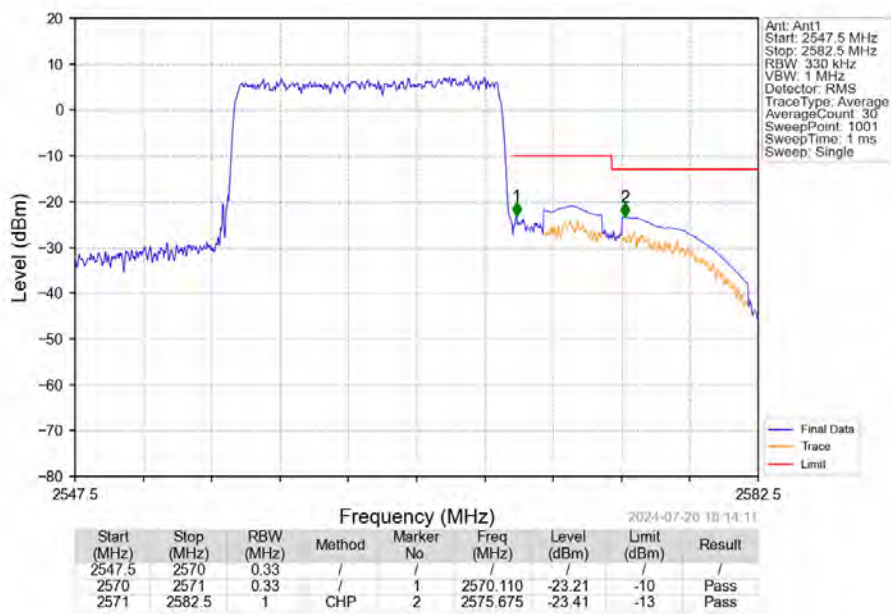
Band7 15MHz 16QAM HCH 2562.5MHz RB 75 0 NTNV
